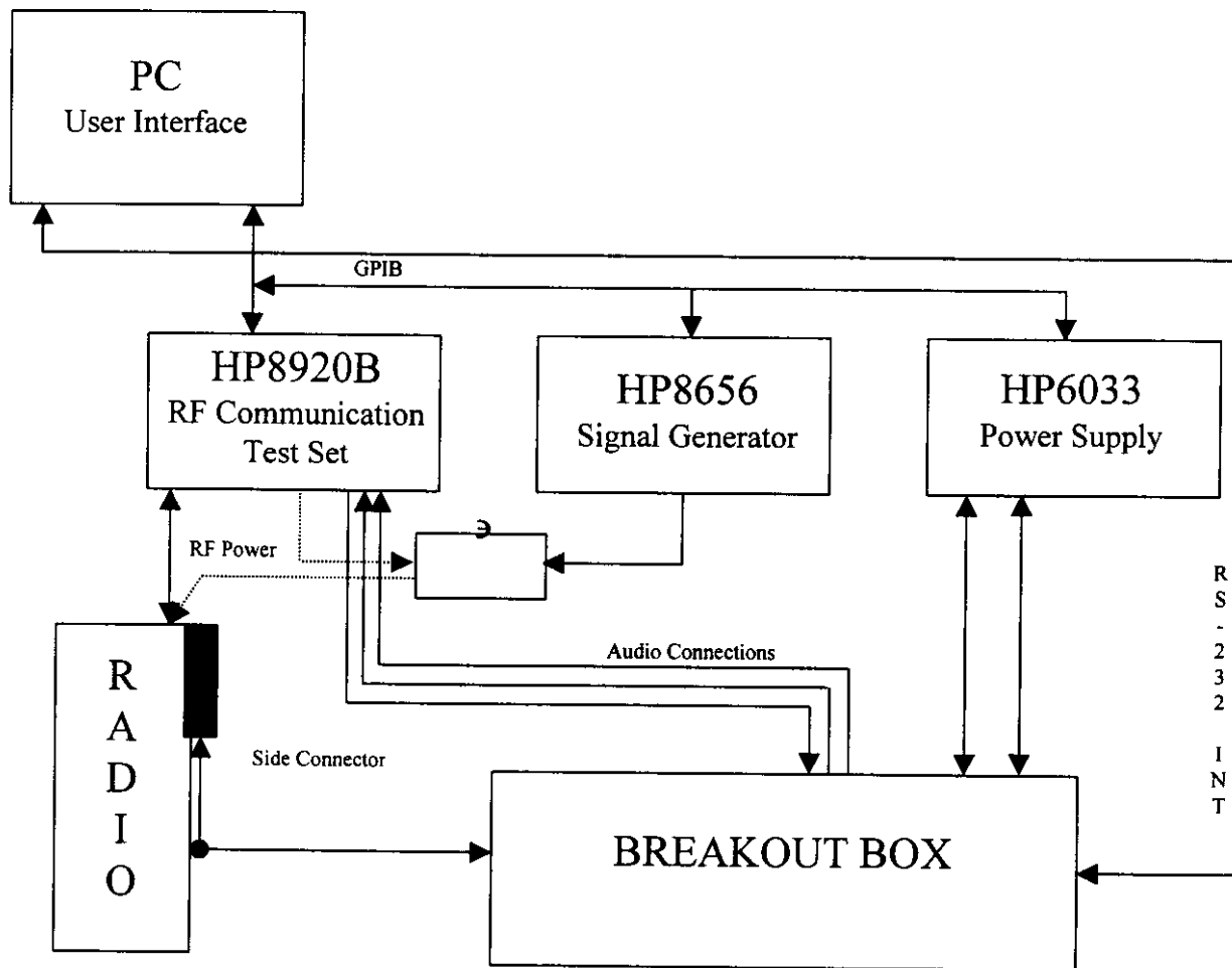
Figure 3-1. Test Configuration
