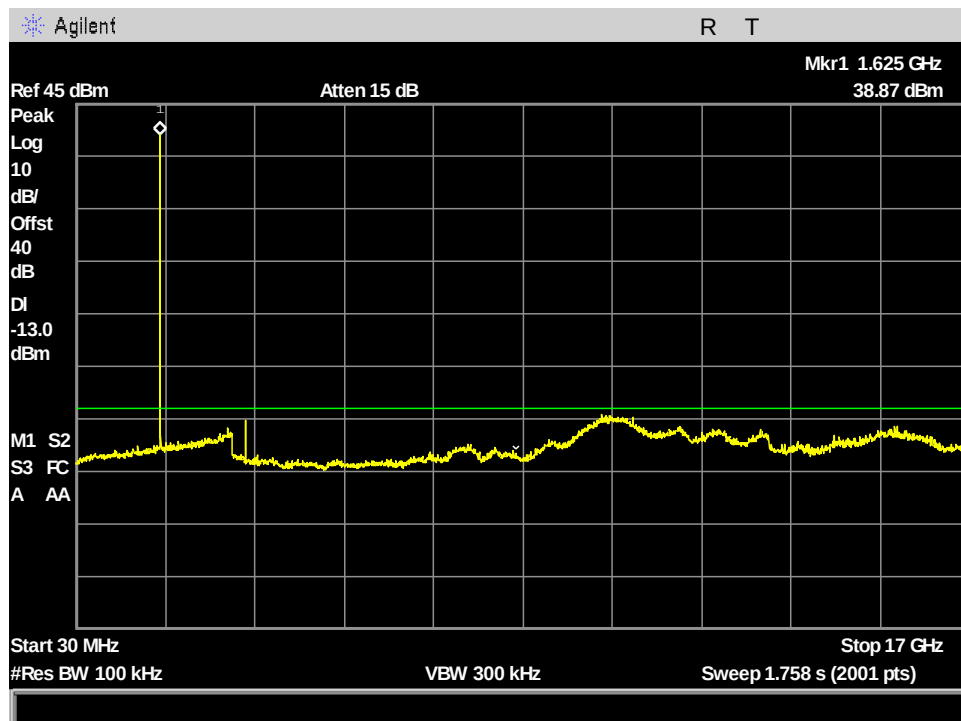
Figure 138: §25.202(f) VesseLINK Spurious Emissions at Antenna Terminals, ch232_666.666kHz_30MHz - 17GHz
