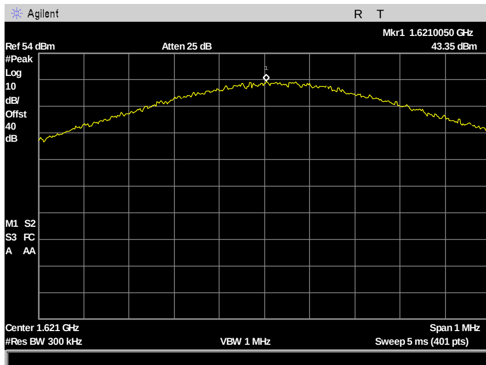
Figure 62: §25.204(a) Conducted RF Output Power, MissionLINK PK_Output Power_ch121_41.668kHz BW
