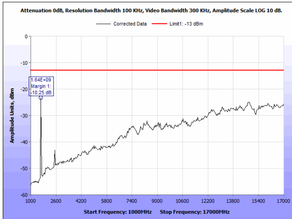
Figure 170: §25.202(f) Radiated Spurious Emissions, MissionLINK 200, Ch232_83.334kHz BW_1-17 GHz.
