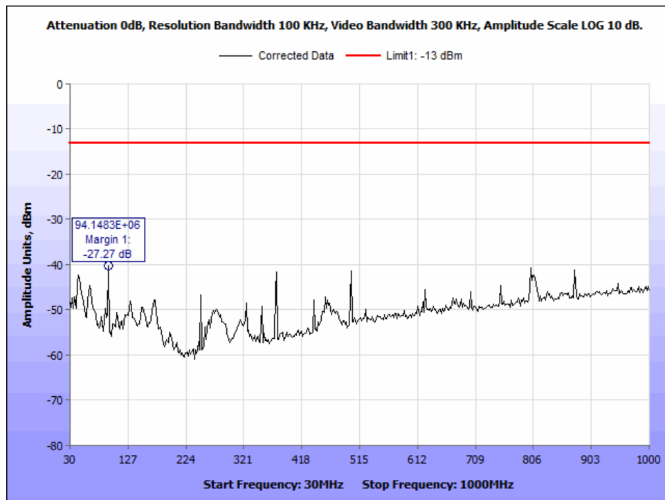
Figure 169: §25.202(f) Radiated Spurious Emissions, MissionLINK 200, Ch232_666.666kHz BW_30-1000MHz.
