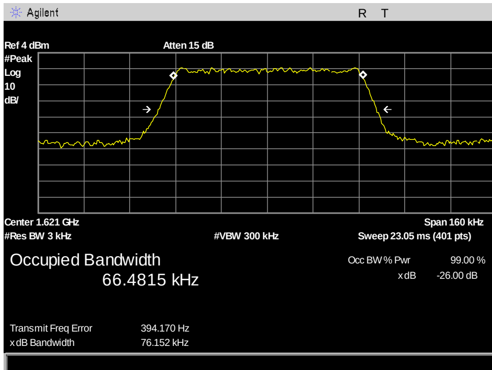
Figure 100: §2.1049(b) Occupied Bandwidth, Ch121_OBW_83.334kHz
