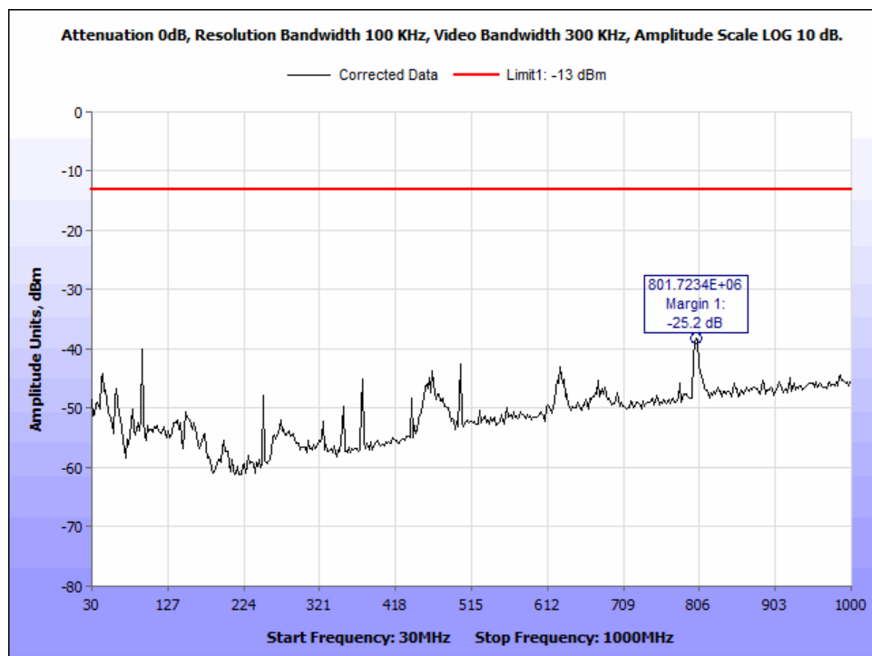
Figure 171: §25.202(f) Radiated Spurious Emissions, MissionLINK 200, Ch232_83.334kHz BW_30-1000MHz.
