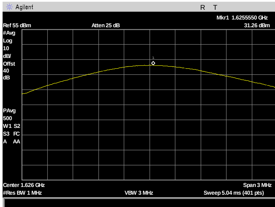
Figure 81: §25.204(a) Conducted RF Output Power, VesseLINK AVG_Output Power_ch232_333.333kHz BW
