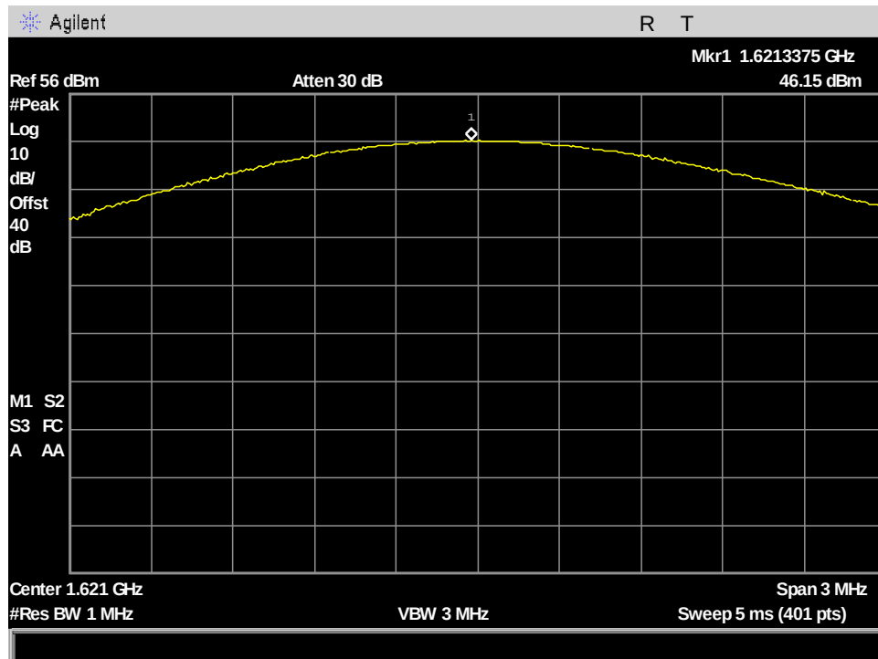
Figure 63: §25.204(a) Conducted RF Output Power, MissionLINK PK_Output Power_ch121_666.666kHz BW
