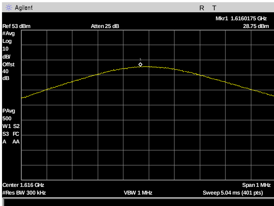
Figure 80: §25.204(a) Conducted RF Output Power, VesseLINK AVG_Output Power_ch1_83.334kHz BW
