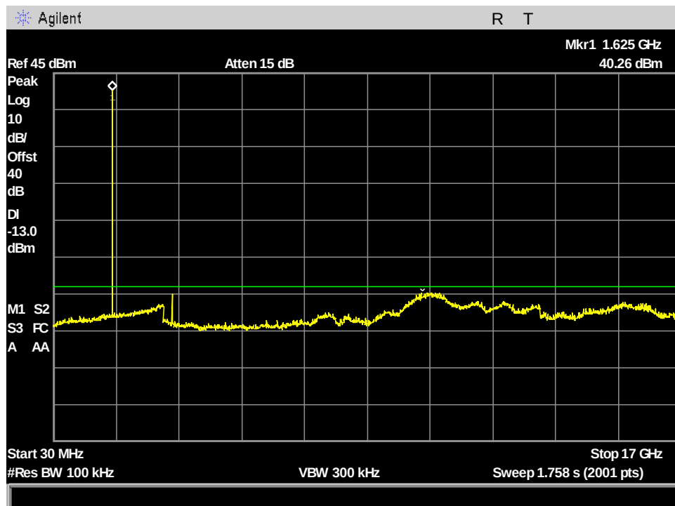
Figure 128: §25.202(f) VesseLINK Spurious Emissions at Antenna Terminals, ch121_333.333kHz_30MHz - 17GHz
