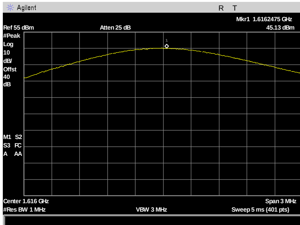
Figure 65: §25.204(a) Conducted RF Output Power, MissionLINK PK_Output Power_ch1_333.333kHz BW
