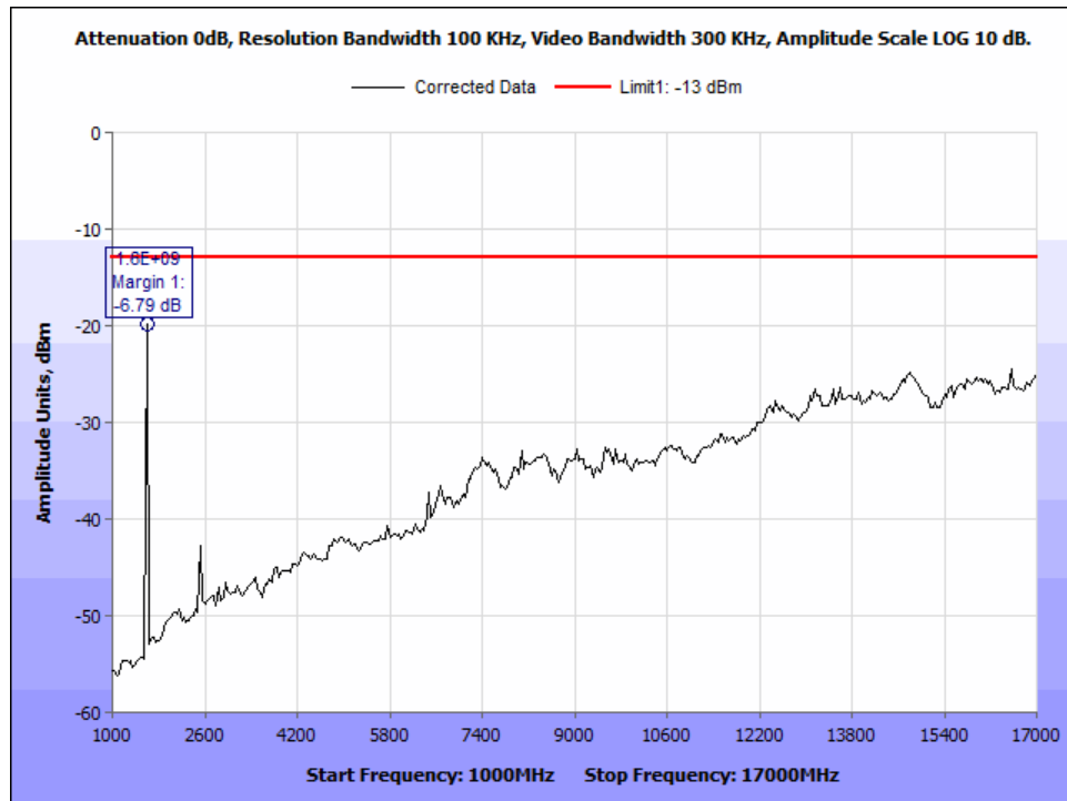
Figure 156: §25.202(f) Radiated Spurious Emissions, MissionLINK 200, Ch1_333.333kHz BW_1-17 GHz.
