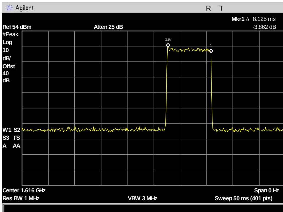
Figure 44: §25.204(a) Conducted RF Output Power, 41.668kHz_Ton
