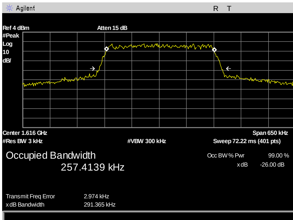
Figure 101: §2.1049(b) Occupied Bandwidth, Ch1_OBW_333.333kHz
