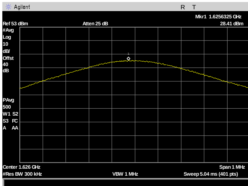
Figure 82: §25.204(a) Conducted RF Output Power, VesseLINK AVG_Output Power_ch232_41.668kHz BW
