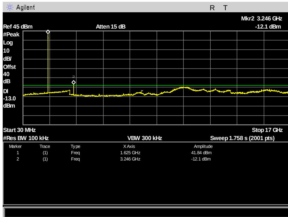
Figure 111: §25.202(f) MissionLINK Spurious Emissions at Antenna Terminals, ch121_41.668kHz_30MHz - 17GHz
