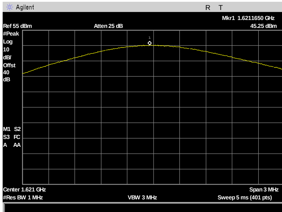
Figure 61: §25.204(a) Conducted RF Output Power, MissionLINK PK_Output Power_ch121_333.333kHz BW
