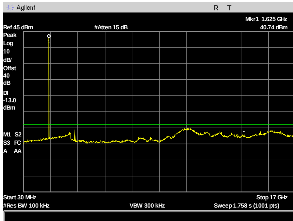
Figure 139: §25.202(f) VesseLINK Spurious Emissions at Antenna Terminals, ch232_83.334kHz_30MHz - 17GHz
