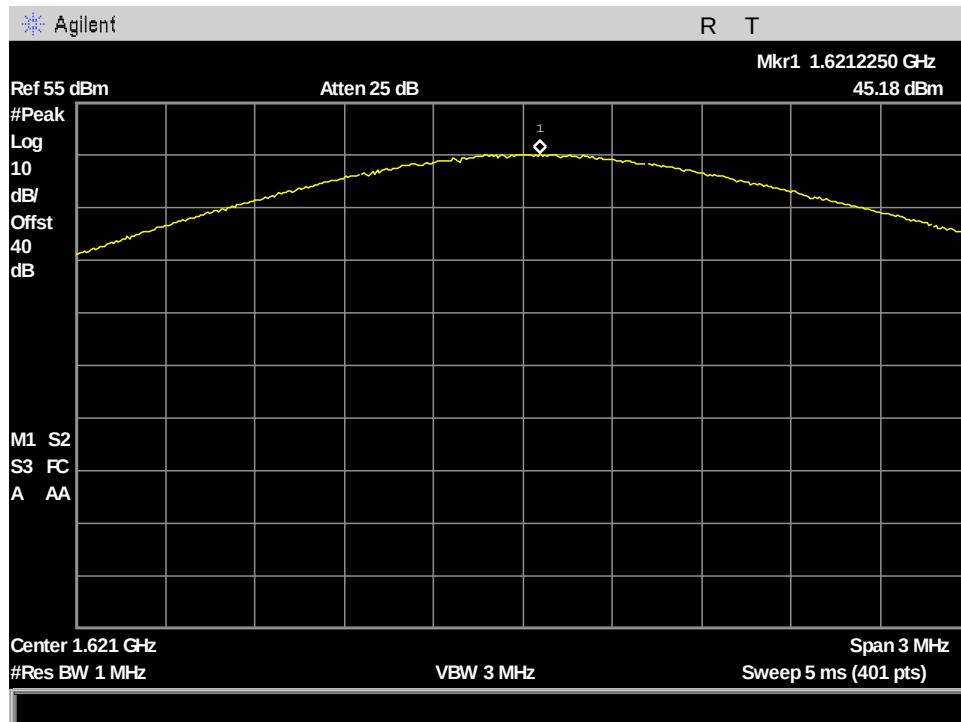
Figure 85: §25.204(a) Conducted RF Output Power, VesseLINK PK_Output Power_ch121_333.333kHz BW
