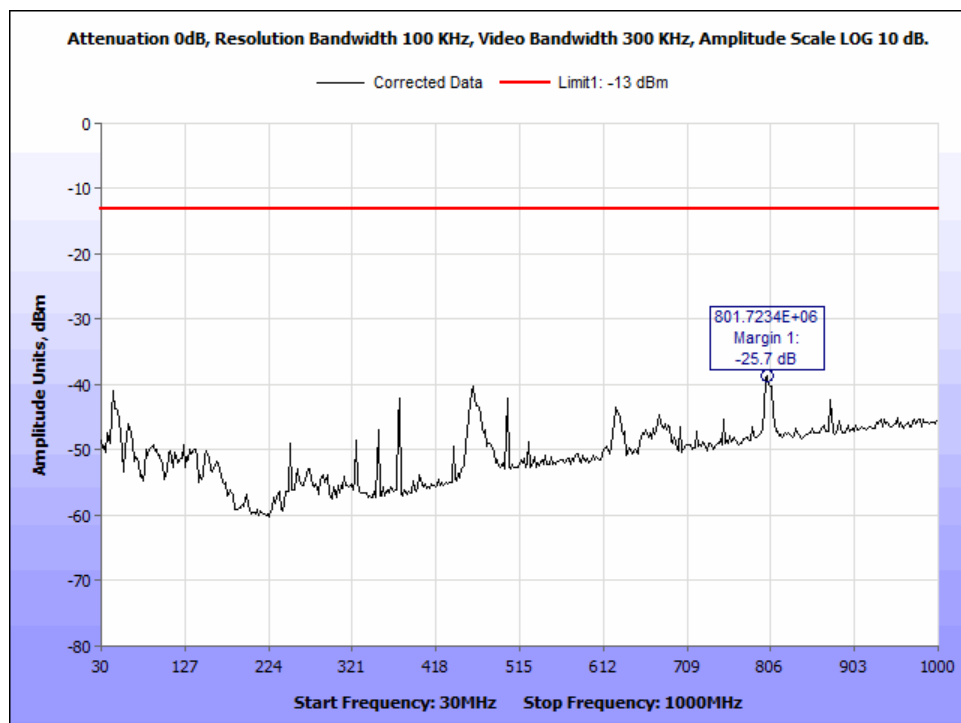
Figure 159: §25.202(f) Radiated Spurious Emissions, MissionLINK 200, Ch1_41.668kHz BW_30-1000MHz.
