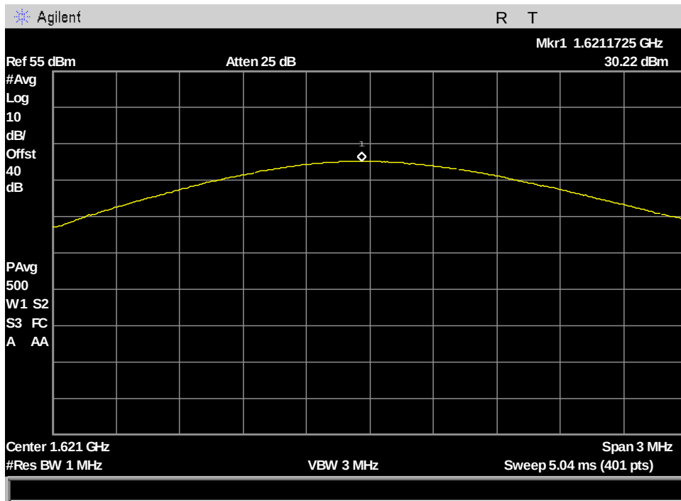
Figure 49: §25.204(a) Conducted RF Output Power, MissionLINK AVG_Output Power_ch121_333.333kHz BW
