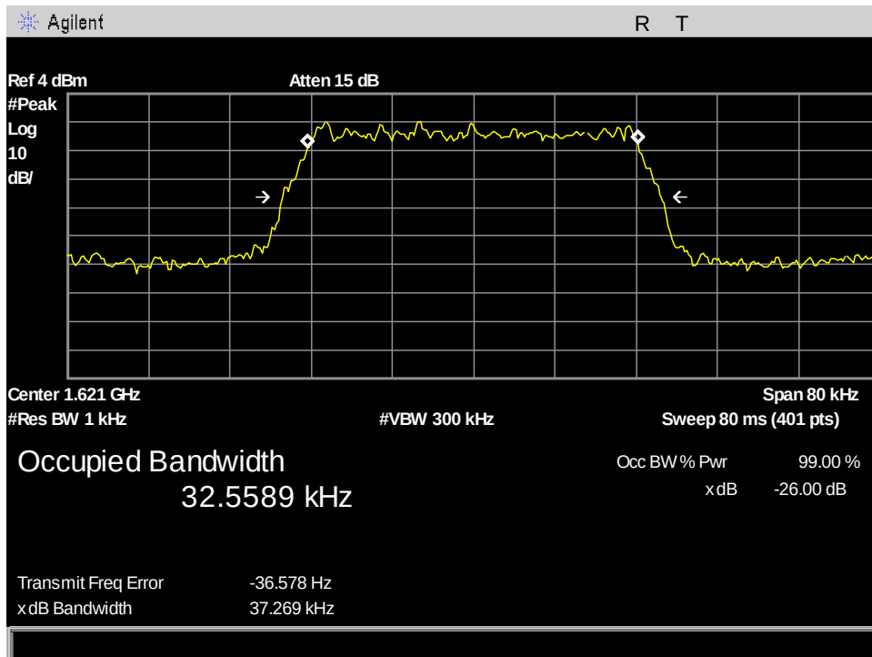
Figure 98: §2.1049(b) Occupied Bandwidth, Ch121_OBW_41.668kHz
