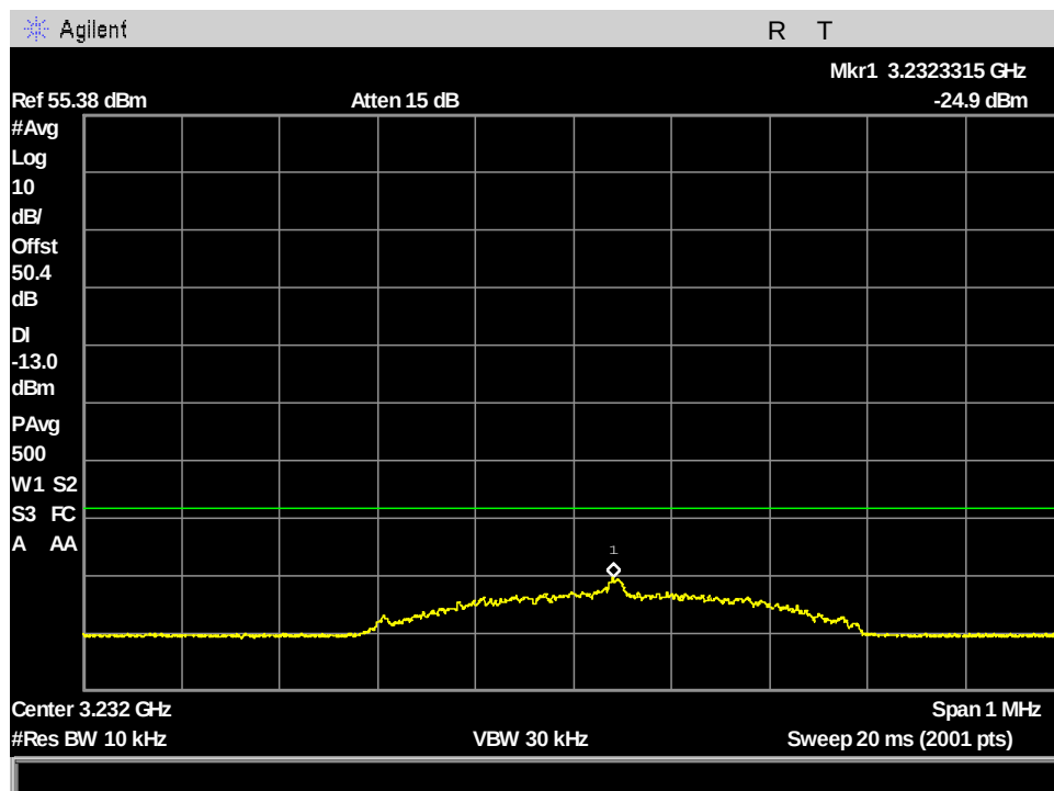
Figure 114: §25.202(f) MissionLINK Spurious Emissions at Antenna Terminals, ch1_333.333kHz_2x harmonic Avg measurement
