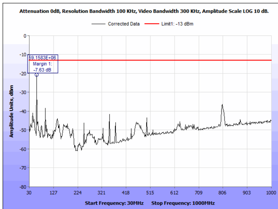
Figure 165: §25.202(f) Radiated Spurious Emissions, MissionLINK 200, Ch232_333.333kHz BW_30-1000MHz.
