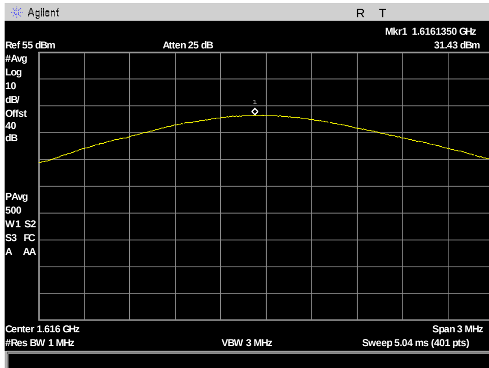
Figure 53: §25.204(a) Conducted RF Output Power, MissionLINK AVG_Output Power_ch1_333.333kHz BW
