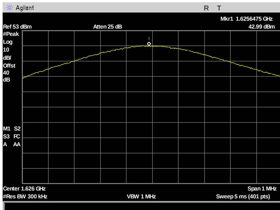
Figure 94: §25.204(a) Conducted RF Output Power, VesseLINK PK_Output Power_ch232_41.668kHz BW
