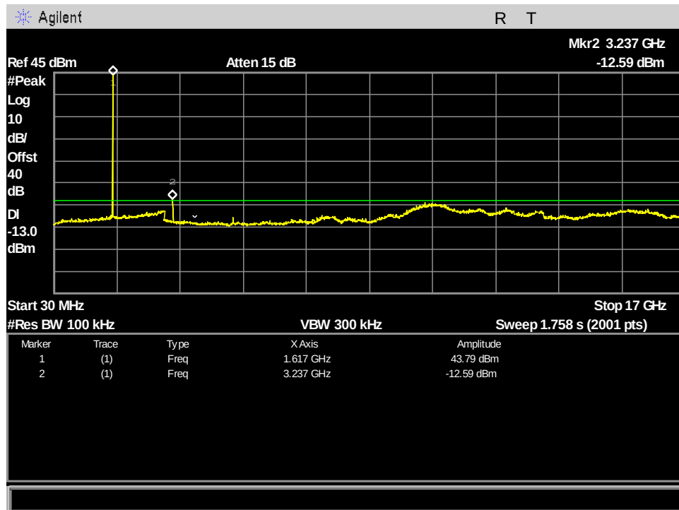
Figure 115: §25.202(f) MissionLINK Spurious Emissions at Antenna Terminals, ch1_333.333kHz_30MHz - 17GHz
