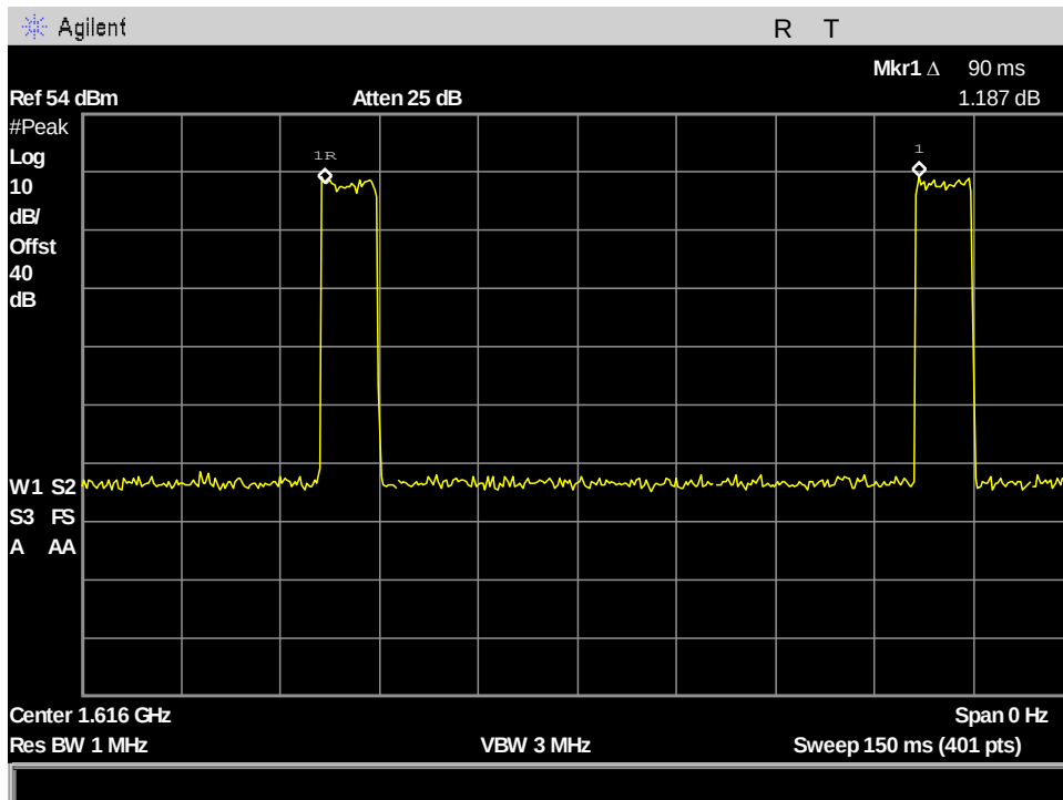
Figure 43: §25.204(a) Conducted RF Output Power, 41.668kHz_Period
