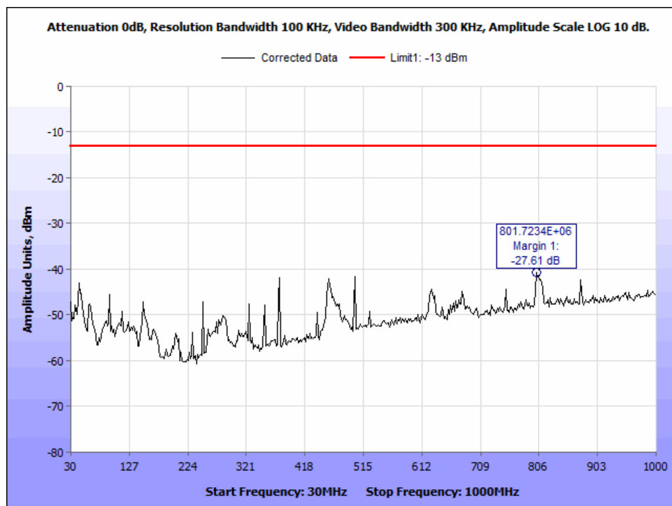
Figure 155: §25.202(f) Radiated Spurious Emissions, MissionLINK 200, Ch121_83.334kHz BW_30-1000MHz.
