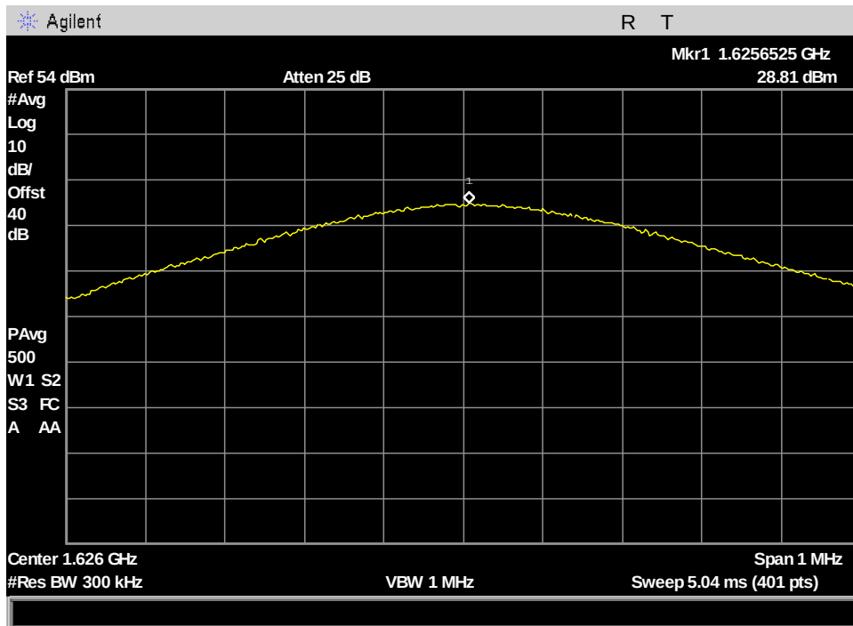
Figure 58: §25.204(a) Conducted RF Output Power, MissionLINK AVG_Output Power_ch232_41.668kHz BW
