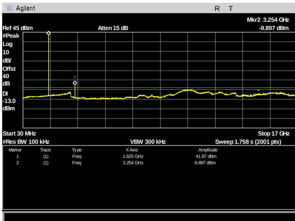
Figure 124: §25.202(f) MissionLINK Spurious Emissions at Antenna Terminals, ch232_41.668kHz_30MHz - 17GHz
