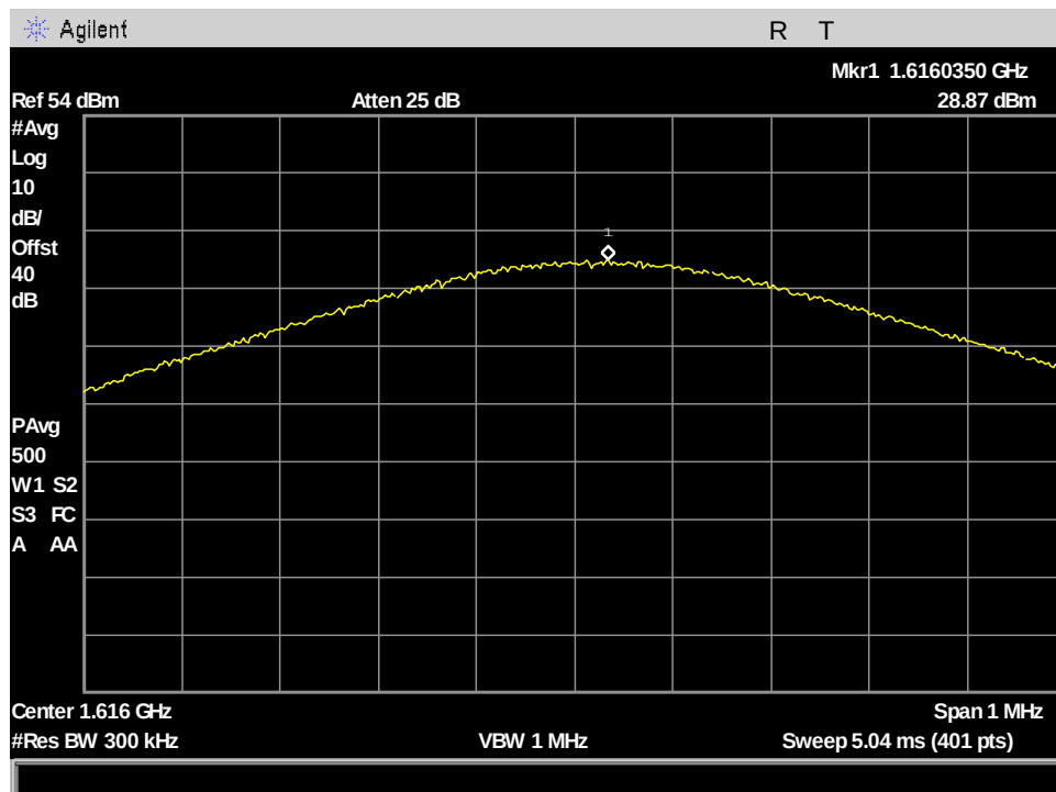
Figure 54: §25.204(a) Conducted RF Output Power, MissionLINK AVG_Output Power_ch1_41.668kHz BW
