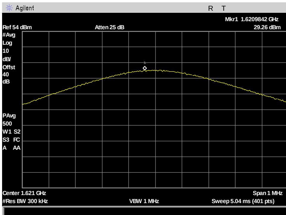
Figure 74: §25.204(a) Conducted RF Output Power, VesseLINK AVG_Output Power_ch121_41.668kHz BW
