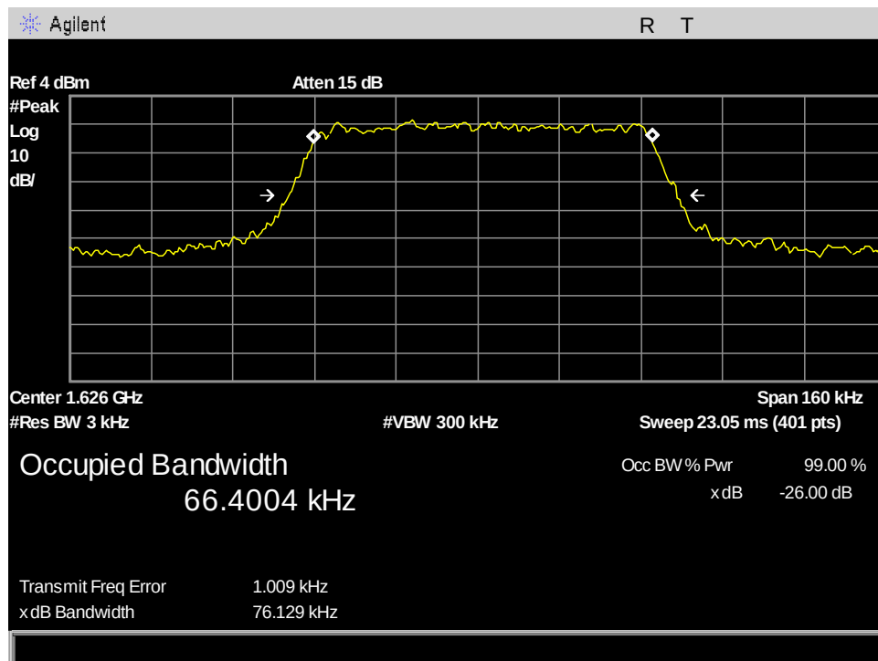
Figure 108: §2.1049(b) Occupied Bandwidth, Ch232_OBW_83.334kHz
