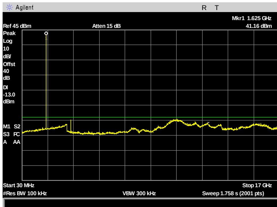
Figure 136: §25.202(f) VesseLINK Spurious Emissions at Antenna Terminals, ch232_333.333kHz_30MHz - 17GHz
