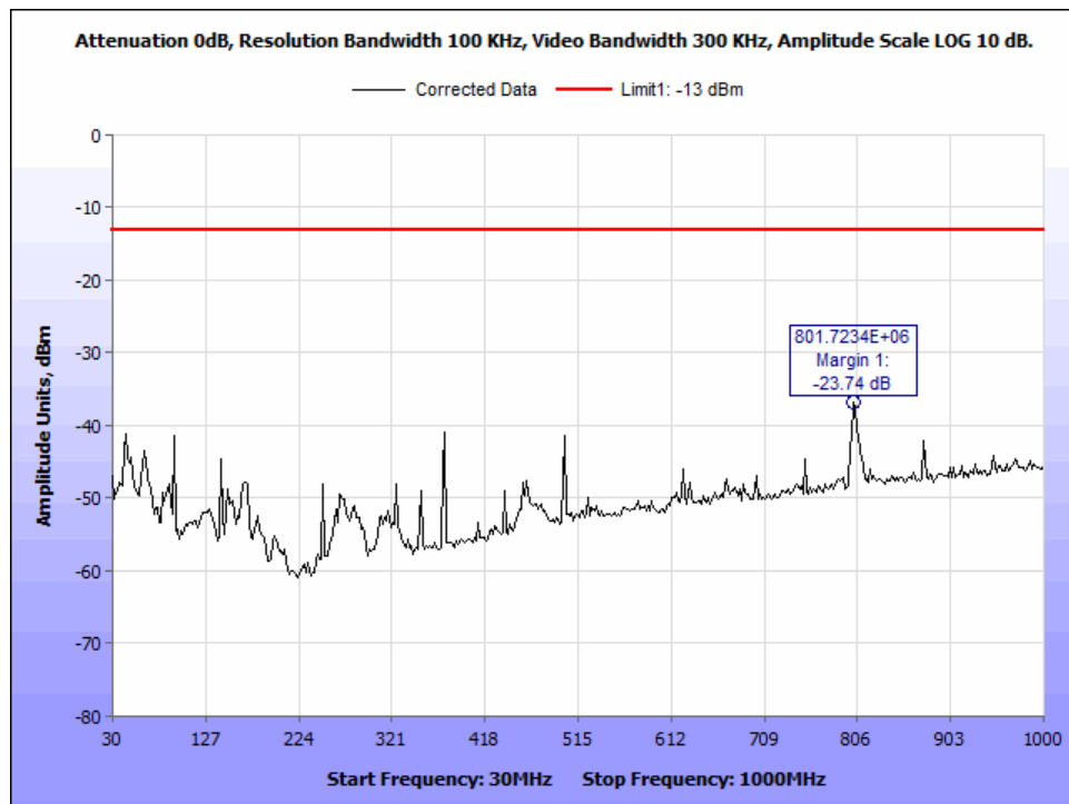
Figure 161: §25.202(f) Radiated Spurious Emissions, MissionLINK 200, Ch1_666.666kHz BW_30-1000MHz.
