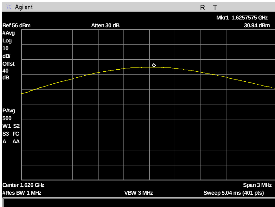
Figure 83: §25.204(a) Conducted RF Output Power, VesseLINK AVG_Output Power_ch232_666.666kHz BW
