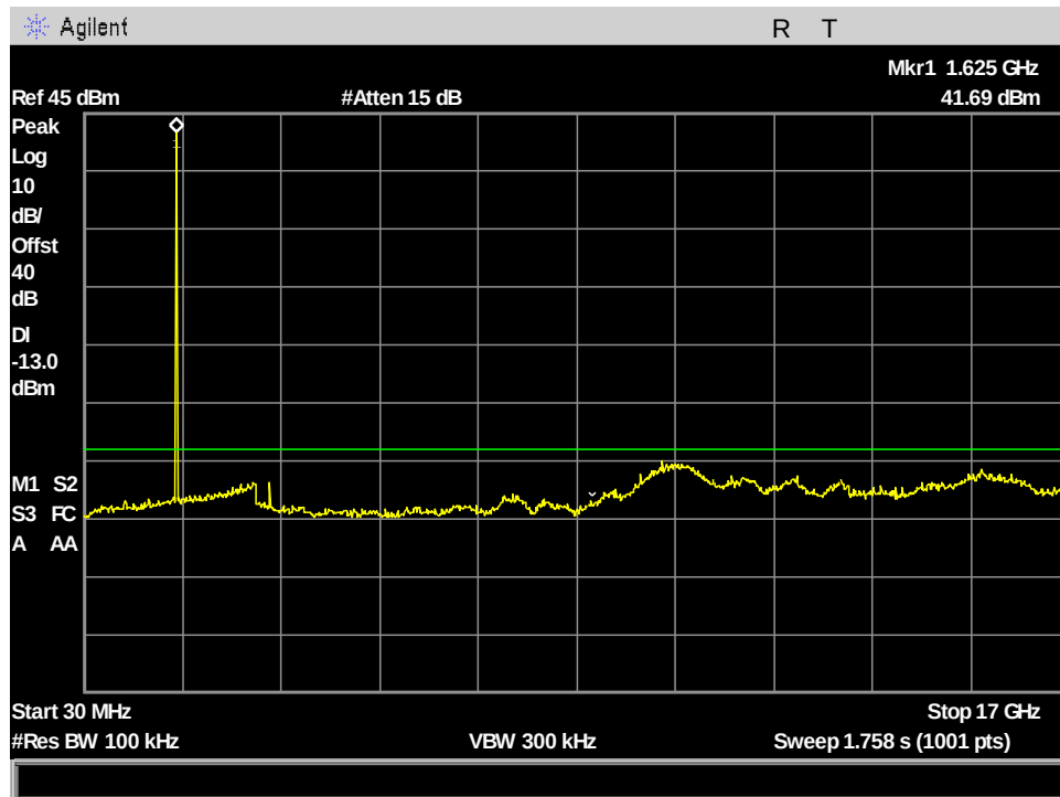
Figure 131: §25.202(f) VesseLINK Spurious Emissions at Antenna Terminals, ch121_83.334kHz_30MHz - 17GHz
