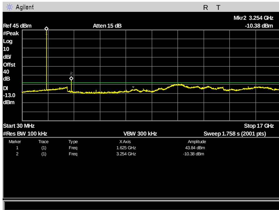
Figure 127: §25.202(f) MissionLINK Spurious Emissions at Antenna Terminals, ch232_83.334kHz_30MHz - 17GHz
