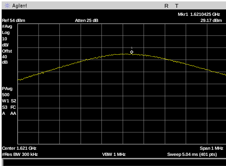
Figure 50: §25.204(a) Conducted RF Output Power, MissionLINK AVG_Output Power_ch121_41.668kHz BW
