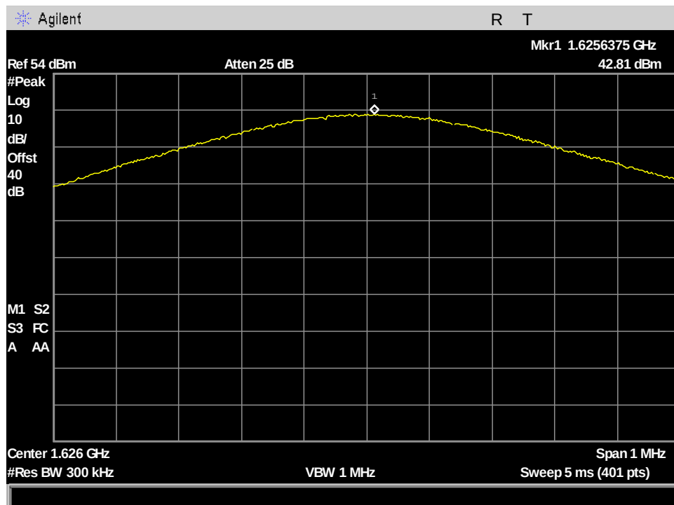
Figure 72: §25.204(a) Conducted RF Output Power, MissionLINK PK_Output Power_ch232_83.334kHz BW
