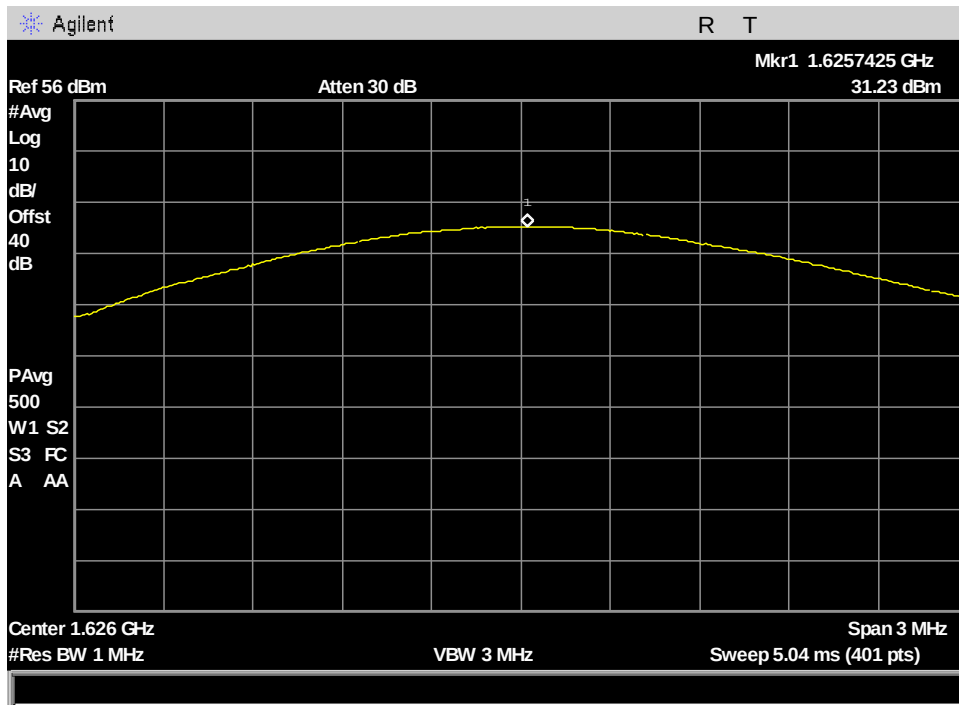
Figure 59: §25.204(a) Conducted RF Output Power, MissionLINK AVG_Output Power_ch232_666.666kHz BW
