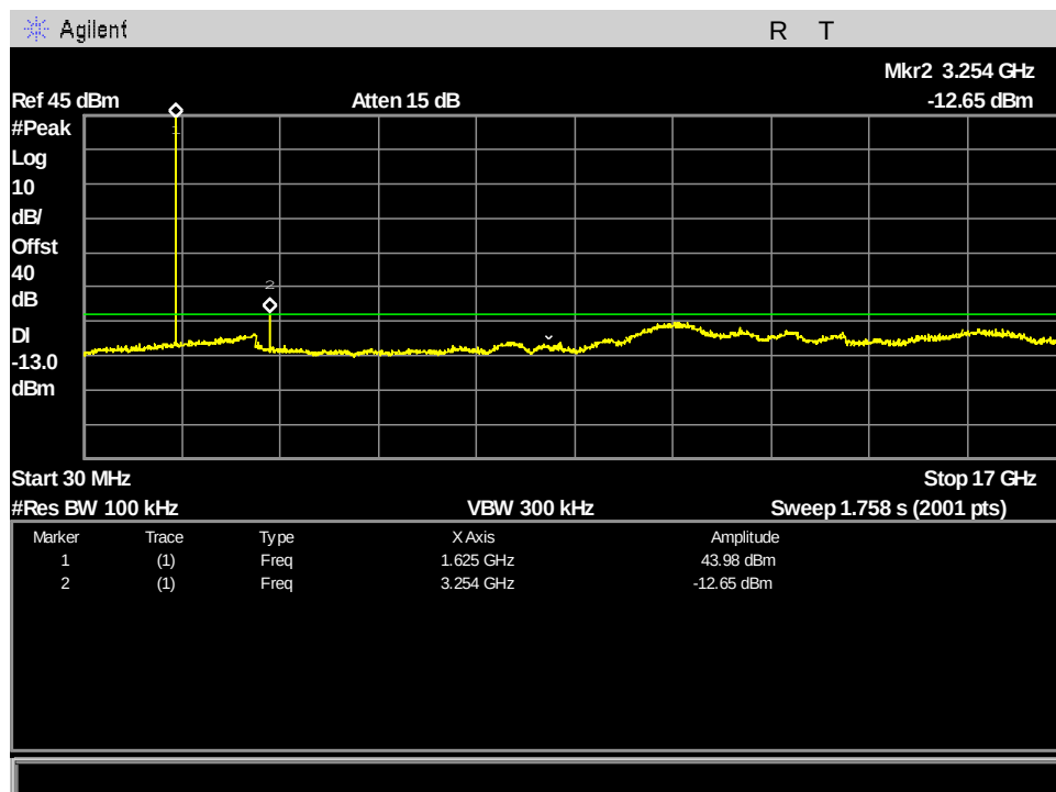
Figure 122: §25.202(f) MissionLINK Spurious Emissions at Antenna Terminals, ch232_333.333kHz_30MHz - 17GHz
