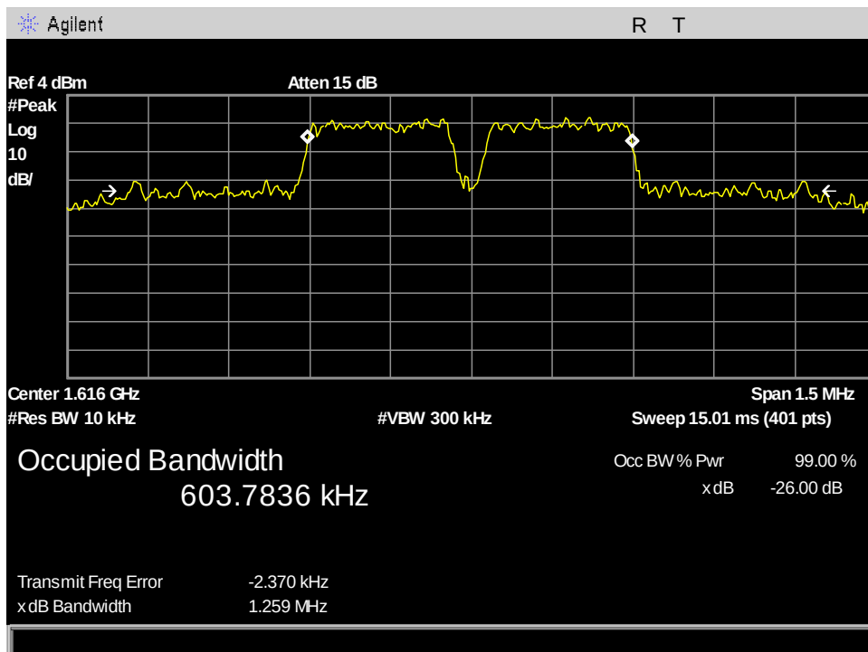
Figure 103: §2.1049(b) Occupied Bandwidth, Ch1_OBW_666.666kHz
