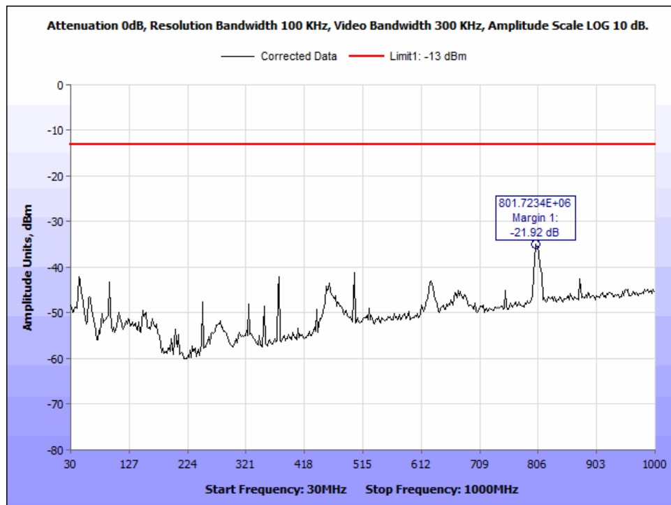
Figure 167: §25.202(f) Radiated Spurious Emissions, MissionLINK 200, Ch232_41.668kHz BW_30-1000MHz.
