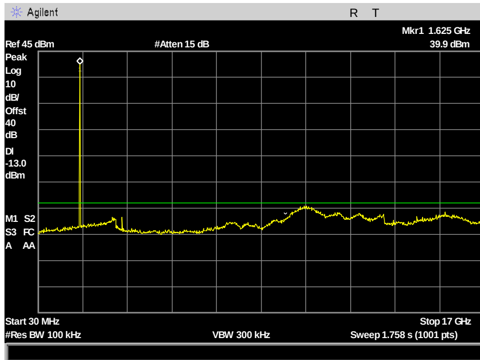
Figure 133: §25.202(f) VesseLINK Spurious Emissions at Antenna Terminals, ch1_41.668kHz_30MHz - 17GHz
