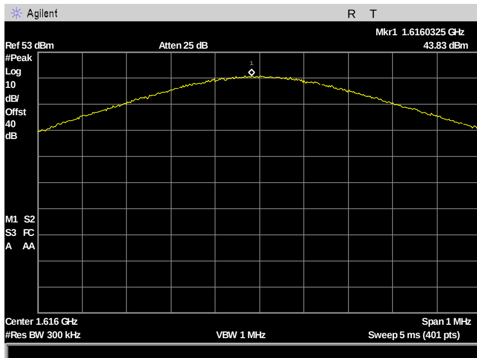
Figure 92: §25.204(a) Conducted RF Output Power, VesseLINK PK_Output Power_ch1_83.334kHz BW
