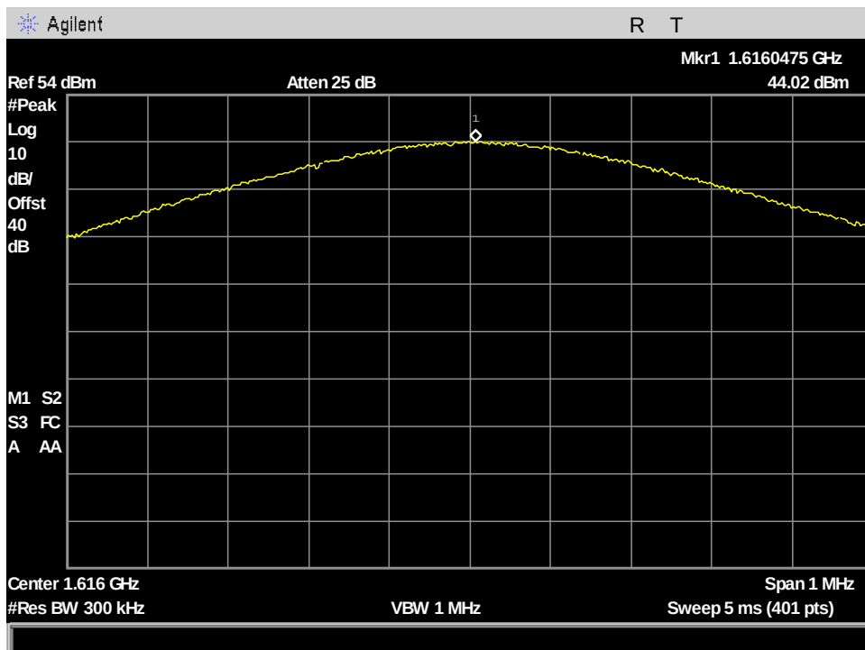
Figure 68: §25.204(a) Conducted RF Output Power, MissionLINK PK_Output Power_ch1_83.334kHz BW
