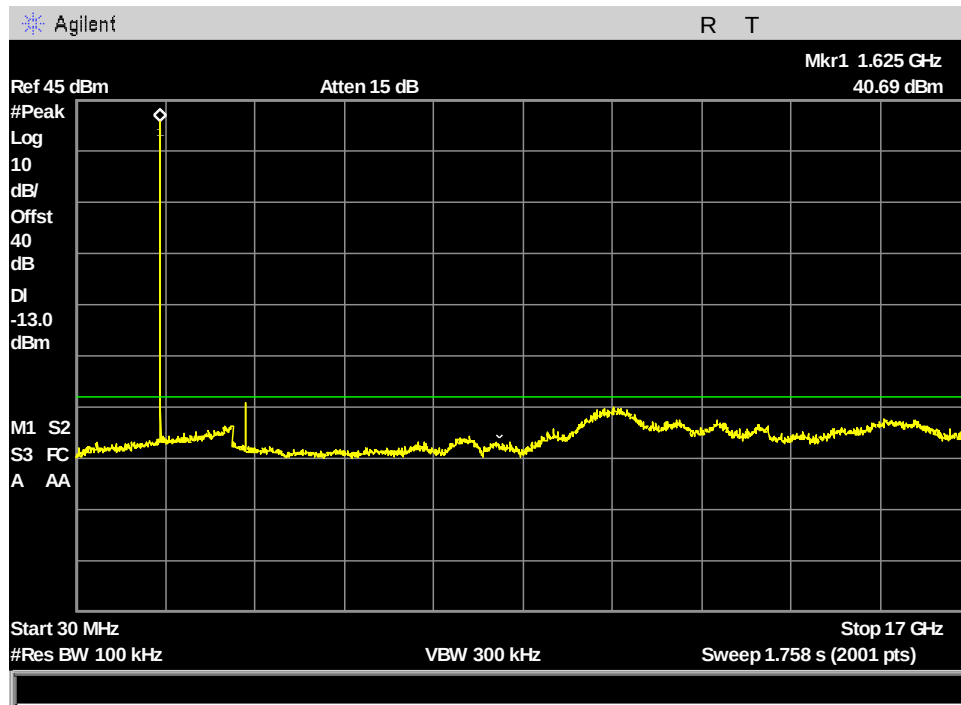
Figure 125: §25.202(f) MissionLINK Spurious Emissions at Antenna Terminals, ch232_666.666kHz_30MHz - 17GHz
