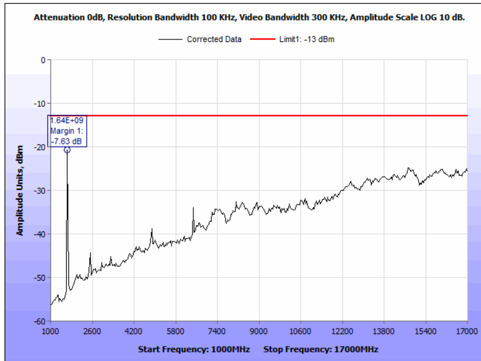
Figure 152: §25.202(f) Radiated Spurious Emissions, MissionLINK 200, Ch121_666.666kHz BW_1-17 GHz.
