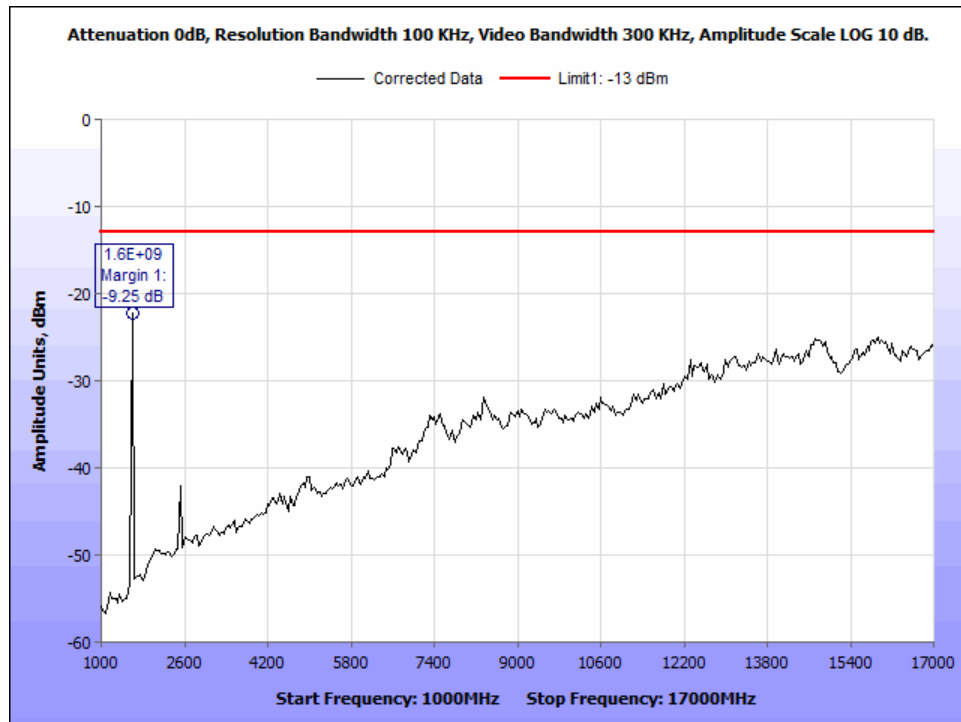
Figure 158: §25.202(f) Radiated Spurious Emissions, MissionLINK 200, Ch1_41.668kHz BW_1-17 GHz.
