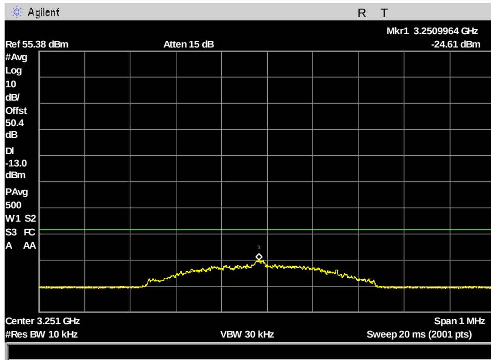
Figure 121: §25.202(f) MissionLINK Spurious Emissions at Antenna Terminals, ch232_333.333kHz_2x harmonic Avg measurement
