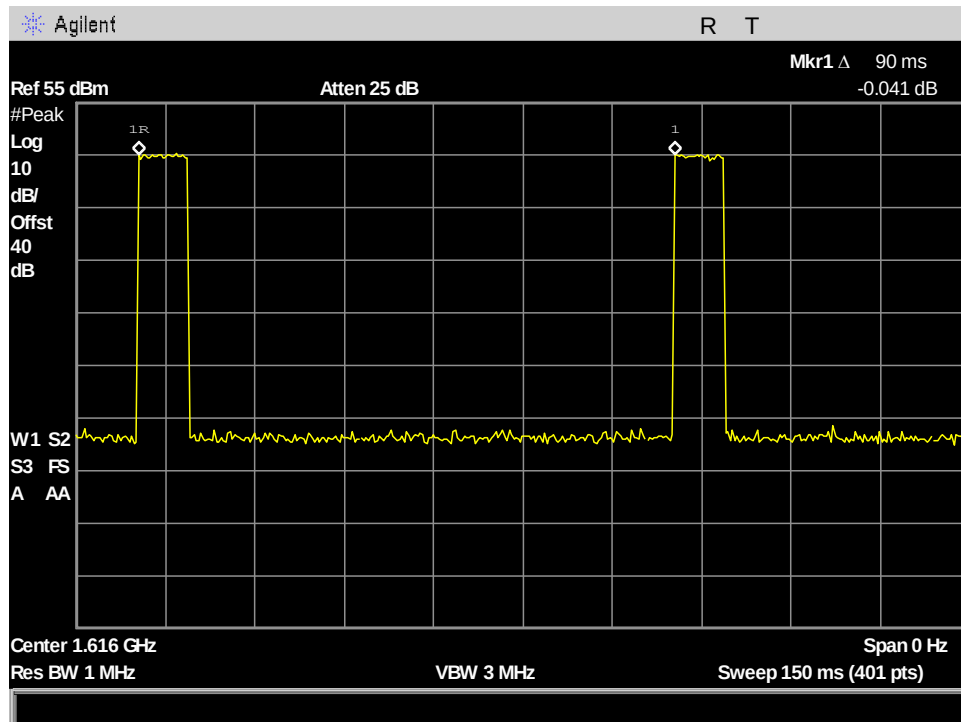
Figure 41: §25.204(a) Conducted RF Output Power, 333.333kHz_Period
