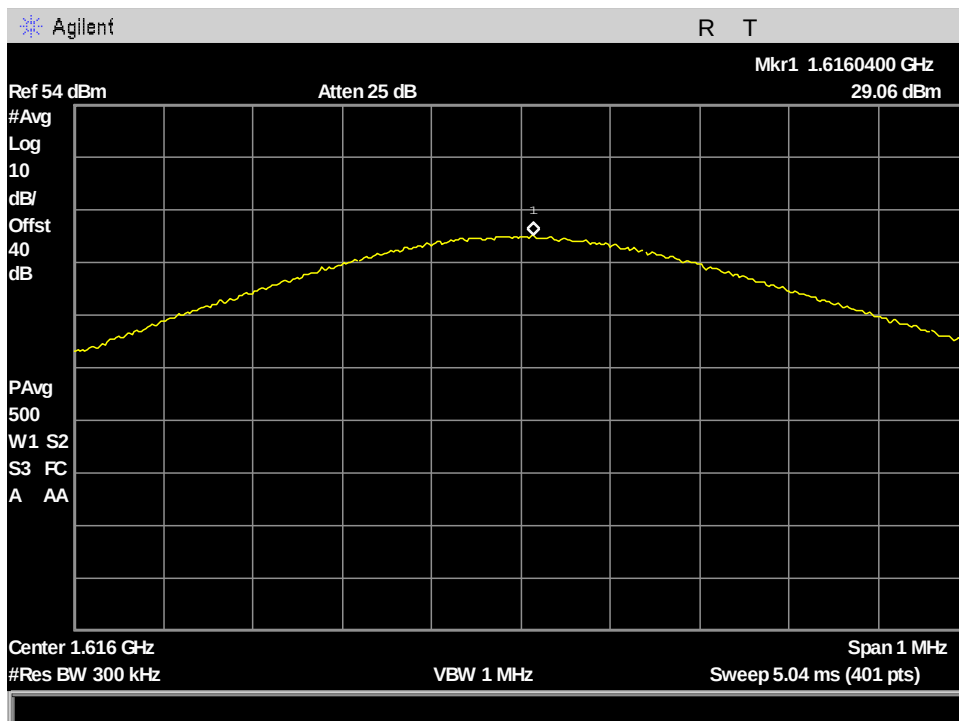
Figure 78: §25.204(a) Conducted RF Output Power, VesseLINK AVG_Output Power_ch1_41.668kHz BW
