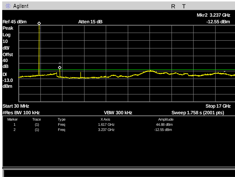
Figure 117: §25.202(f) MissionLINK Spurious Emissions at Antenna Terminals, ch1_41.668kHz_30MHz - 17GHz
