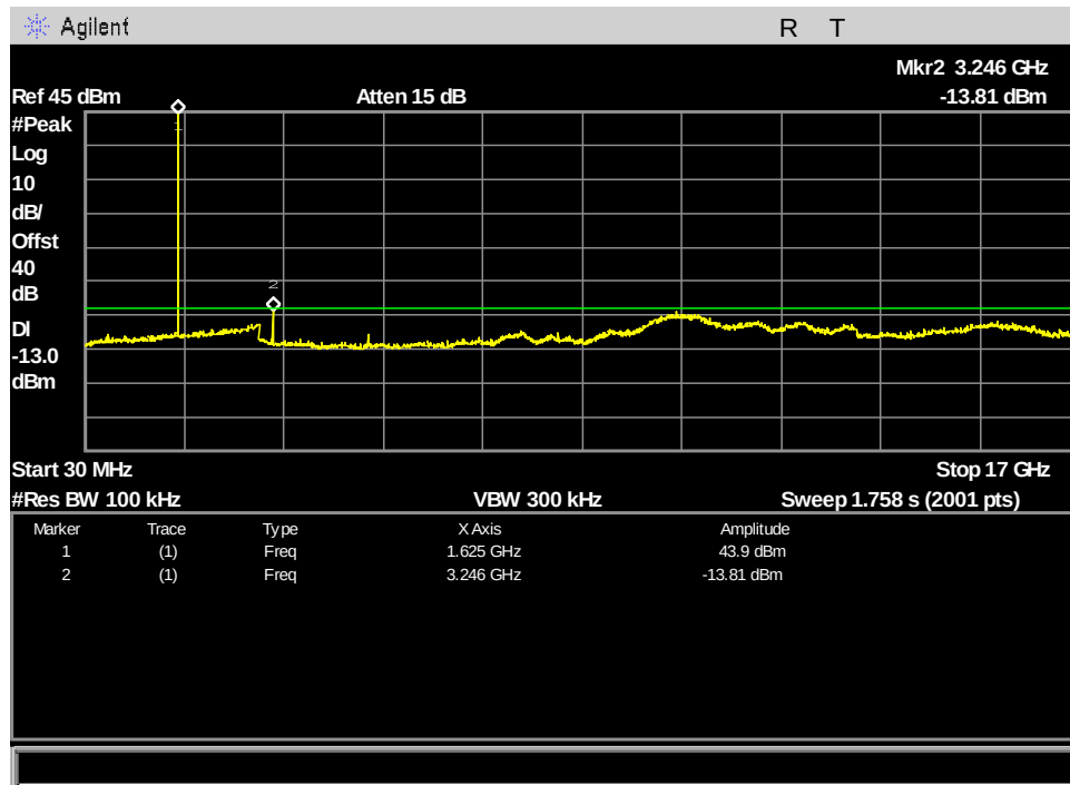
Figure 113: §25.202(f) MissionLINK Spurious Emissions at Antenna Terminals, ch121_83.334kHz_30MHz - 17GHz
