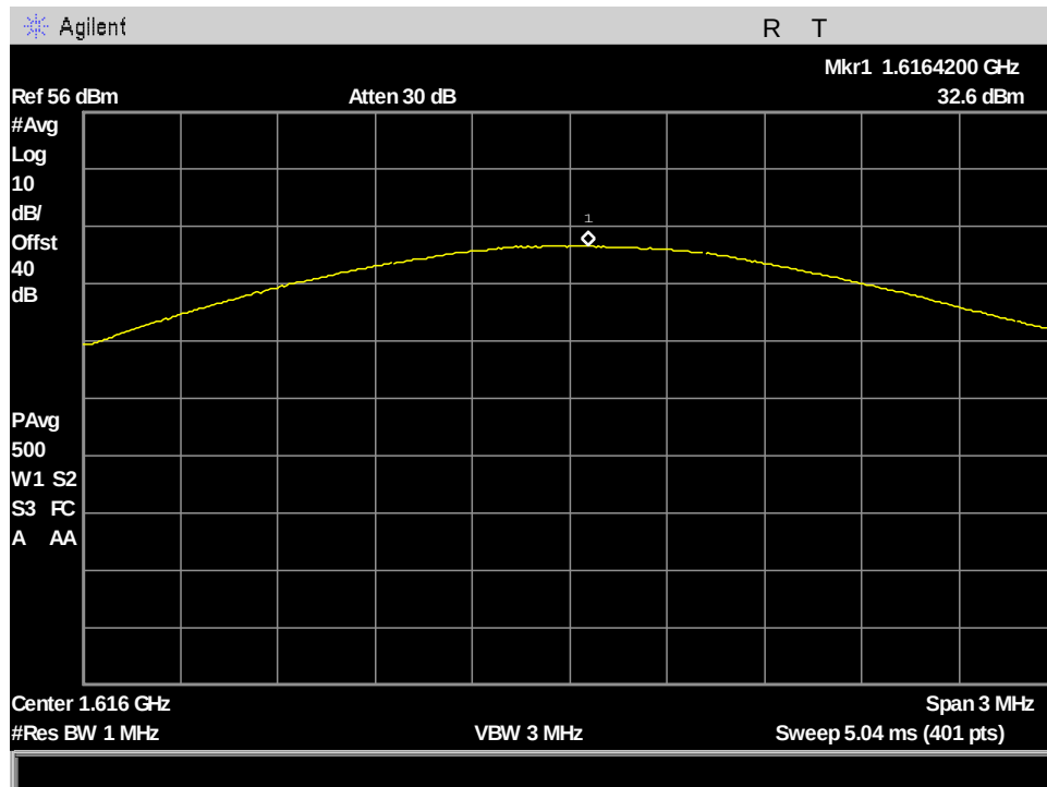
Figure 55: §25.204(a) Conducted RF Output Power, MissionLINK AVG_Output Power_ch1_666.666kHz BW
