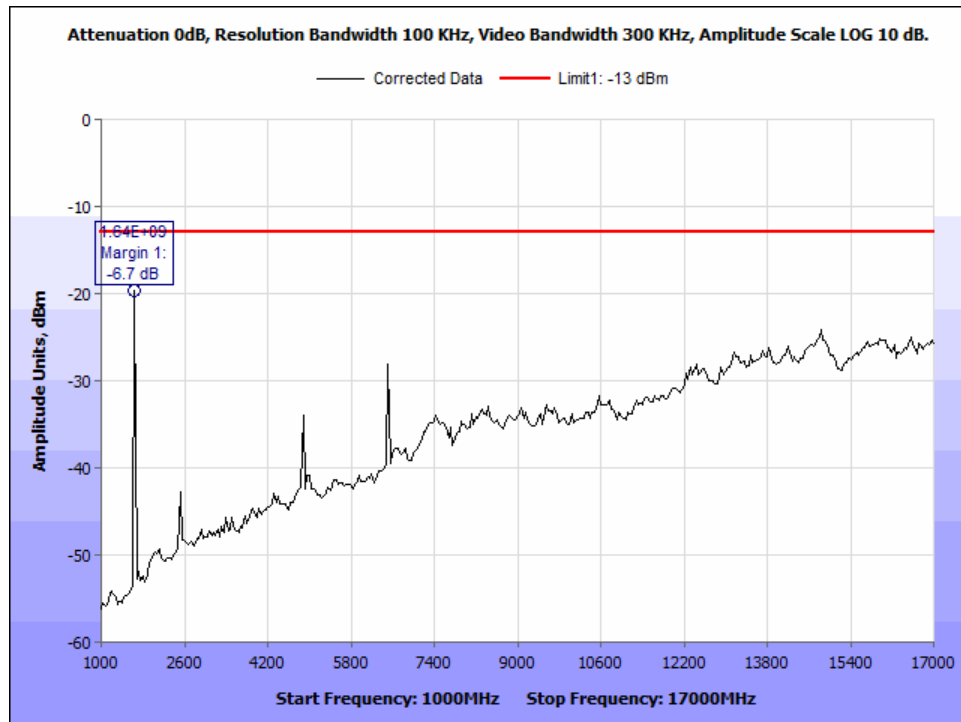
Figure 168: §25.202(f) Radiated Spurious Emissions, MissionLINK 200, Ch232_666.666kHz BW_1-17 GHz.
