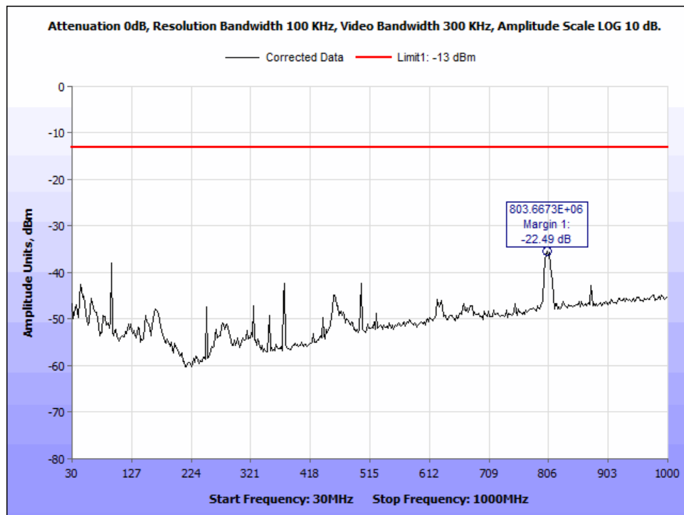
Figure 153: §25.202(f) Radiated Spurious Emissions, MissionLINK 200, Ch121_666.666kHz BW_30-1000MHz.
