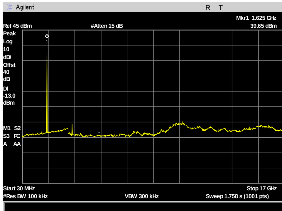
Figure 137: §25.202(f) VesseLINK Spurious Emissions at Antenna Terminals, ch232_41.668kHz_30MHz - 17GHz
