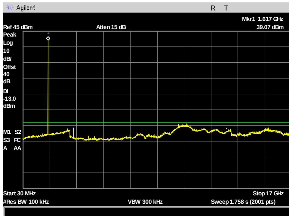
Figure 134: §25.202(f) VesseLINK Spurious Emissions at Antenna Terminals, ch1_666.666kHz_30MHz - 17GHz
