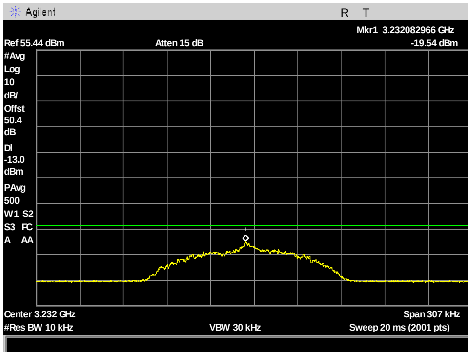
Figure 119: §25.202(f) MissionLINK Spurious Emissions at Antenna Terminals, ch1_83.334kHz_2x harmonic Avg measurement
