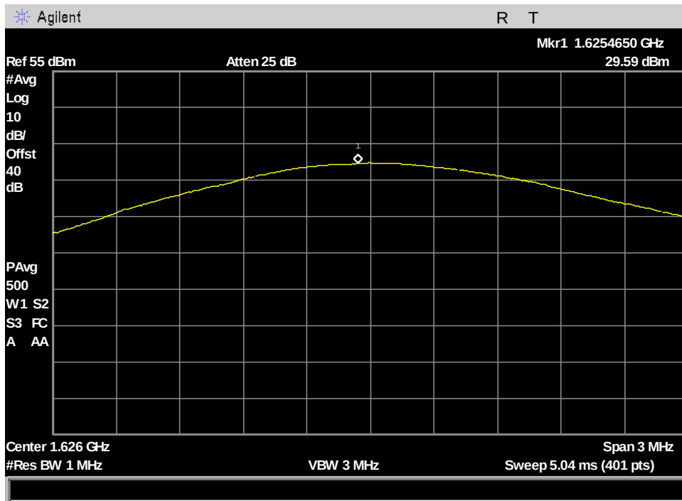
Figure 57: §25.204(a) Conducted RF Output Power, MissionLINK AVG_Output Power_ch232_333.333kHz BW
