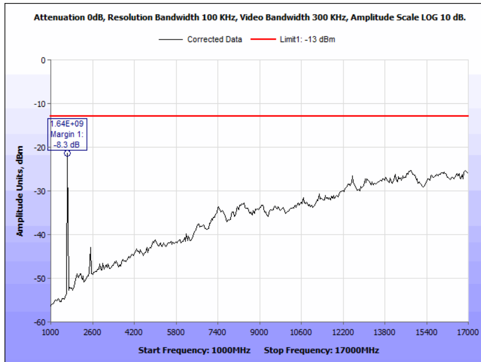
Figure 150: §25.202(f) Radiated Spurious Emissions, MissionLINK 200, Ch121_41.668kHz BW_1-17 GHz.
