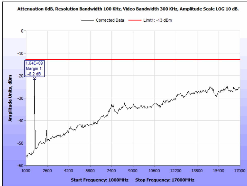
Figure 154: §25.202(f) Radiated Spurious Emissions, MissionLINK 200, Ch121_83.334kHz BW_1-17 GHz.
