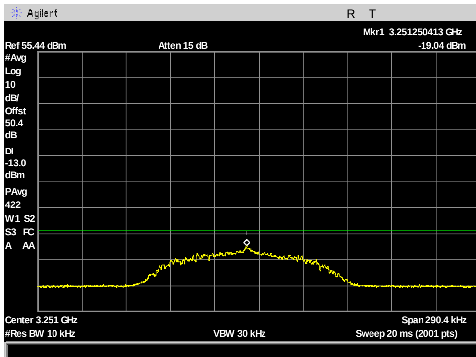
Figure 126: §25.202(f) MissionLINK Spurious Emissions at Antenna Terminals, ch232_83.334kHz_2x harmonic Avg measurement
