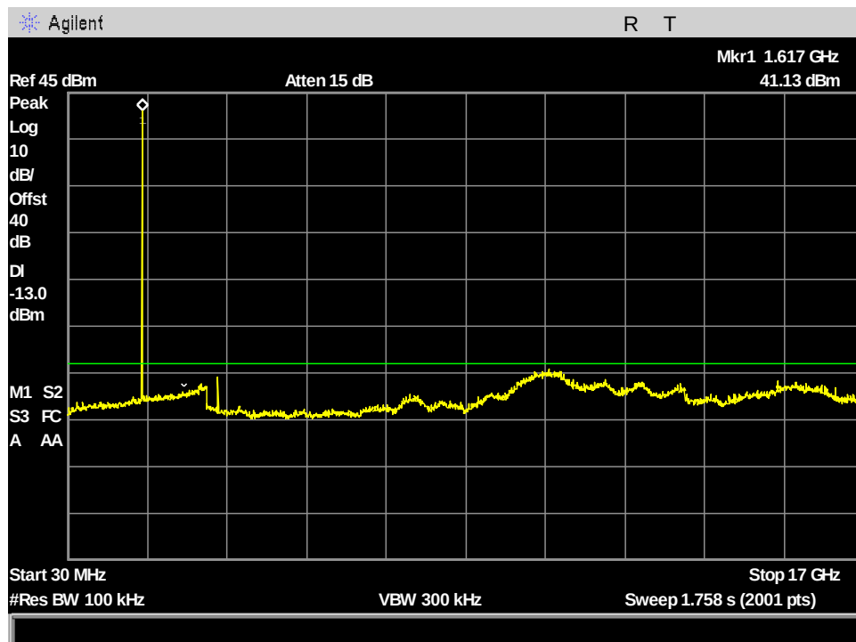
Figure 132: §25.202(f) VesseLINK Spurious Emissions at Antenna Terminals, ch1_333.333kHz_30MHz - 17GHz
