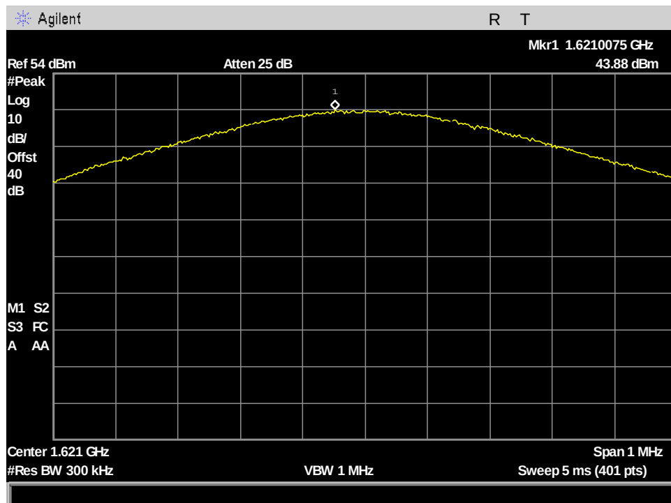
Figure 64: §25.204(a) Conducted RF Output Power, MissionLINK PK_Output Power_ch121_83.334kHz BW
