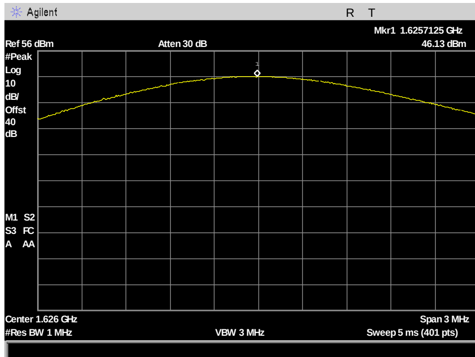
Figure 71: §25.204(a) Conducted RF Output Power, MissionLINK PK_Output Power_ch232_666.666kHz BW
