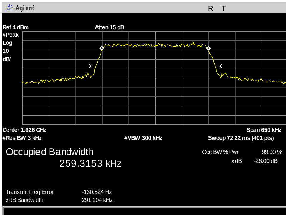
Figure 105: §2.1049(b) Occupied Bandwidth, Ch232_OBW_333.333kHz
