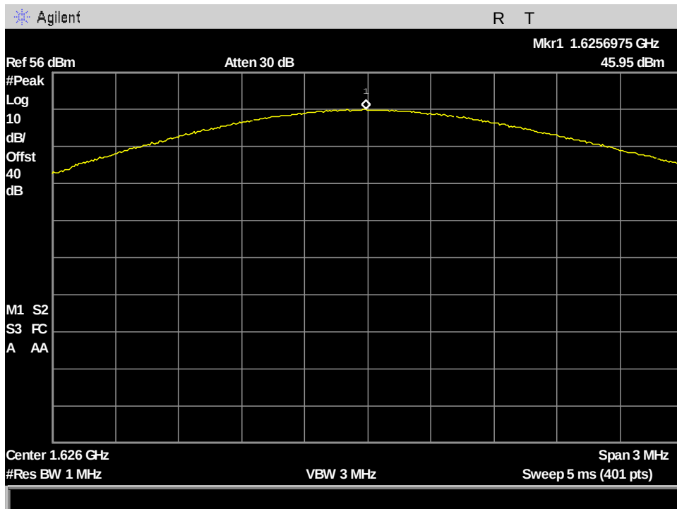
Figure 95: §25.204(a) Conducted RF Output Power, VesseLINK PK_Output Power_ch232_666.666kHz BW
