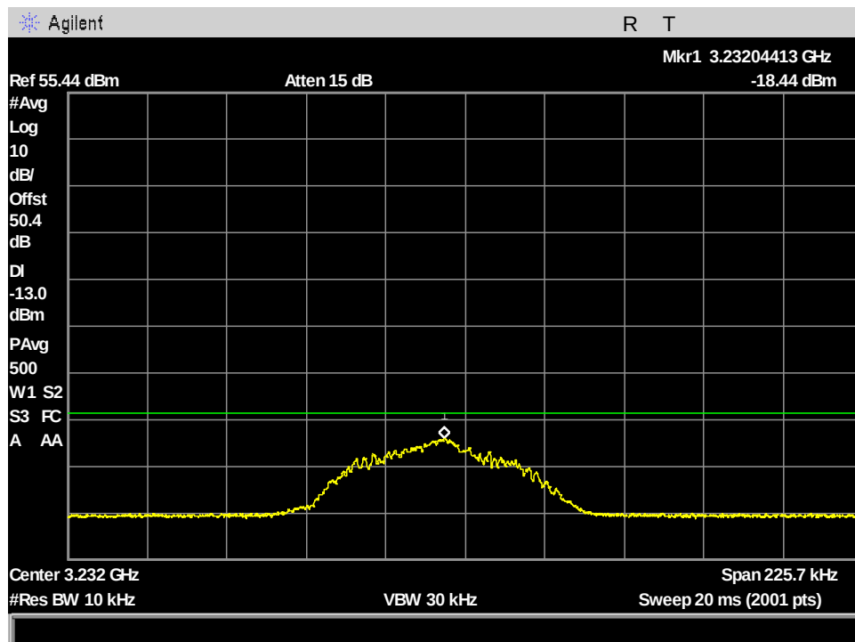
Figure 116: §25.202(f) MissionLINK Spurious Emissions at Antenna Terminals, ch1_41.668kHz_2x harmonic Avg measurement
