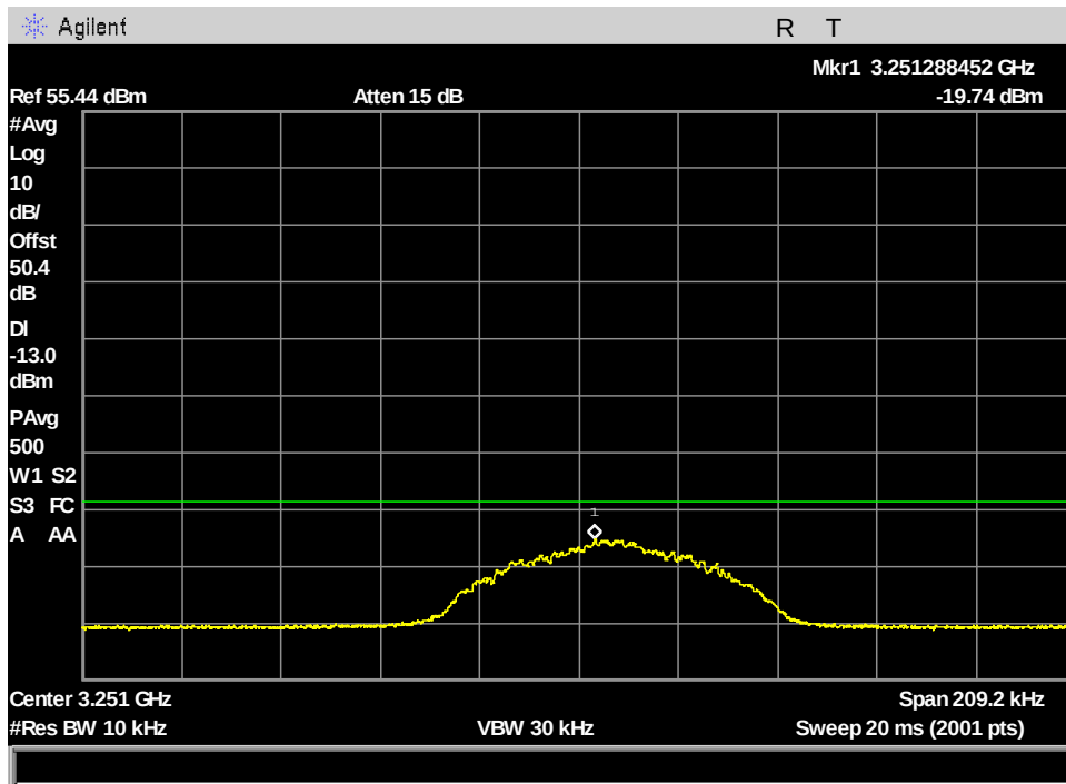
Figure 123: §25.202(f) MissionLINK Spurious Emissions at Antenna Terminals, ch232_41.668kHz_2x harmonic Avg measurement
