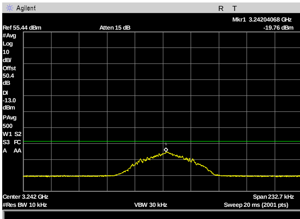
Figure 110: §25.202(f) MissionLINK Spurious Emissions at Antenna Terminals, ch121_41.668kHz_2x harmonic Avg measurement
