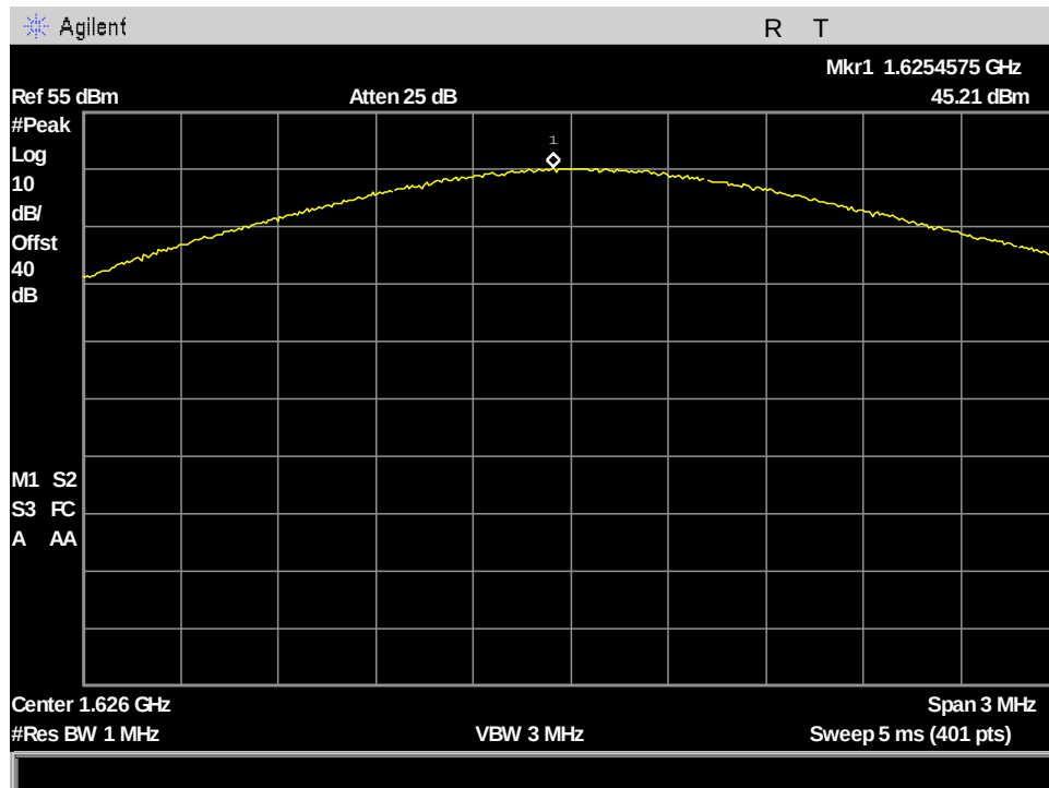
Figure 93: §25.204(a) Conducted RF Output Power, VesseLINK PK_Output Power_ch232_333.333kHz BW
