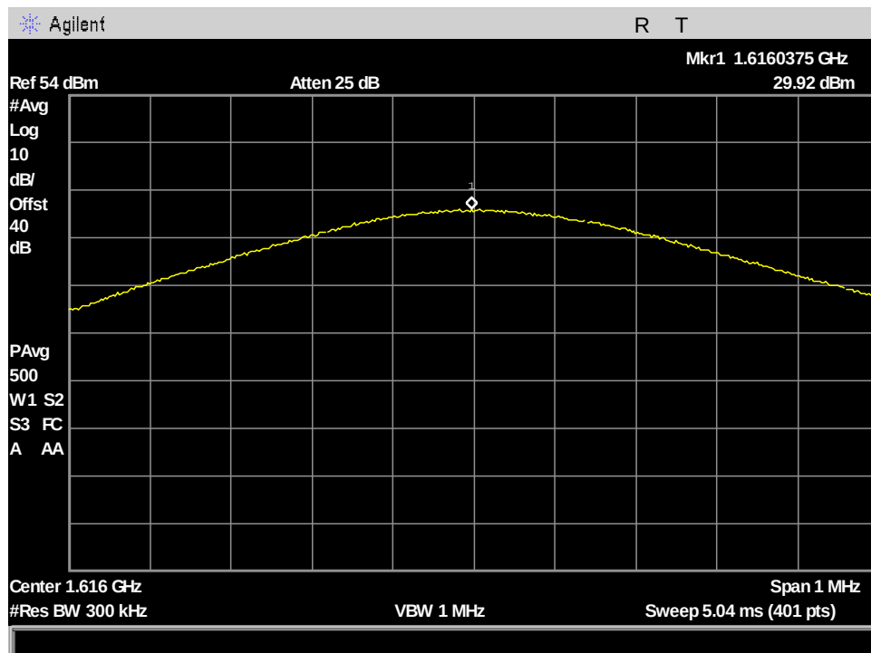
Figure 56: §25.204(a) Conducted RF Output Power, MissionLINK AVG_Output Power_ch1_83.334kHz BW
