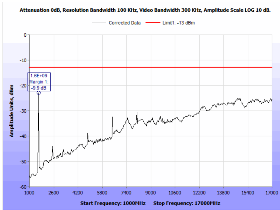
Figure 160: §25.202(f) Radiated Spurious Emissions, MissionLINK 200, Ch1_666.666kHz BW_1-17 GHz.
