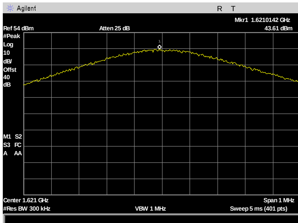
Figure 86: §25.204(a) Conducted RF Output Power, VesseLINK PK_Output Power_ch121_41.668kHz BW
