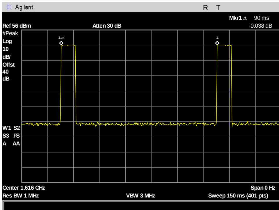
Figure 45: §25.204(a) Conducted RF Output Power, 666.666kHz_Period
