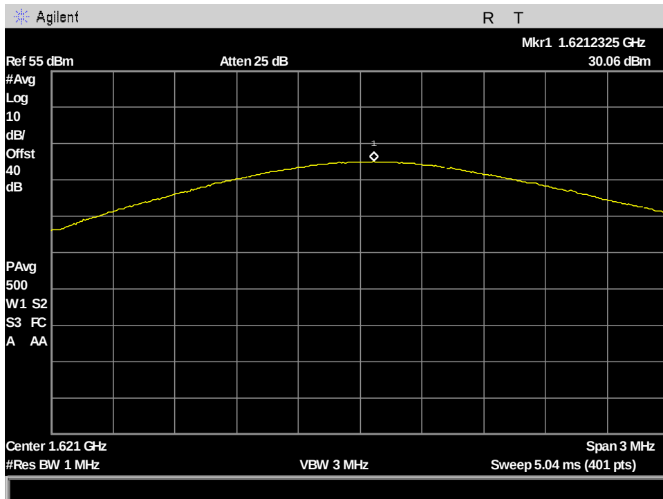
Figure 73: §25.204(a) Conducted RF Output Power, VesseLINK AVG_Output Power_ch121_333.333kHz BW
