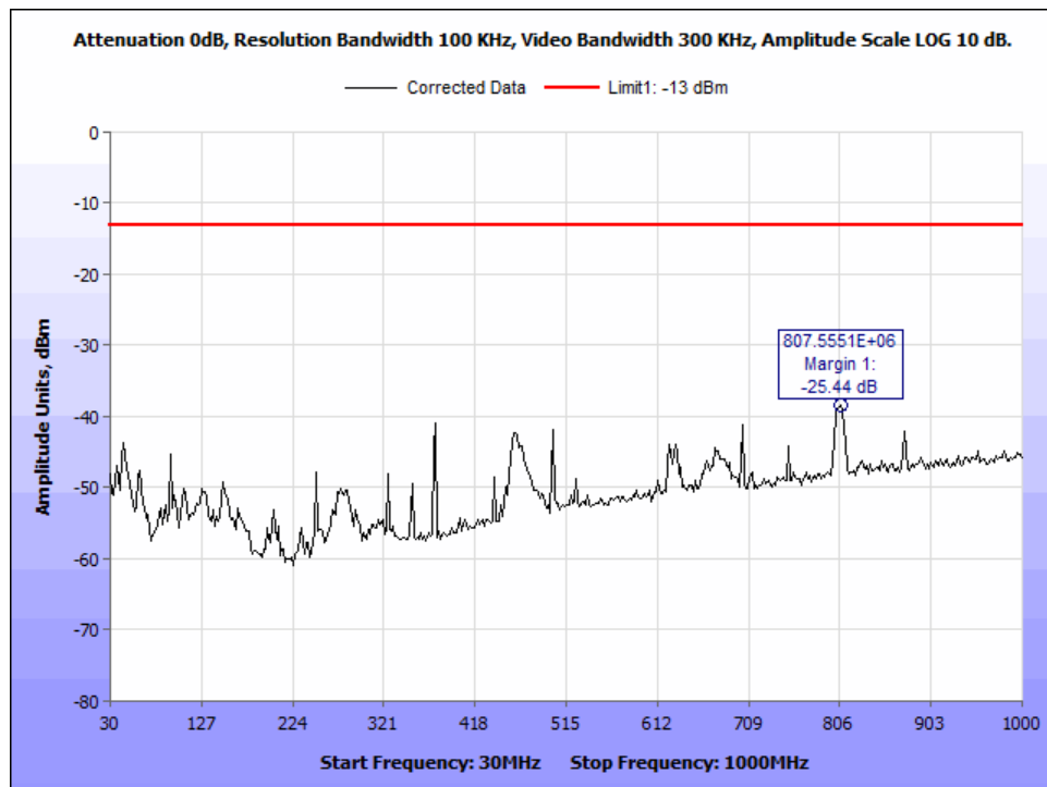
Figure 163: §25.202(f) Radiated Spurious Emissions, MissionLINK 200, Ch1_83.334kHz BW_30-1000MHz.
