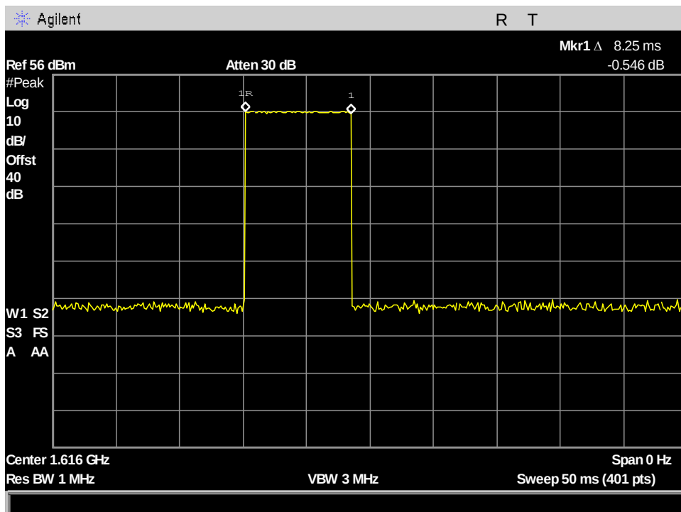
Figure 46: §25.204(a) Conducted RF Output Power, 666.666kHz_Ton
