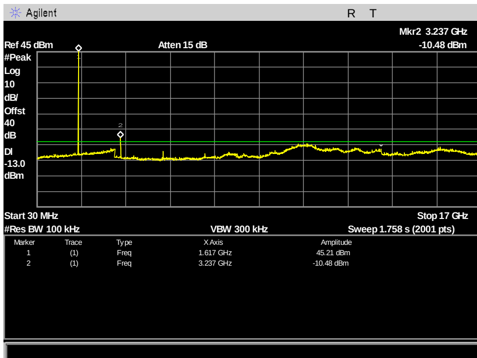
Figure 120: §25.202(f) MissionLINK Spurious Emissions at Antenna Terminals, ch1_83.334kHz_30MHz - 17GHz
