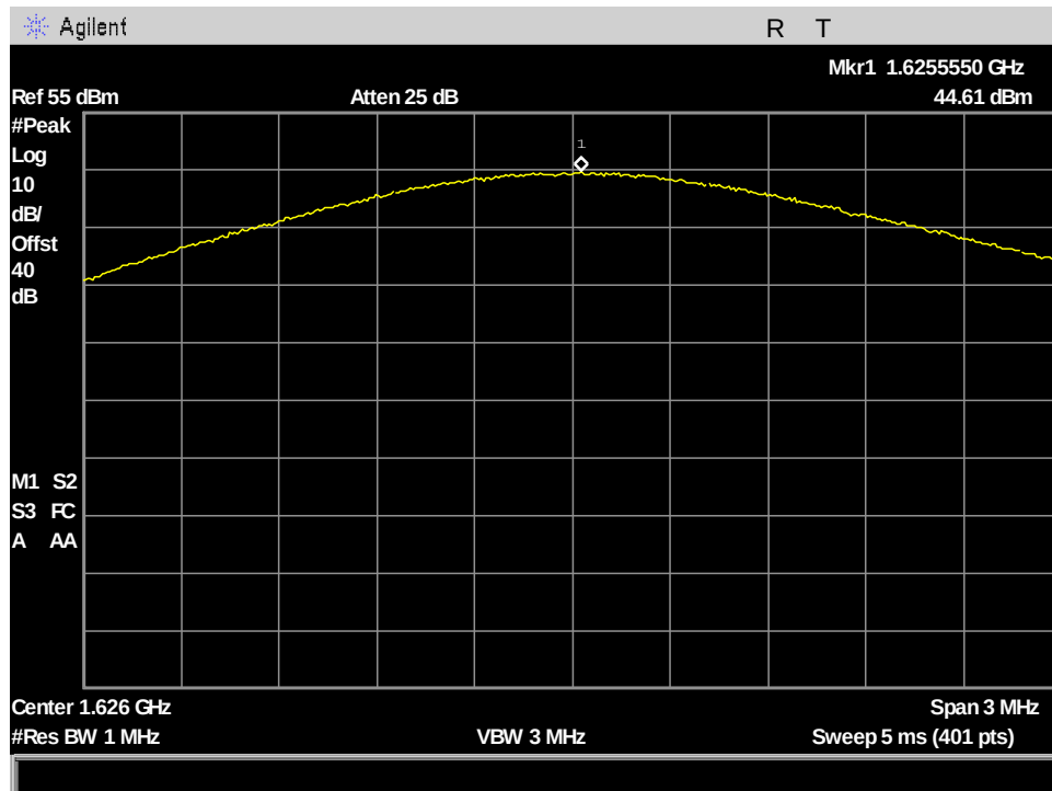
Figure 69: §25.204(a) Conducted RF Output Power, MissionLINK PK_Output Power_ch232_333.333kHz BW
