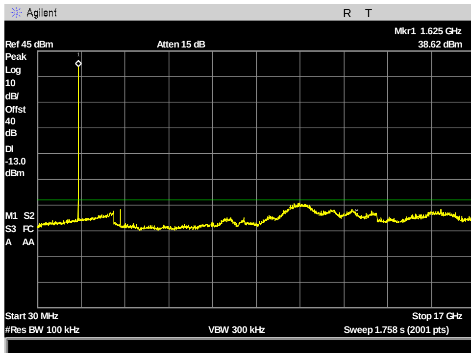
Figure 130: §25.202(f) VesseLINK Spurious Emissions at Antenna Terminals, ch121_666.666kHz_30MHz - 17GHz
