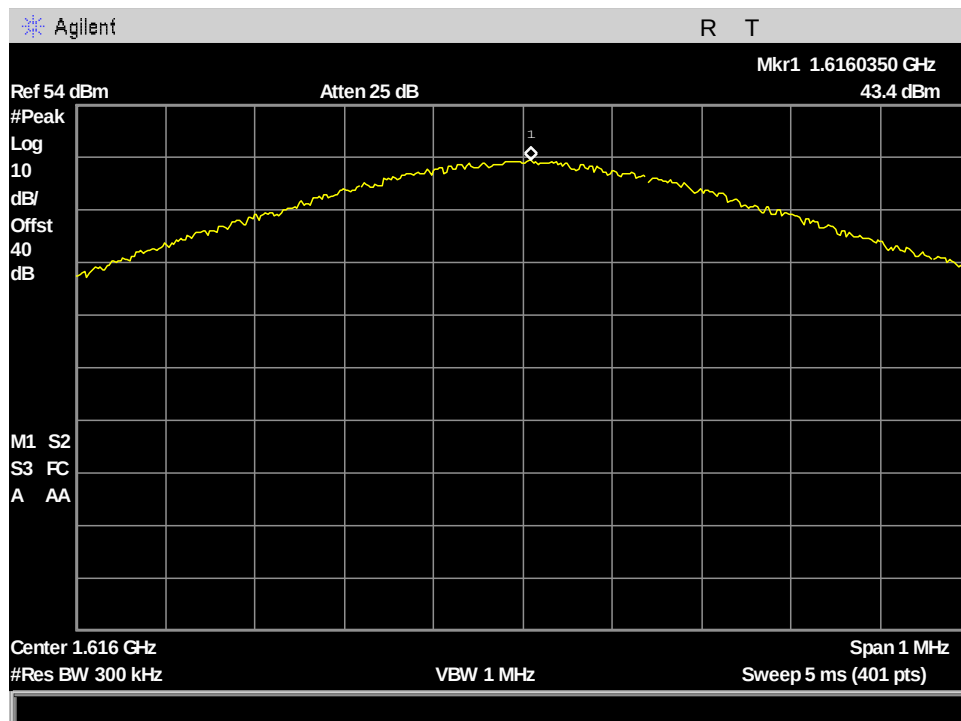
Figure 90: §25.204(a) Conducted RF Output Power, VesseLINK PK_Output Power_ch1_41.668kHz BW
