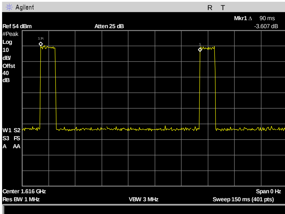
Figure 47: §25.204(a) Conducted RF Output Power, 83.334kHz_Period
