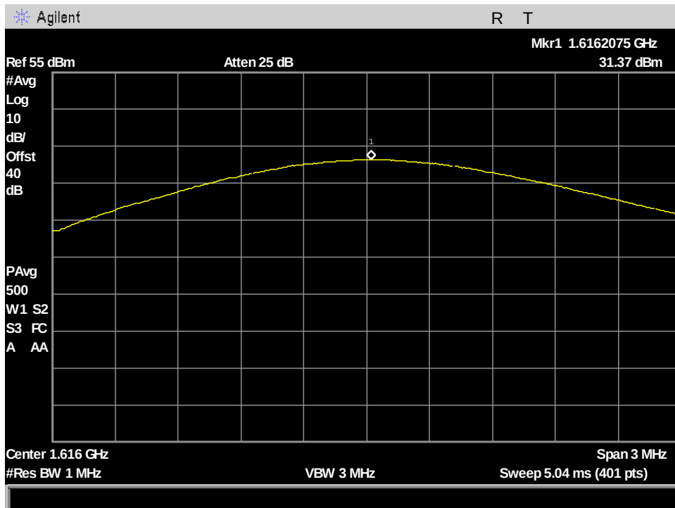
Figure 77: §25.204(a) Conducted RF Output Power, VesseLINK AVG_Output Power_ch1_333.333kHz BW
