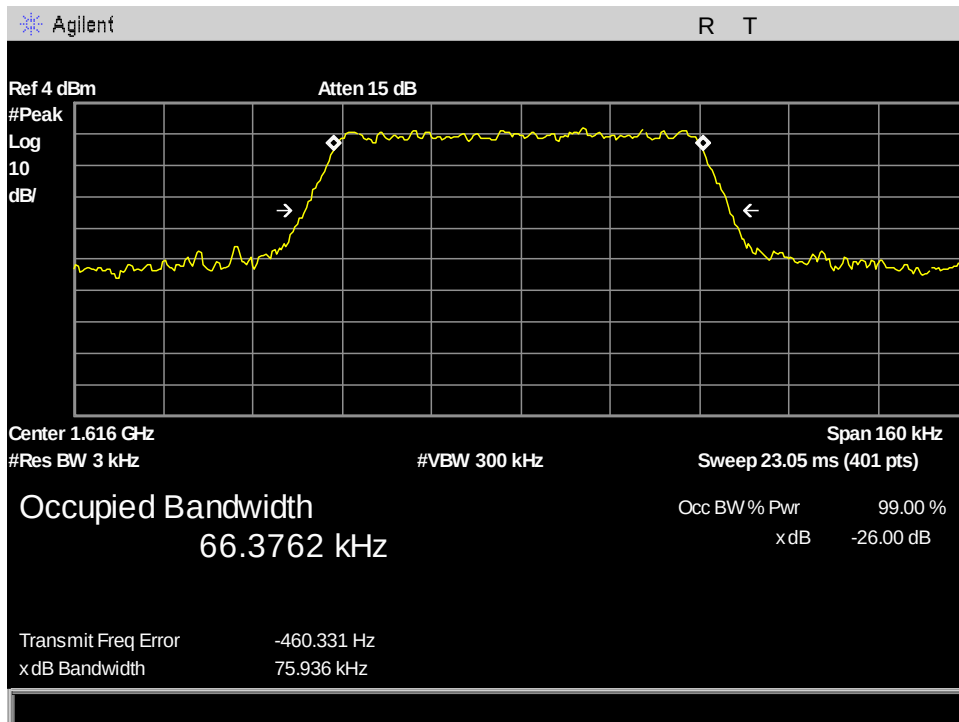
Figure 104: §2.1049(b) Occupied Bandwidth, Ch1_OBW_83.334kHz
