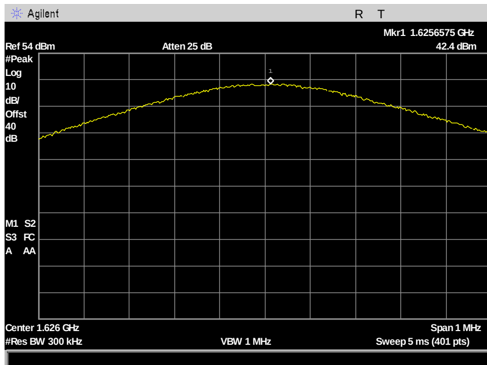
Figure 70: §25.204(a) Conducted RF Output Power, MissionLINK PK_Output Power_ch232_41.668kHz BW
