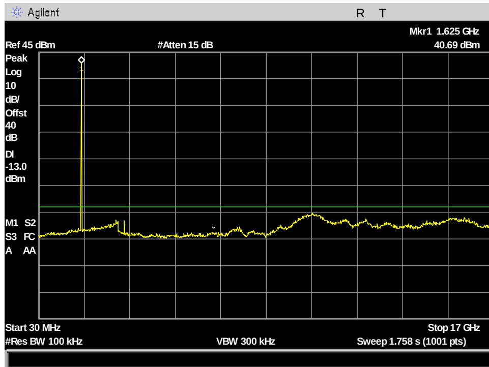
Figure 129: §25.202(f) VesseLINK Spurious Emissions at Antenna Terminals, ch121_41.668kHz_30MHz - 17GHz
