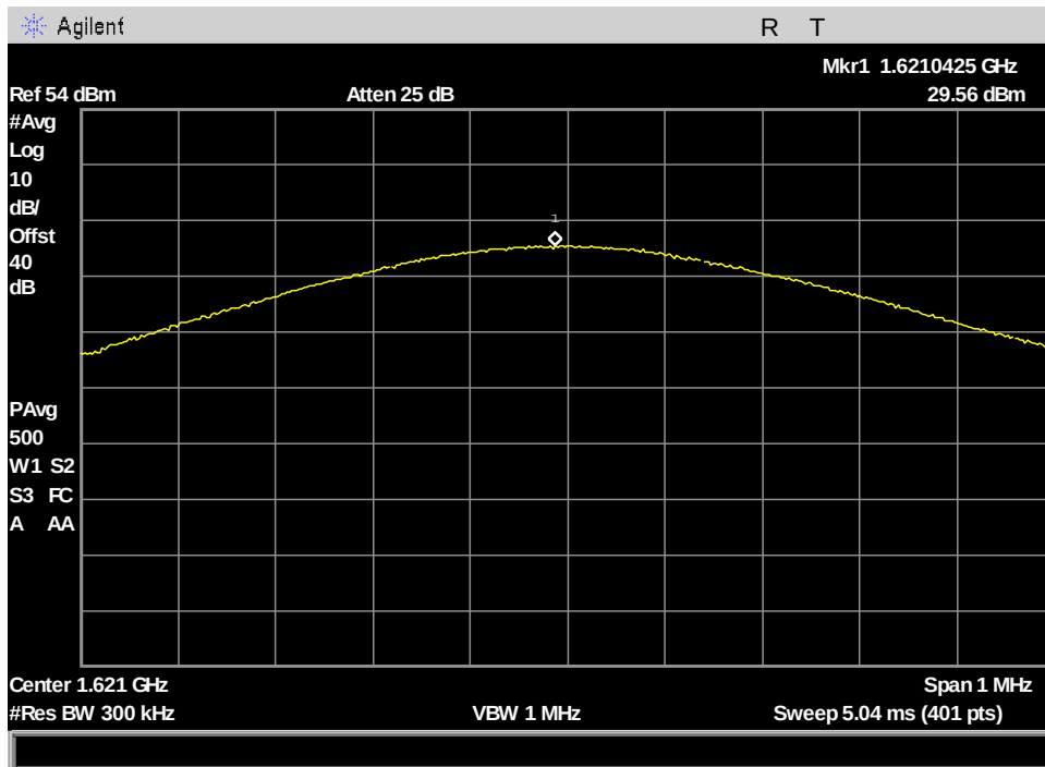
Figure 52: §25.204(a) Conducted RF Output Power, MissionLINK AVG_Output Power_ch121_83.334kHz BW
