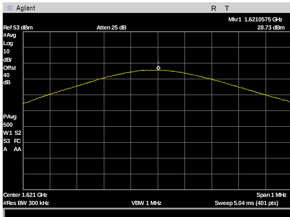
Figure 76: §25.204(a) Conducted RF Output Power, VesseLINK AVG_Output Power_ch121_83.334kHz BW
