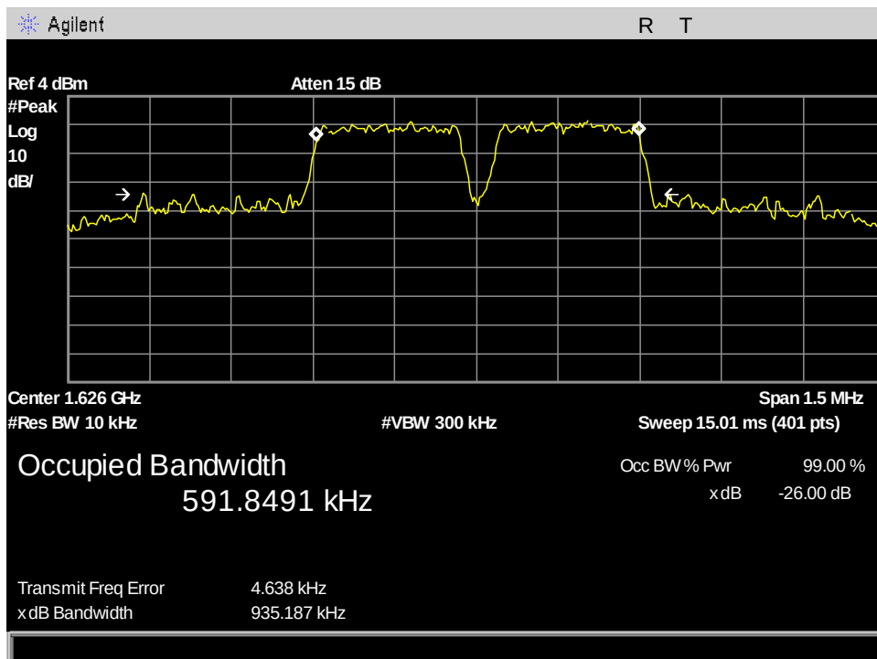
Figure 107: §2.1049(b) Occupied Bandwidth, Ch232_OBW_666.666kHz
