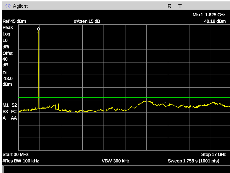
Figure 135: §25.202(f) VesseLINK Spurious Emissions at Antenna Terminals, ch1_83.334kHz_30MHz - 17GHz
