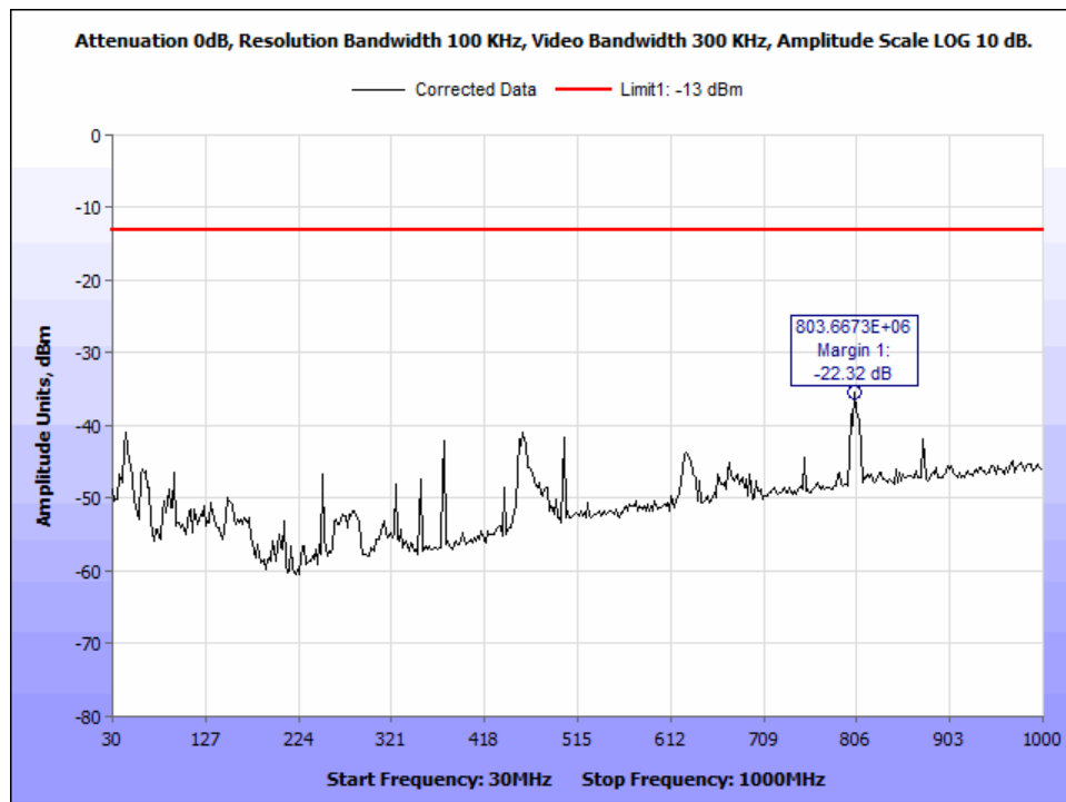
Figure 151: §25.202(f) Radiated Spurious Emissions, MissionLINK 200, Ch121_41.668kHz BW_30-1000MHz.
