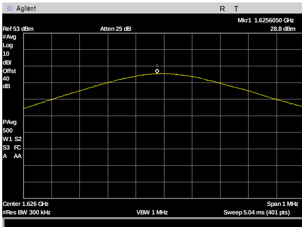
Figure 84: §25.204(a) Conducted RF Output Power, VesseLINK AVG_Output Power_ch232_83.334kHz BW
