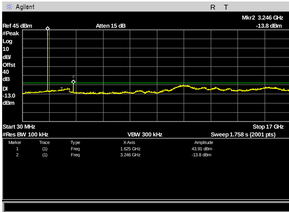
Figure 109: §25.202(f) MissionLINK Spurious Emissions at Antenna Terminals, ch121_333.333kHz_30MHz - 17GHz
