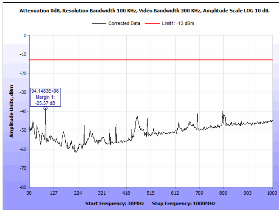
Figure 149: §25.202(f) Radiated Spurious Emissions, MissionLINK 200, Ch121_333.333kHz BW_30-1000MHz.
