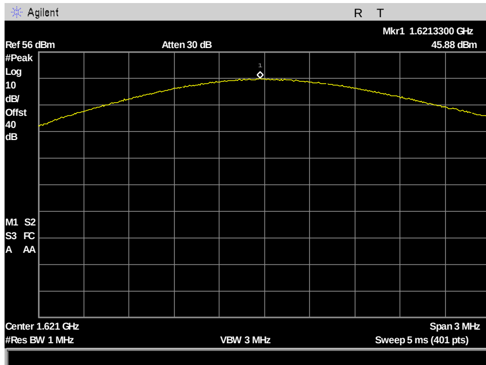
Figure 87: §25.204(a) Conducted RF Output Power, VesseLINK PK_Output Power_ch121_666.666kHz BW
