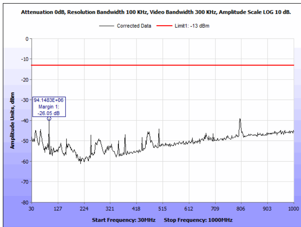
Figure 157: §25.202(f) Radiated Spurious Emissions, MissionLINK 200, Ch1_333.333kHz BW_30-1000MHz.
