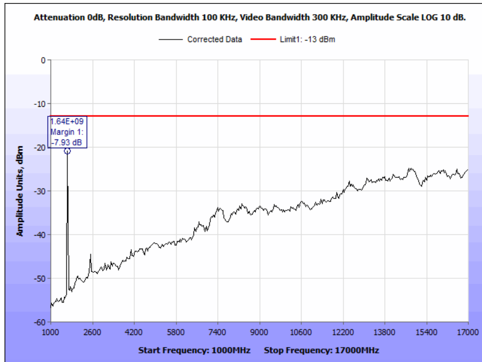
Figure 164: §25.202(f) Radiated Spurious Emissions, MissionLINK 200, Ch232_333.333kHz BW_1-17 GHz.
