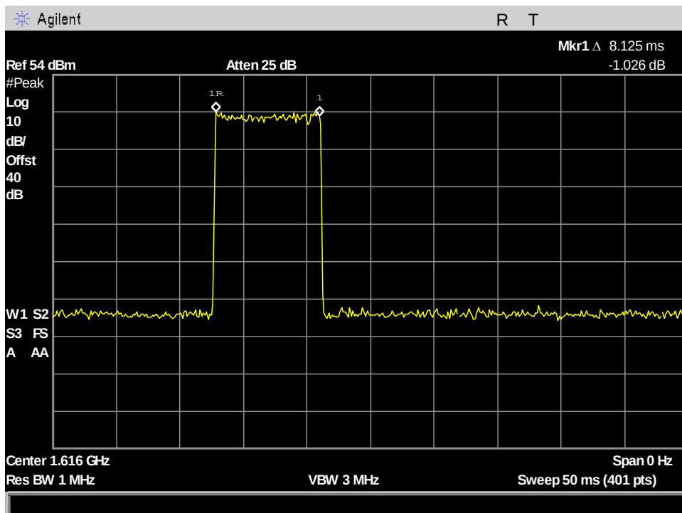
Figure 48: §25.204(a) Conducted RF Output Power, 83.334kHz_Ton
