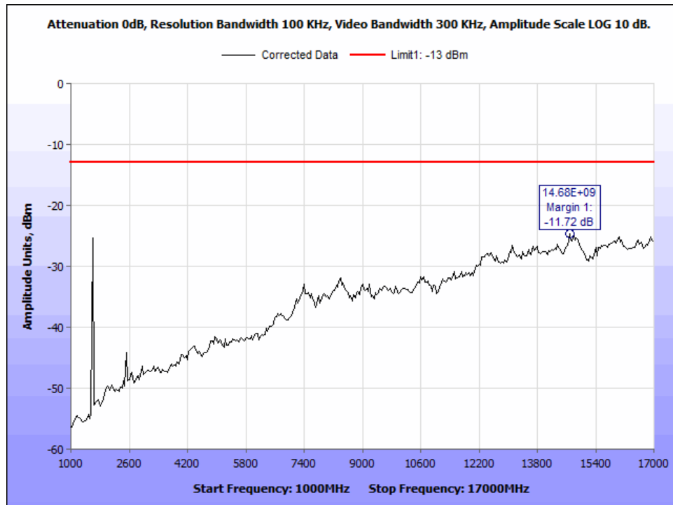
Figure 162: §25.202(f) Radiated Spurious Emissions, MissionLINK 200, Ch1_83.334kHz BW_1-17 GHz.
