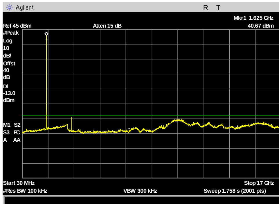
Figure 112: §25.202(f) MissionLINK Spurious Emissions at Antenna Terminals, ch121_666.666kHz_30MHz - 17GHz
