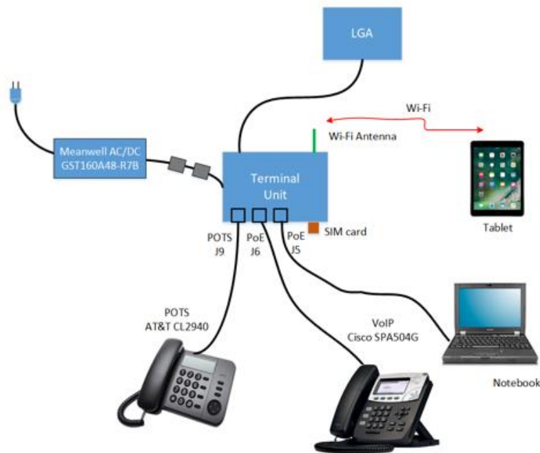
Figure 5: Block Diagram of Test Configuration, MissionLINK 200
