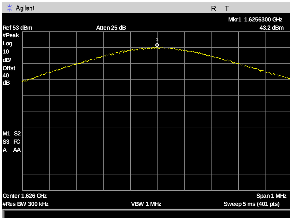
Figure 96: §25.204(a) Conducted RF Output Power, VesseLINK PK_Output Power_ch232_83.334kHz BW
