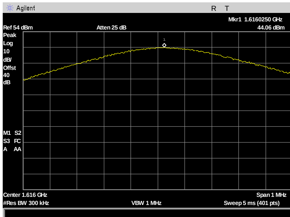
Figure 66: §25.204(a) Conducted RF Output Power, MissionLINK PK_Output Power_ch1_41.668kHz BW
