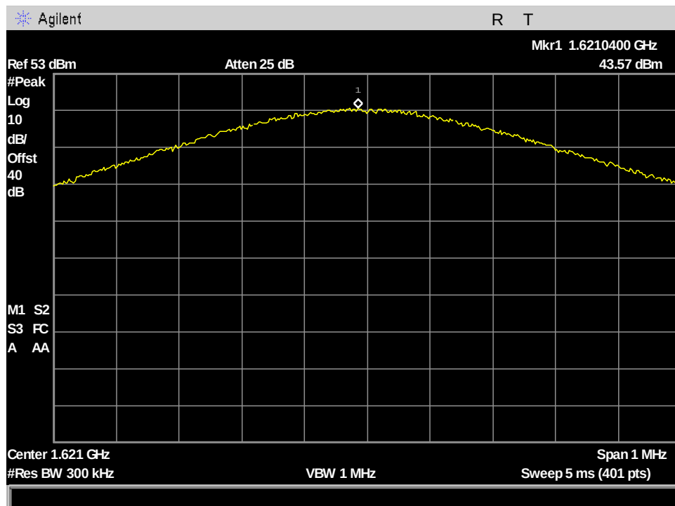
Figure 88: §25.204(a) Conducted RF Output Power, VesseLINK PK_Output Power_ch121_83.334kHz BW
