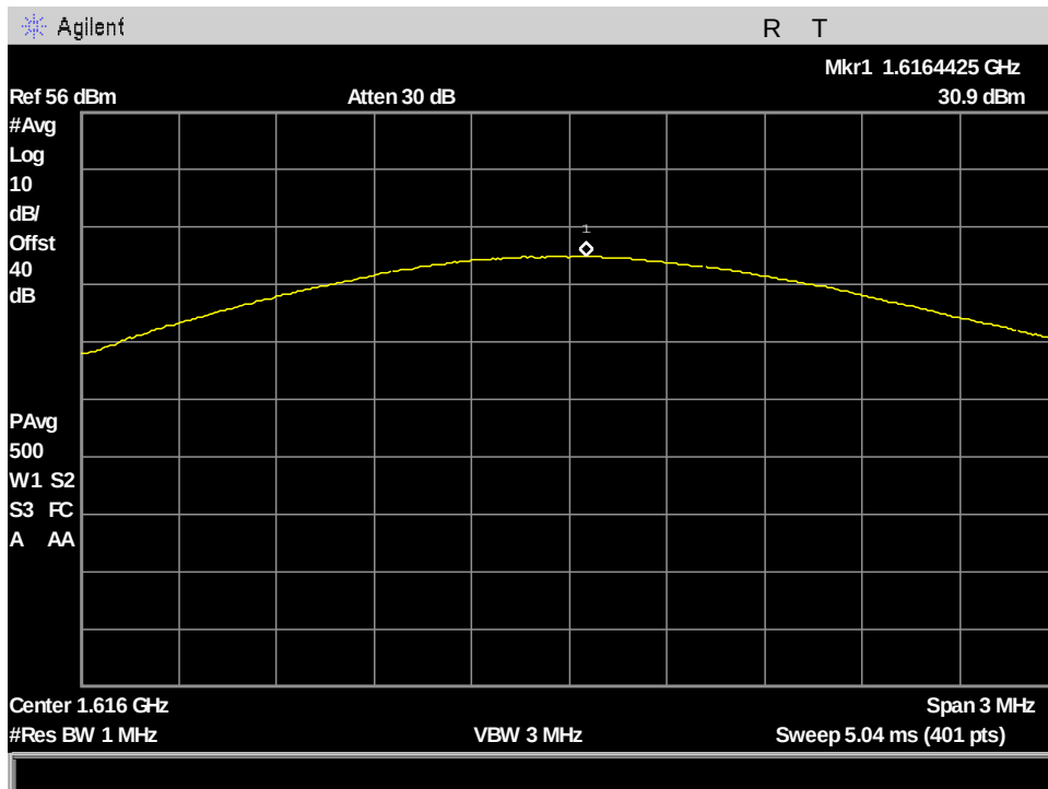
Figure 79: §25.204(a) Conducted RF Output Power, VesseLINK AVG_Output Power_ch1_666.666kHz BW
