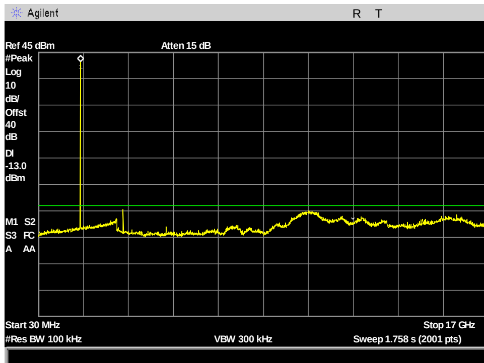
Figure 118: §25.202(f) MissionLINK Spurious Emissions at Antenna Terminals, ch1_666.666kHz_30MHz - 17GHz
