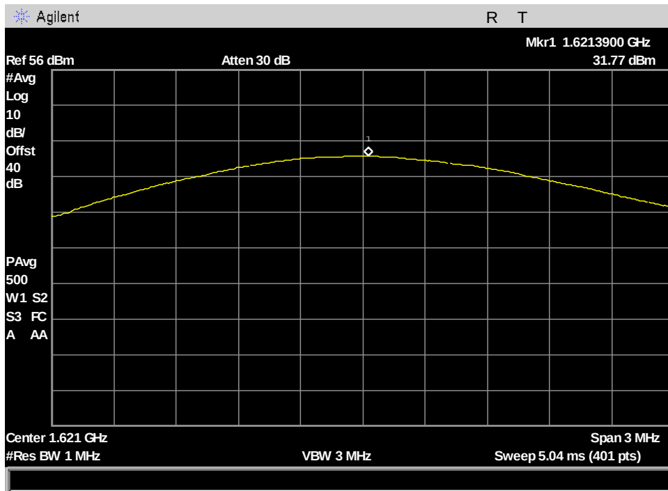
Figure 51: §25.204(a) Conducted RF Output Power, MissionLINK AVG_Output Power_ch121_666.666kHz BW
