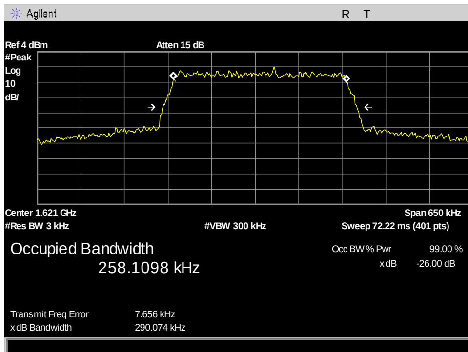
Figure 97: §2.1049(b) Occupied Bandwidth, Ch121_OBW_333.333kHz
