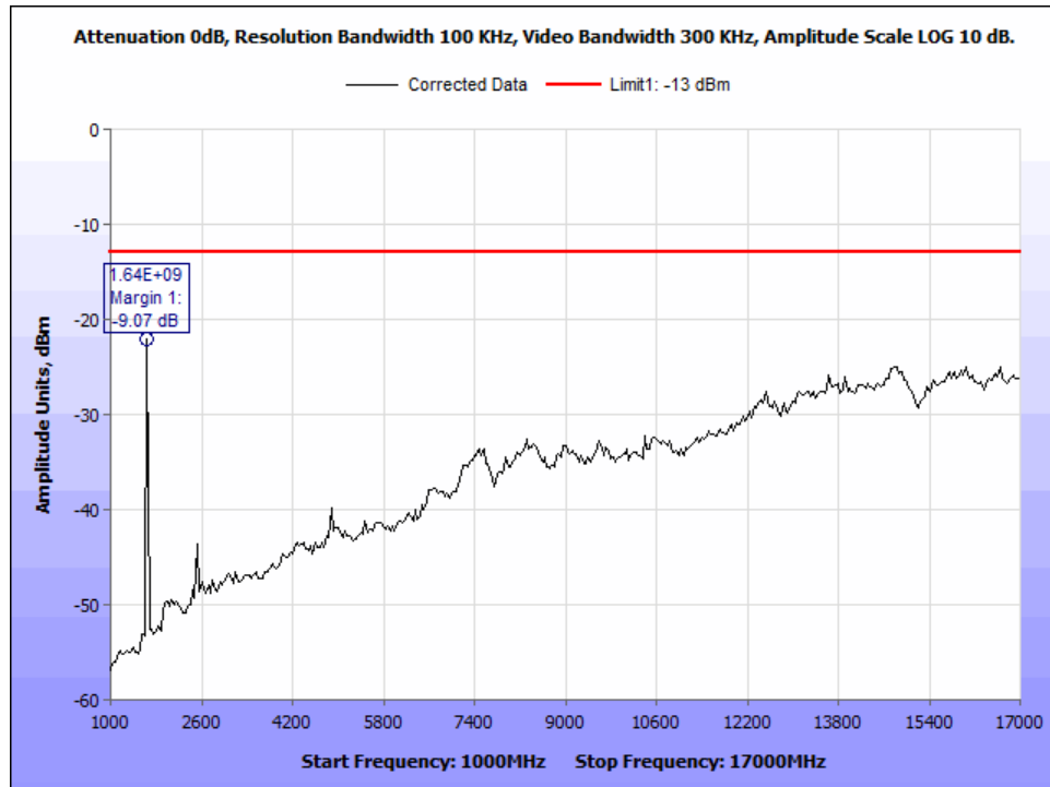
Figure 148: §25.202(f) Radiated Spurious Emissions, MissionLINK 200, Ch121_333.333kHz BW_1-17 GHz.
