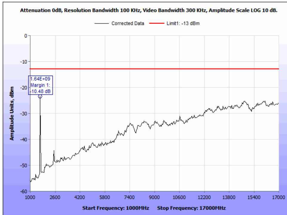
Figure 166: §25.202(f) Radiated Spurious Emissions, MissionLINK 200, Ch232_41.668kHz BW_1-17 GHz.
