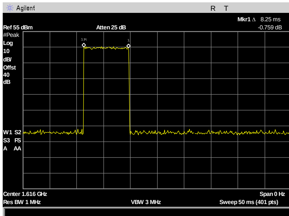
Figure 42: §25.204(a) Conducted RF Output Power, 333.333kHz_Ton
