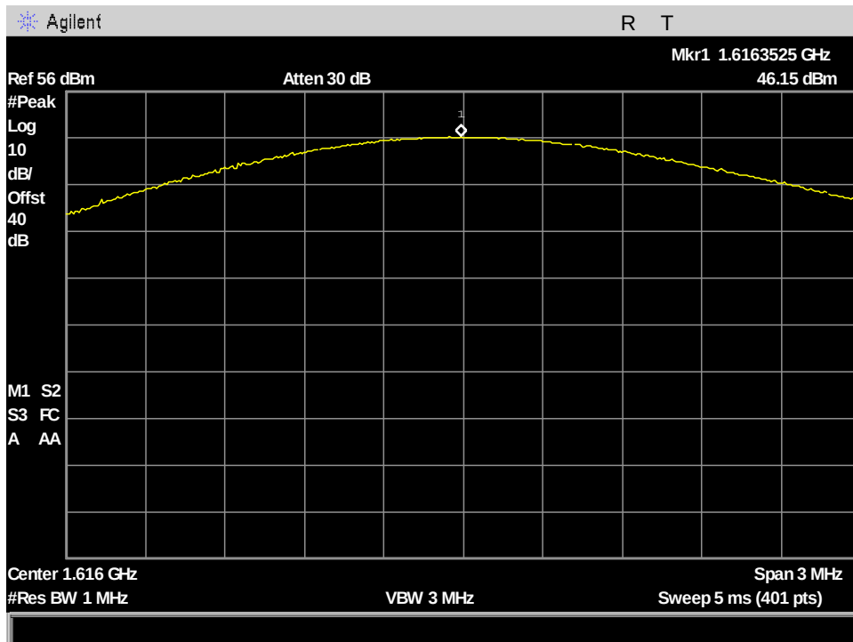
Figure 67: §25.204(a) Conducted RF Output Power, MissionLINK PK_Output Power_ch1_666.666kHz BW
