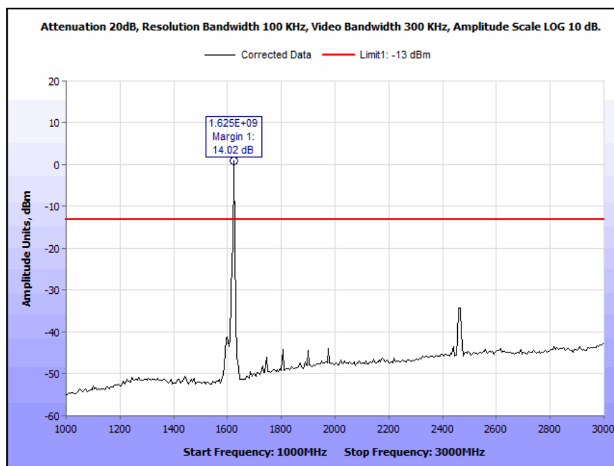
Plot 33. Radiated Spurious Emissions, L423, Channel 232, 1625.666 MHz, 1 GHz – 3 GHz
