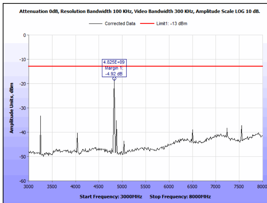
Plot 34. Radiated Spurious Emissions, L423, Channel 232, 1625.666 MHz, 3 GHz – 8 GHz
