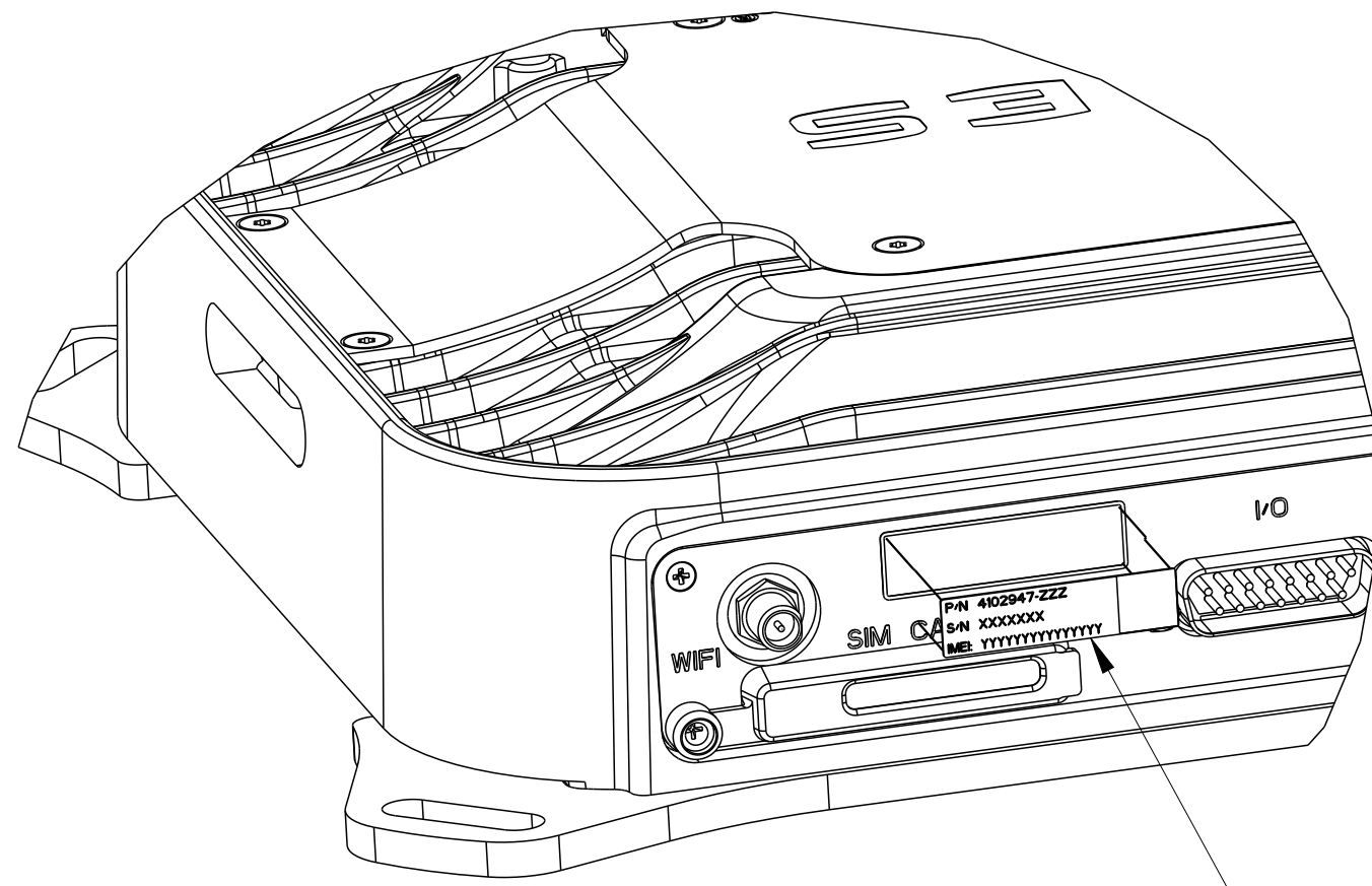
LABEL DETAIL A ALL VARIANTS
