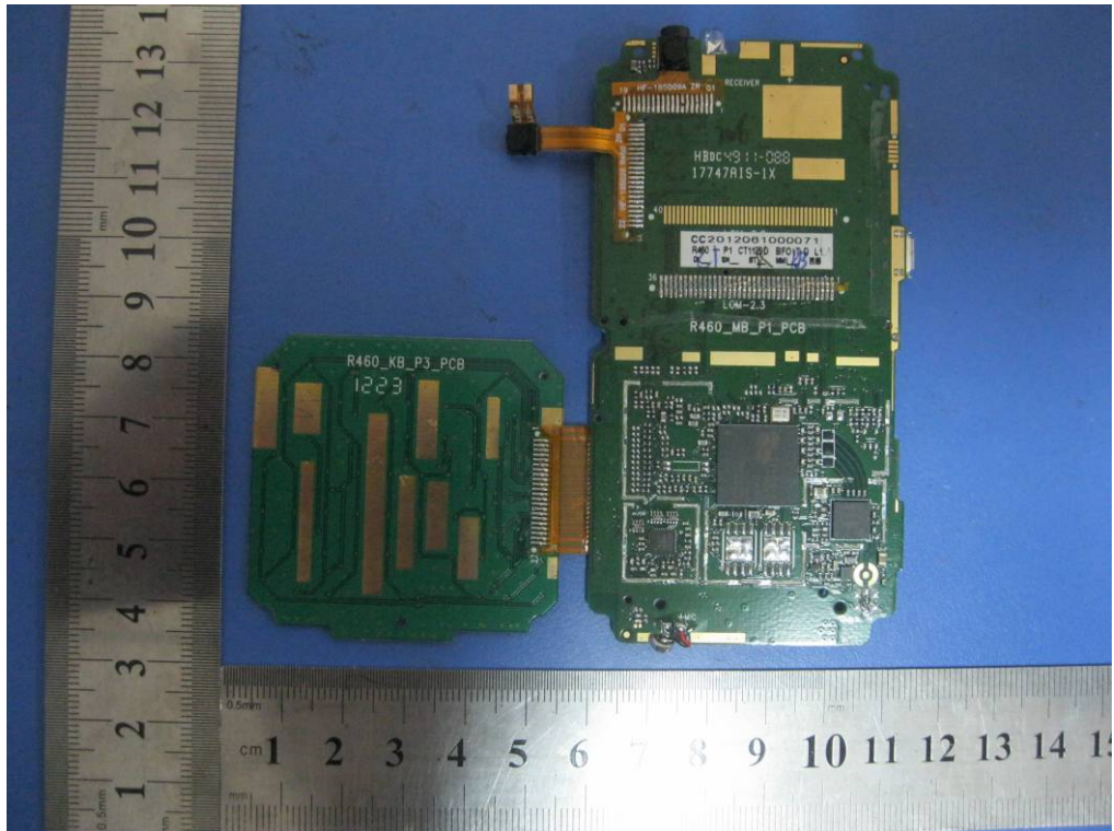
Uncover without LCD - Top View
