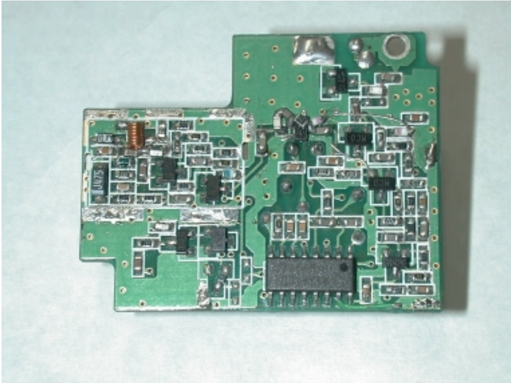
PCB WX Component Side
