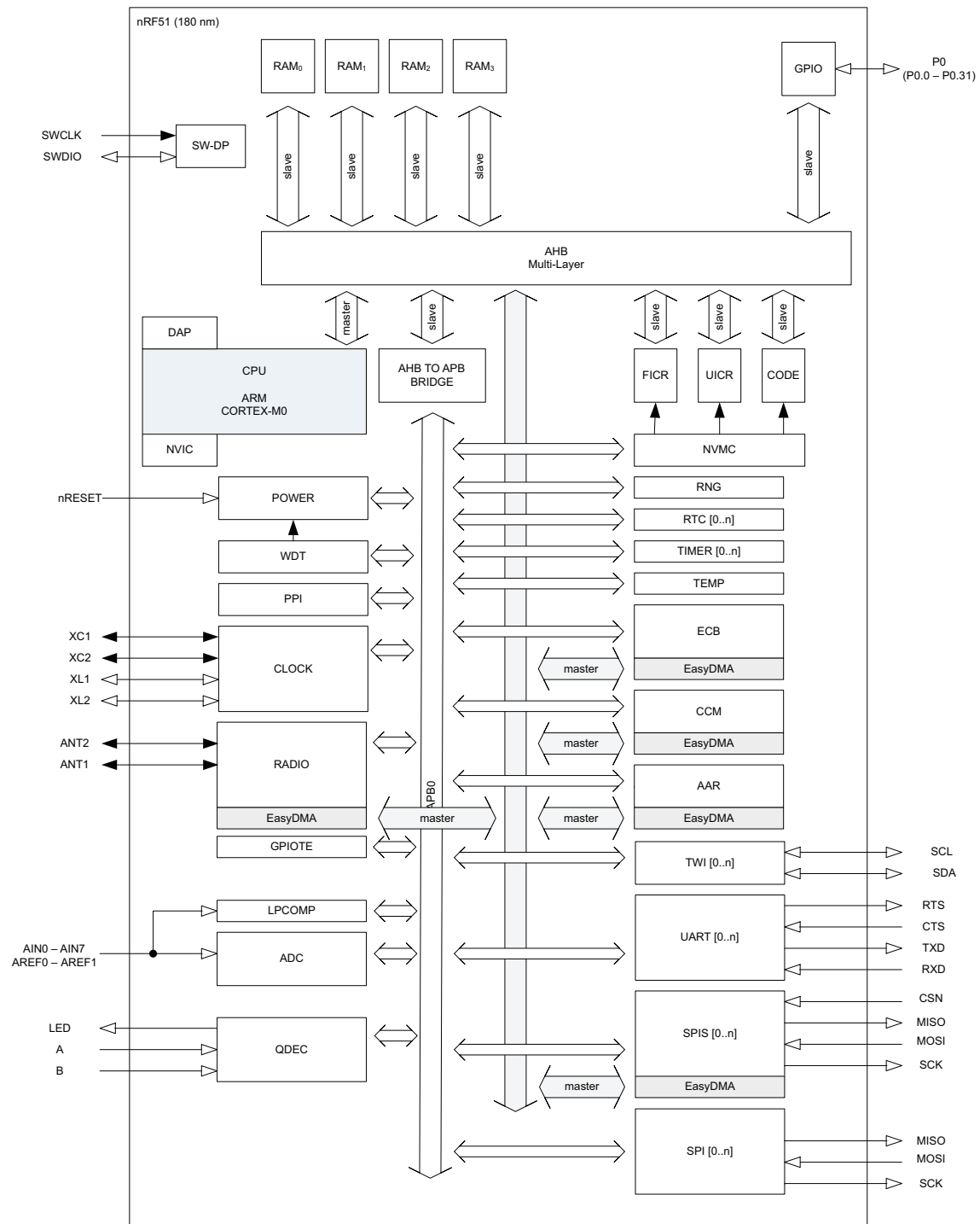
Figure 1 Block diagram
