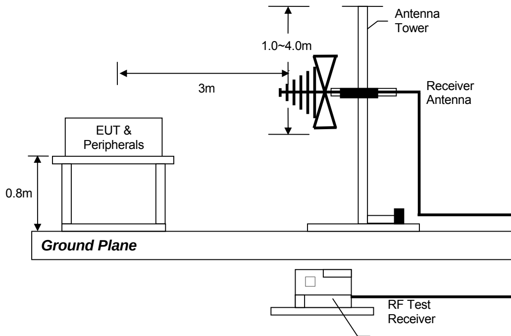
Test setup of radiated emissions upto 1GHz
