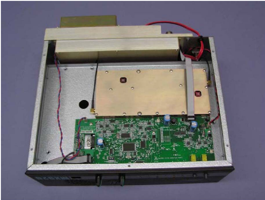
EUT – PCB View Complete in Chassis
