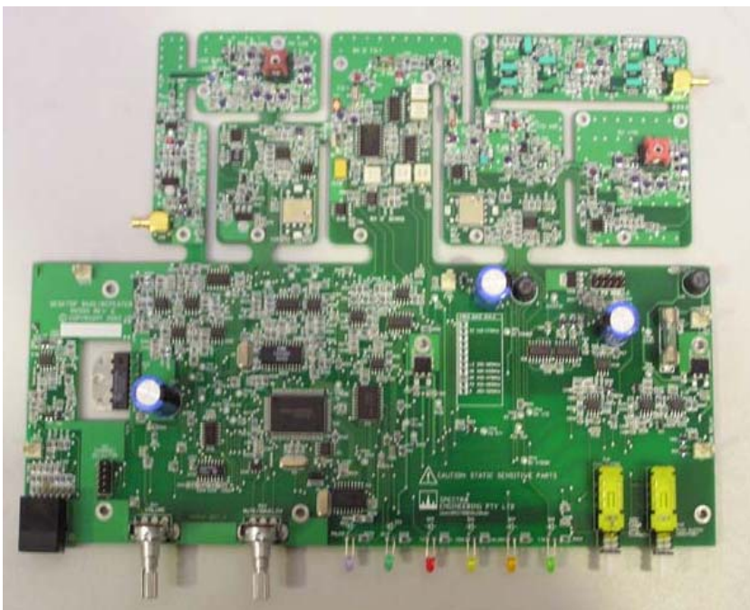
EUT – PCB Top View
