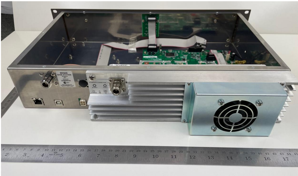
Figure 5. External Rear View.
