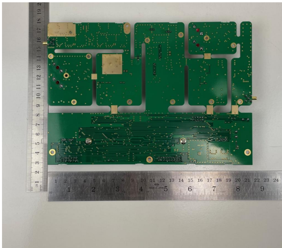
Figure 12. Main RF controller PCB - Bottom View.
