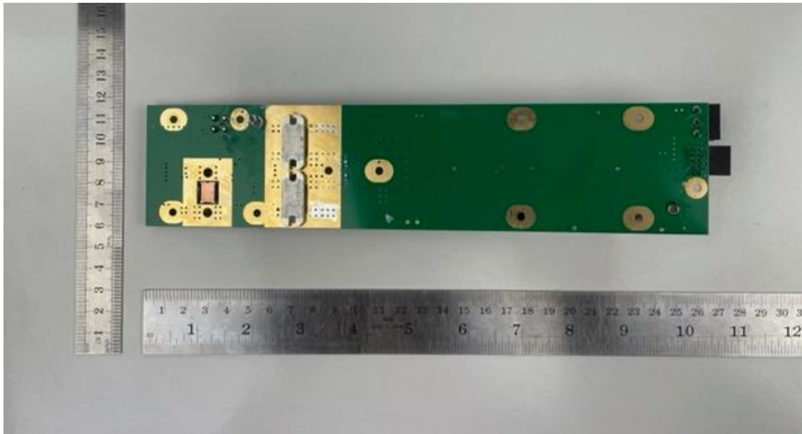
Figure 16. PA PCB Bottom View.
