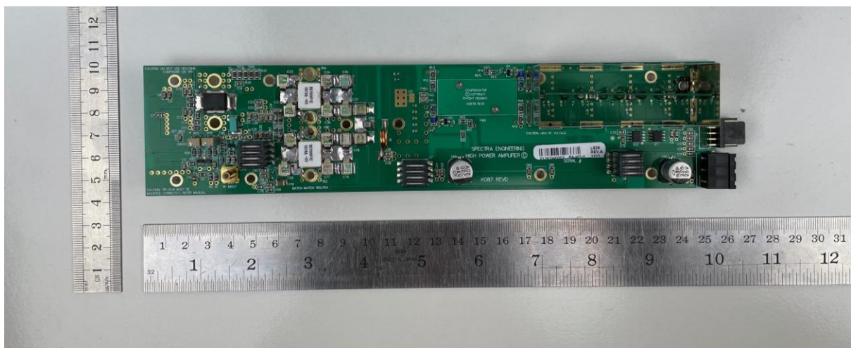
Figure 15. PA PCB Top View.
