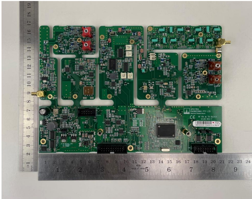
Figure 11. Main RF controller PCB Top View.
