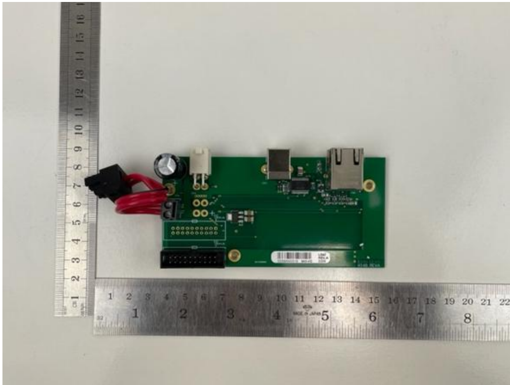
Figure 13. Rear Interface -PCB Top View.
