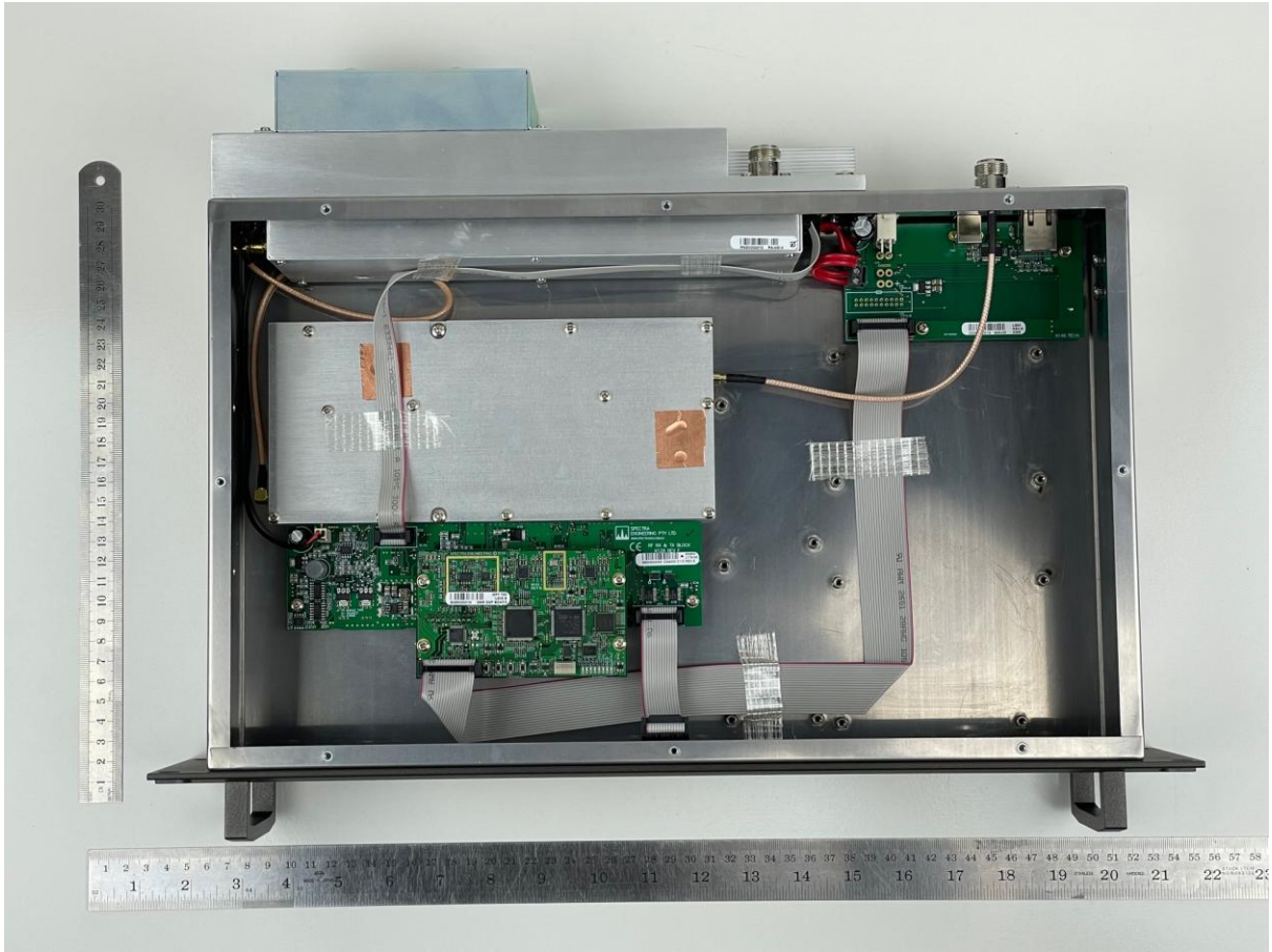
Figure 8. External Chassis Top View Lid off.
