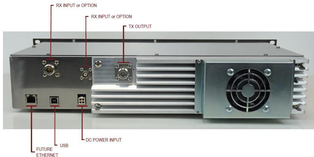
Figure 1-2 MX940 Rear Panel. (RF Connecting cables not shown)
