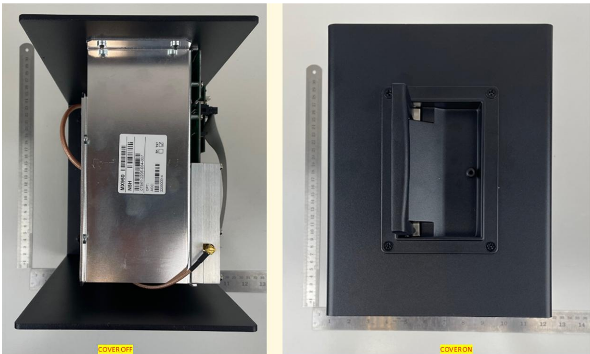
Figure 4. External Chassis Top Views.
