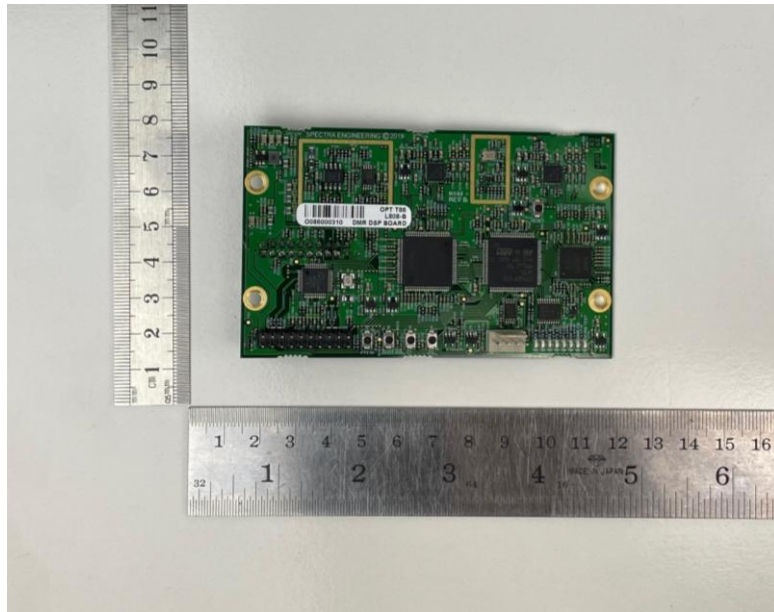
Figure 14. Logic Board Top View.
