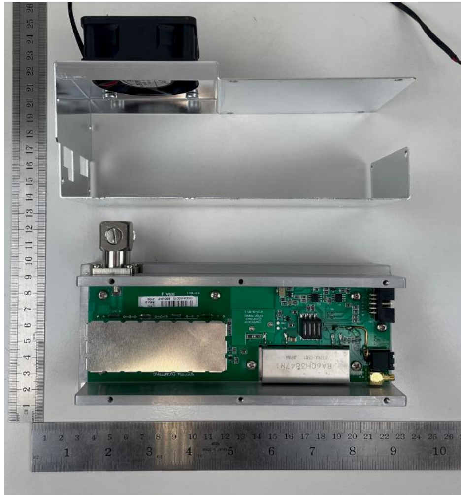
Figure 12. PA Top View.
