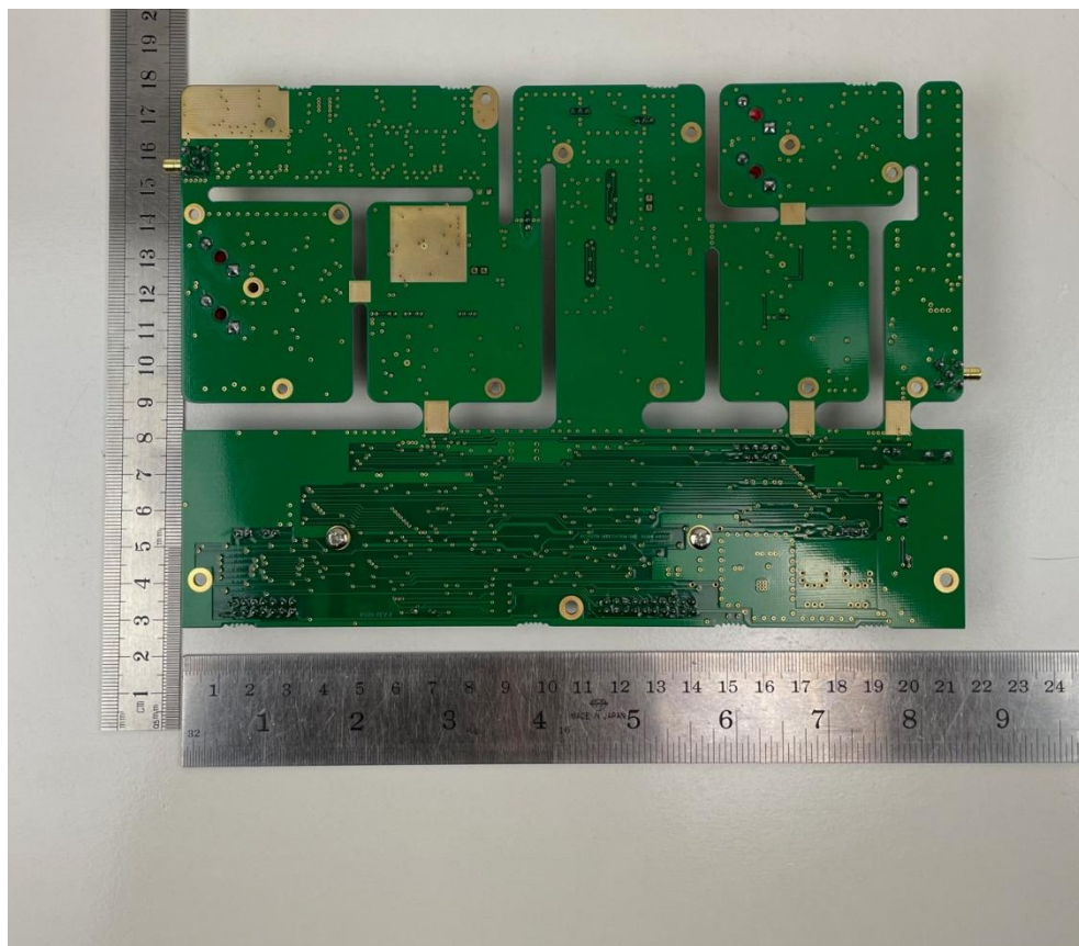
Figure 9. Main RF controller PCB - Bottom View.
