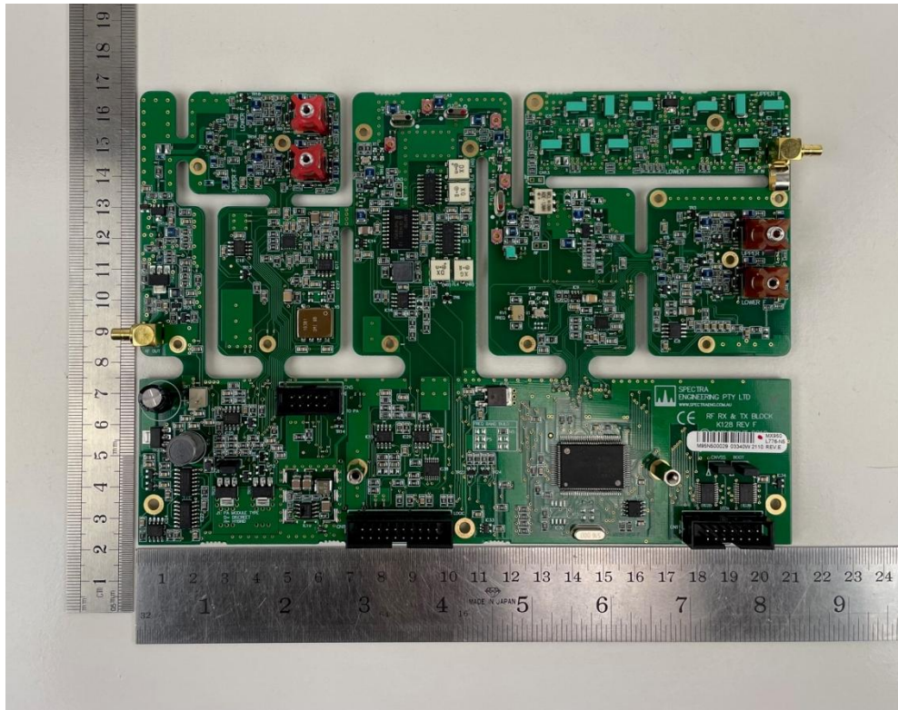
Figure 8. Main RF controller PCB Top View.
