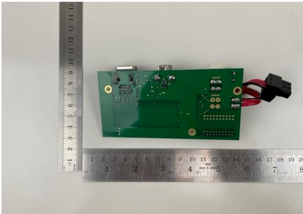
Figure 11. Rear Interface PCB - Bottom View.
