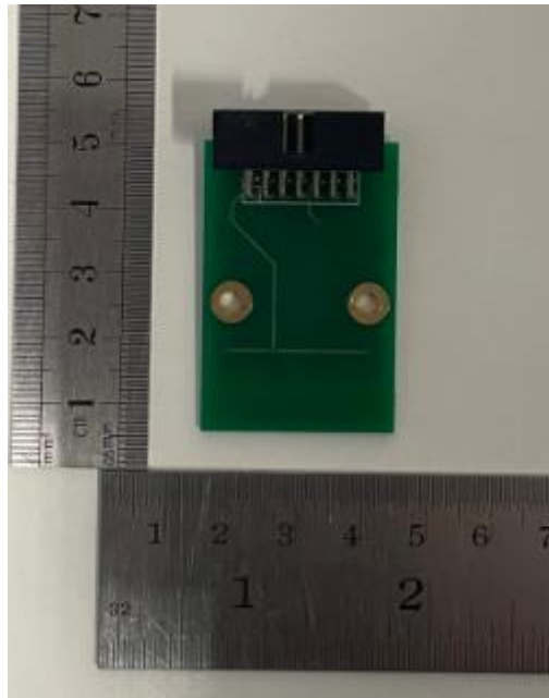
Figure 6. Controller Led PCB Top View.
