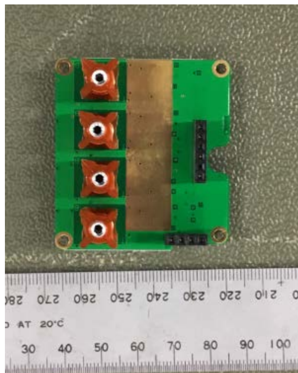
Figure 12. Receiver VCO PCB Bottom View.
