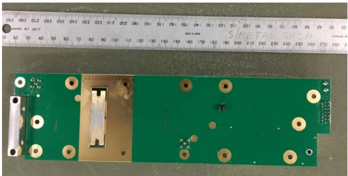
Figure 21. PA PCB Bottom View.
