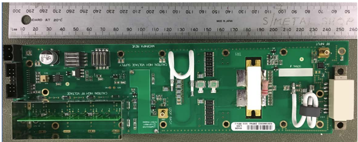
Figure 20. PA PCB Top View.
