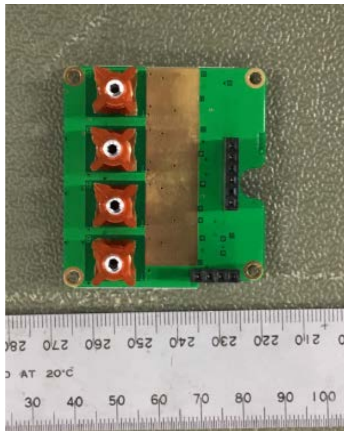
Figure 19. Exciter VCO PCB Bottom View.
