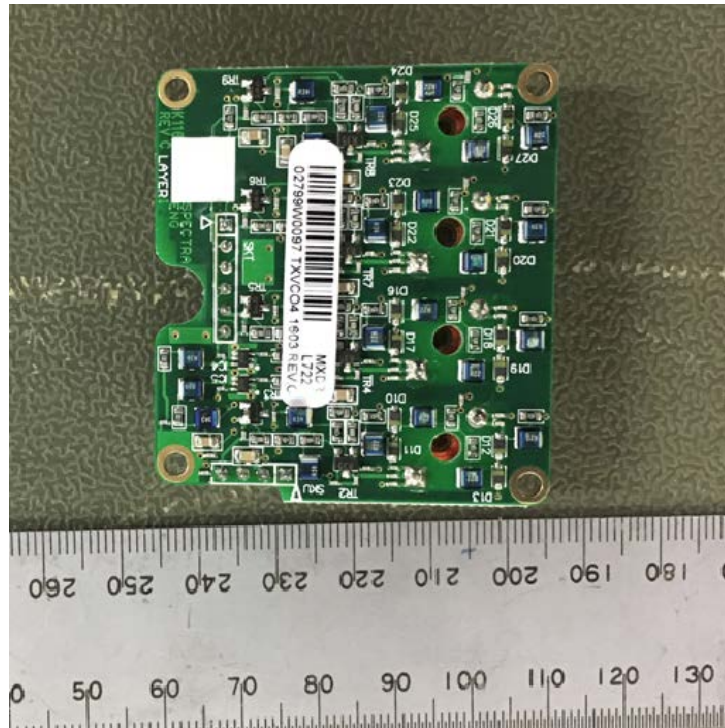
Figure 18. Exciter VCO PCB Top View.
