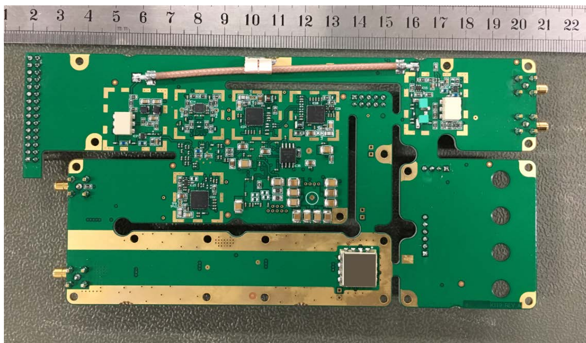
Figure 17. Exciter PCB Bottom View- No shield covers.
