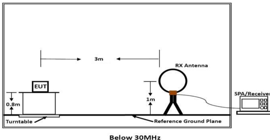
Below 30MHz
