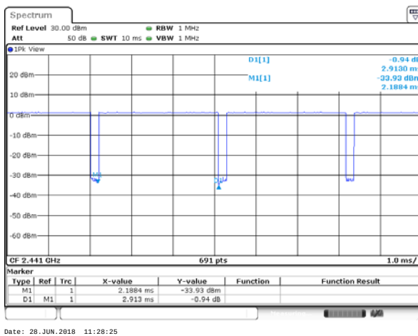
Package Transfer Time Plot CH39-DH5
