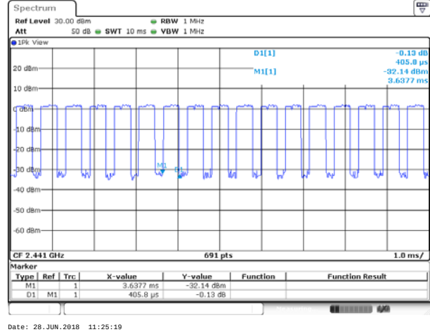
Package Transfer Time Plot CH39-2DH3
