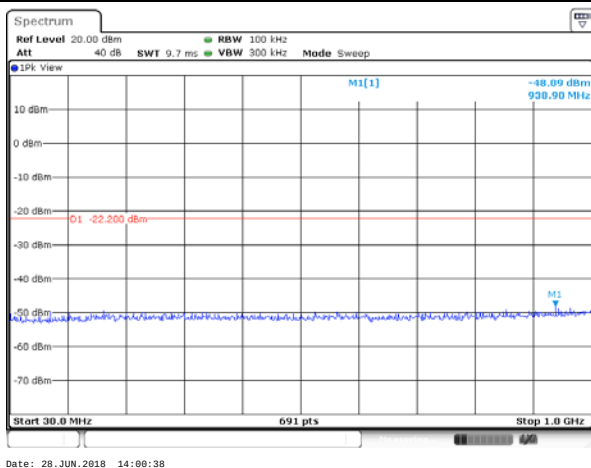
8-DPSK on channel 00
