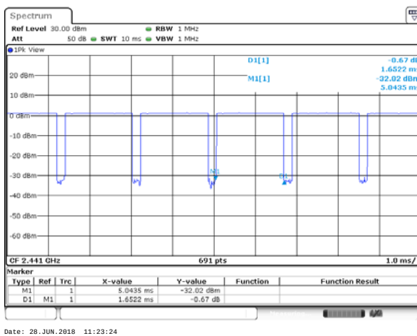
Package Transfer Time Plot CH39-DH3
