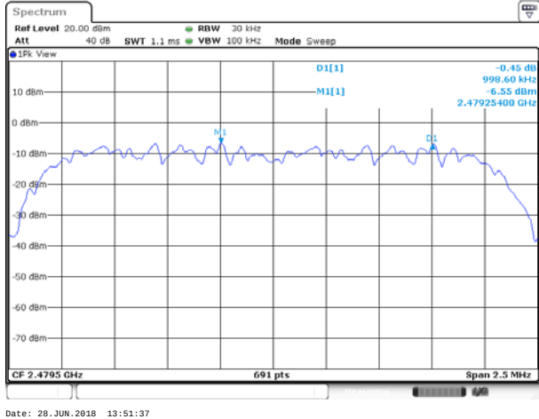
(2Mbps) Channel Separation plot on channel 77-78
