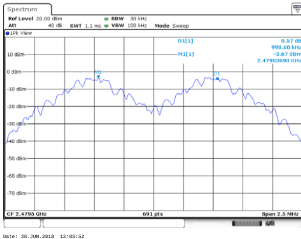
(1Mbps) Channel Separation plot on channel 77-78
