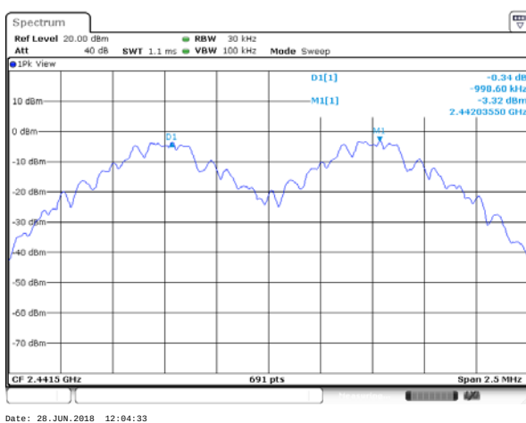
(1Mbps) Channel Separation plot on channel 39-40
