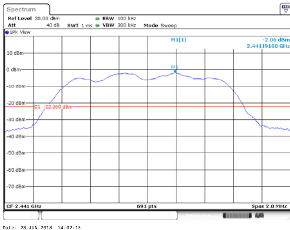
8-DPSK on channel 39
