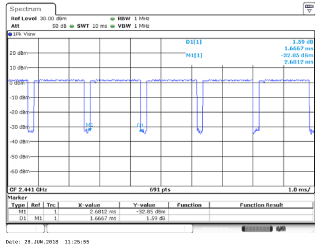
Package Transfer Time Plot CH39-2DH5
