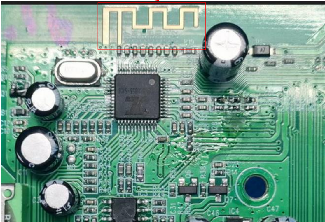
BT antenna
