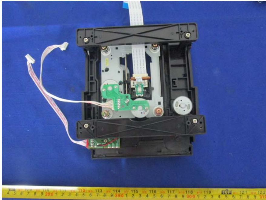
EUT – CD Module Top View
