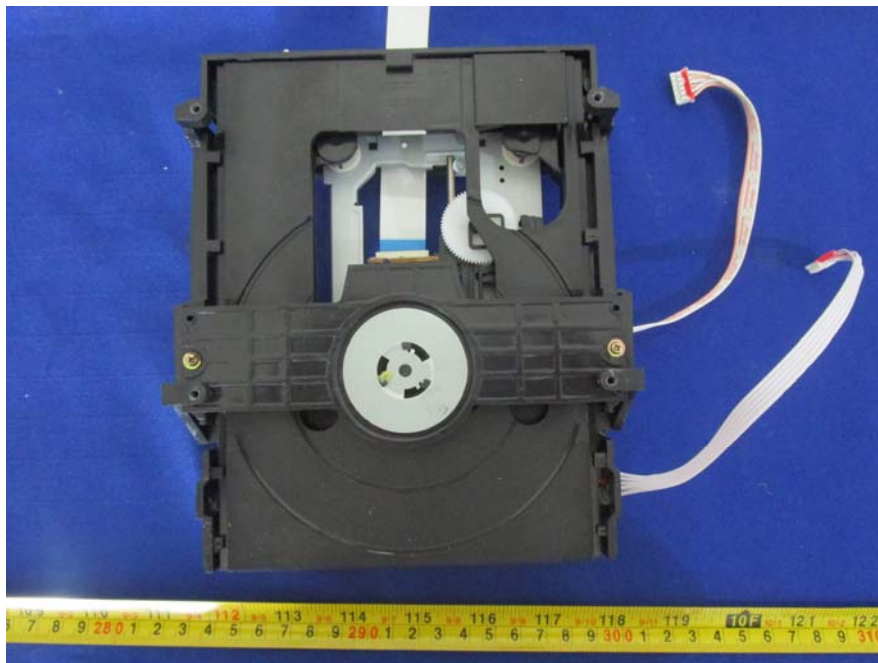
EUT – CD Module Bottom View
