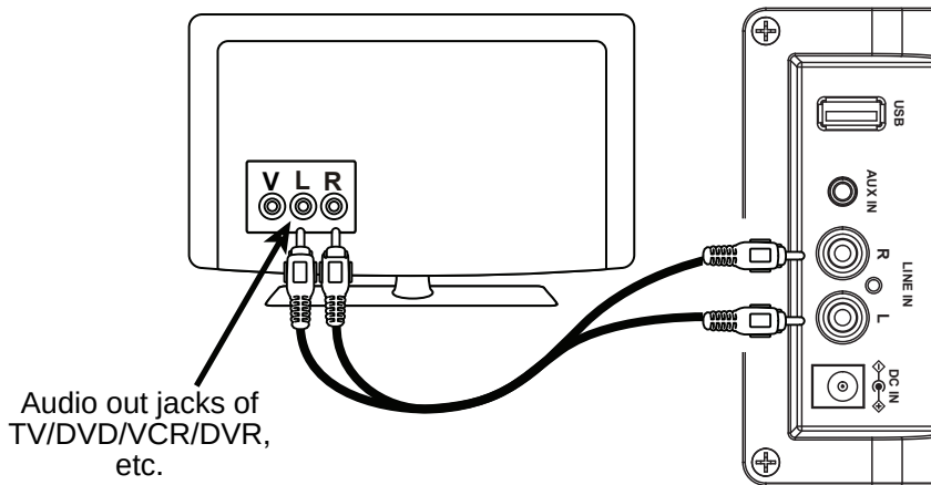
Rear view of the unit
