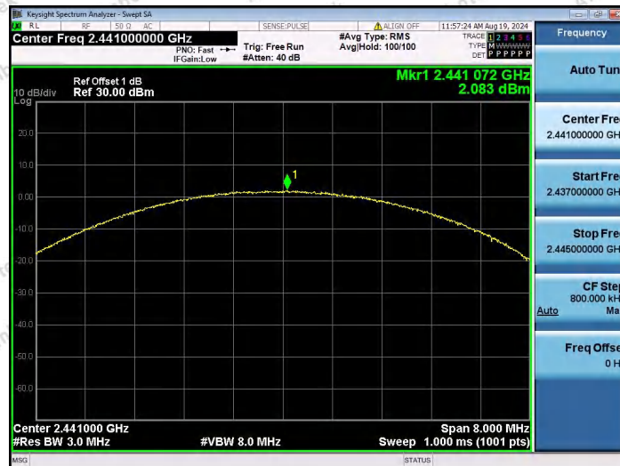
2DH5-Ant1-2441-PASS
