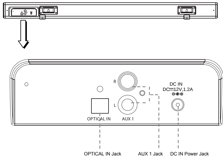
CONTROL PANEL
