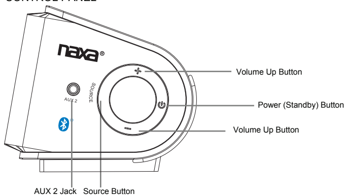
CONTROL PANEL
