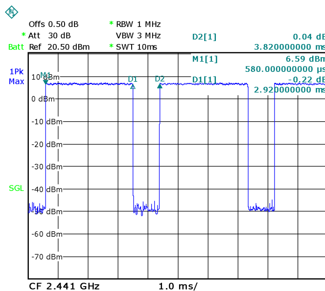
Middle Channel
