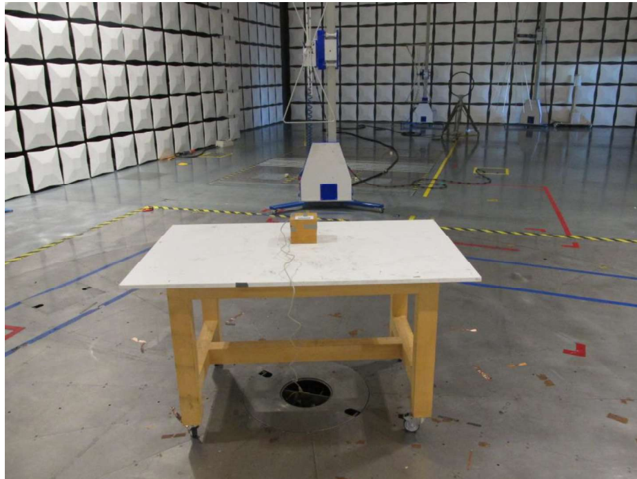
Figure 12 - Test setup for radiated emission
