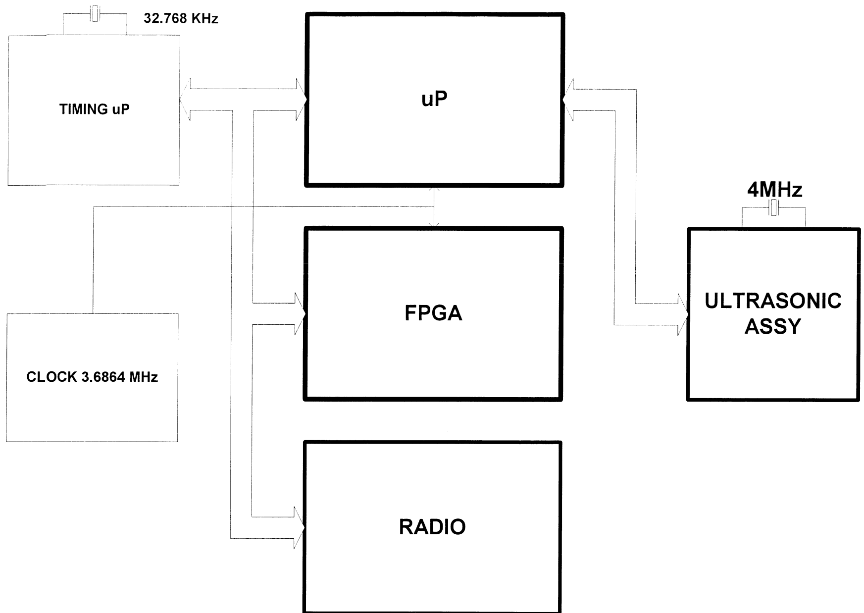
ULTRASONIC MONITOR BLK DIAGRAM
