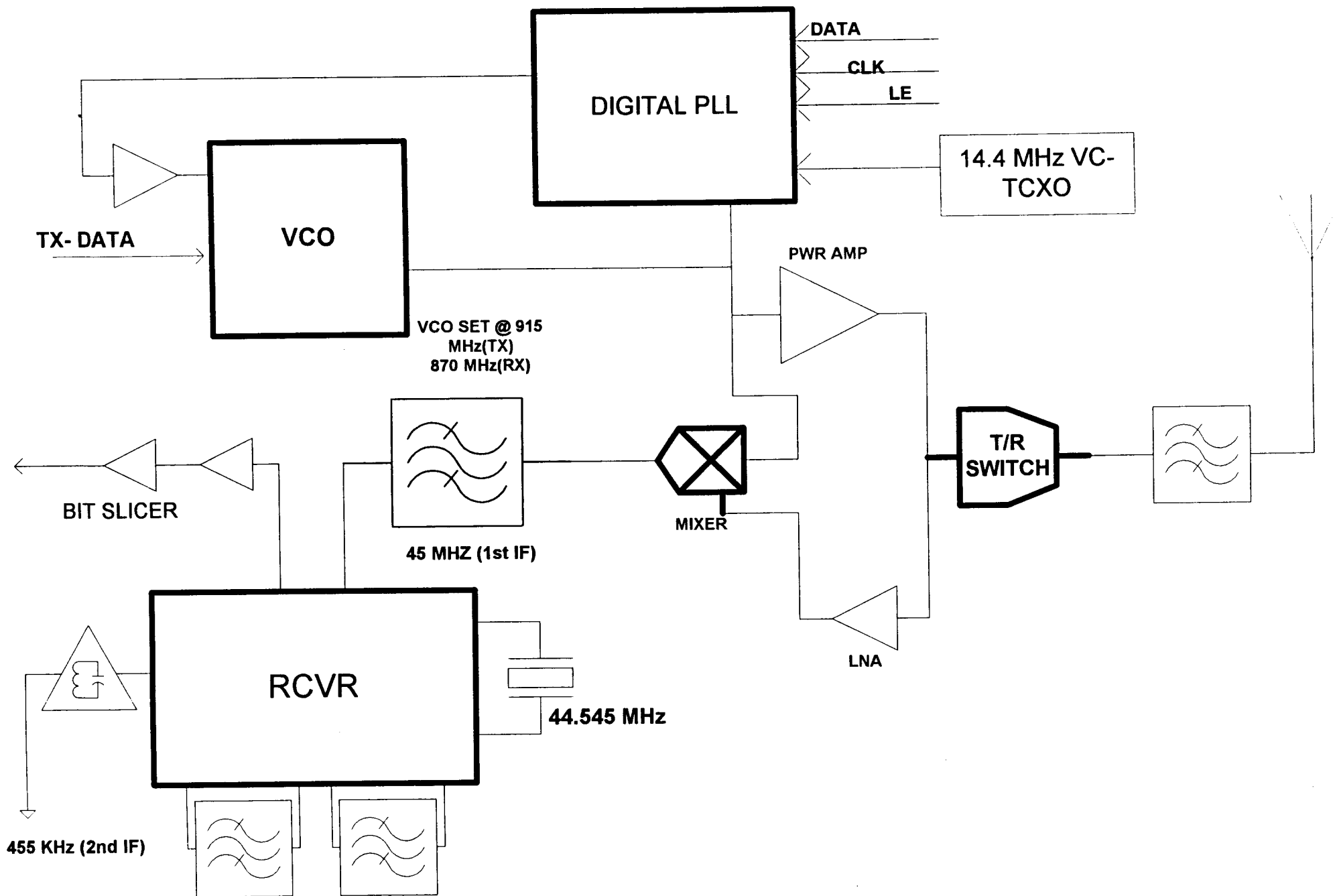
TRANSCEIVER BLK DIAGRAM
