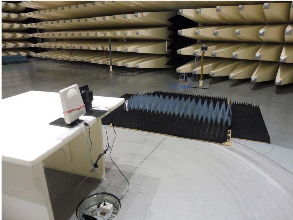
Photo 3: Radiated Emission
