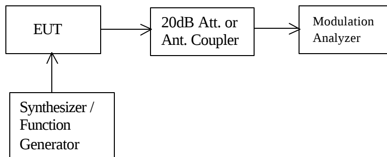
Figure 4: Modulation characteristic measurement configuration
