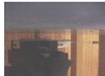
Figure 6. Body SAR Test Setup
