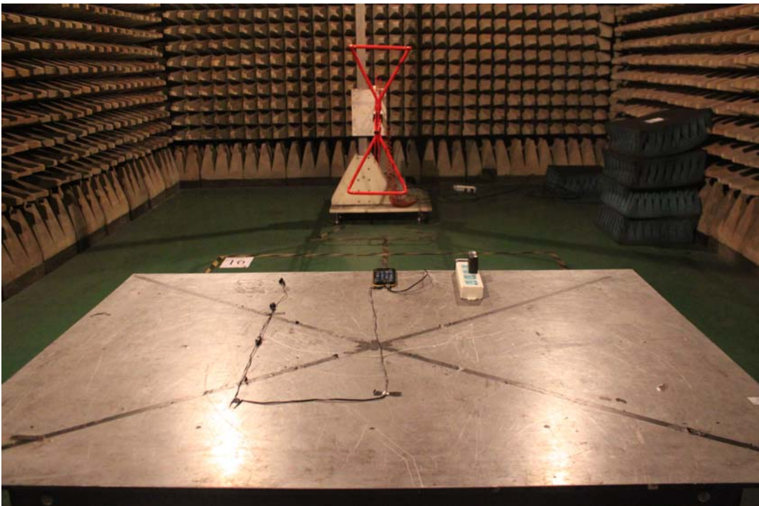
RE TEST SETUP
