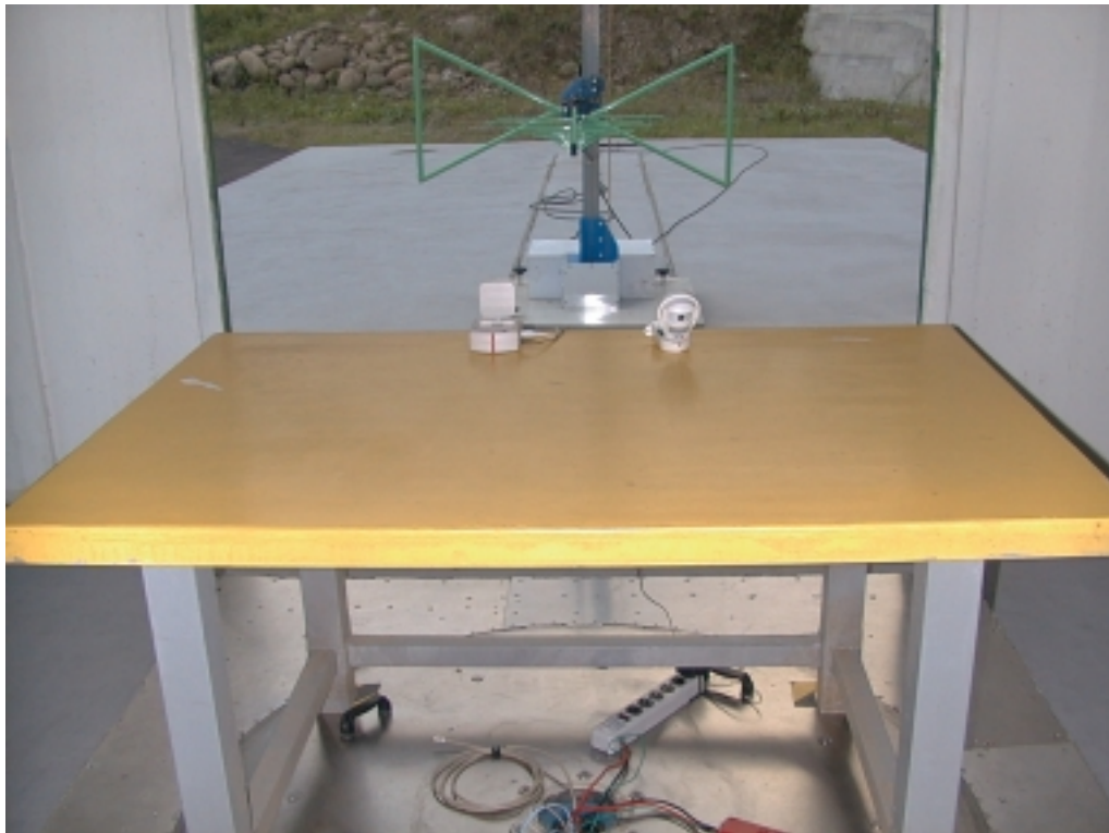
Back View of Radiated Test (M9310)
