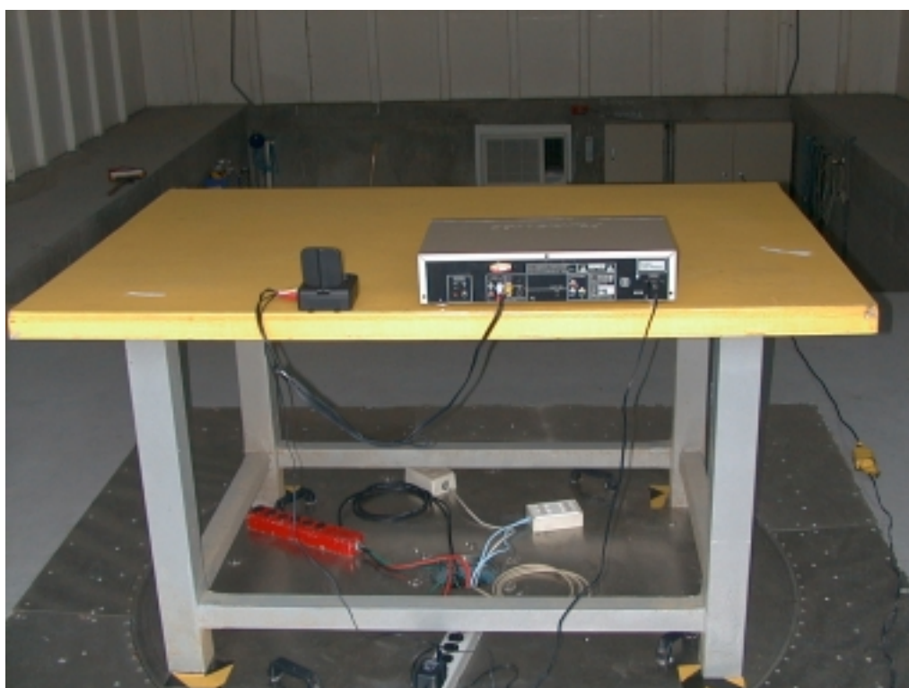
Back View of Radiated Test (M9312)
