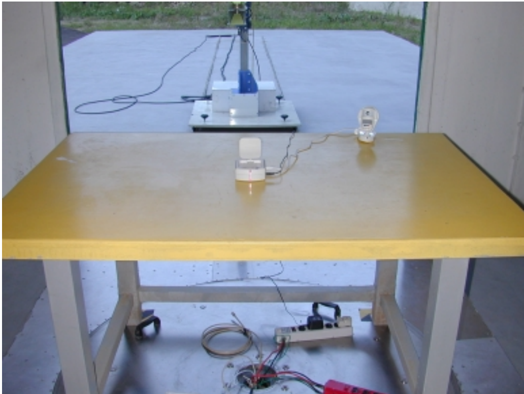
Front View of Radiated Test-HORN (M9312)
