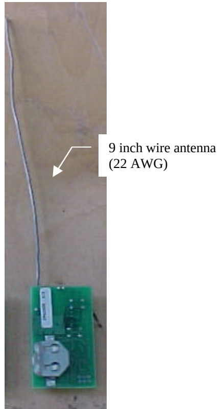
Figure 3 – Bottom Side of 433.92 MHz Transmitter (EUT)
