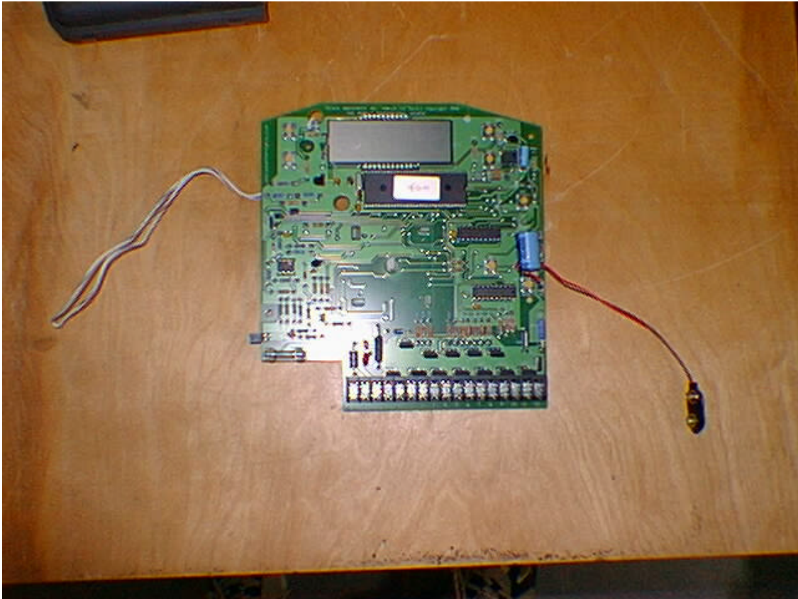
Figure 2 - Component Side of Weathermate (EUT)
