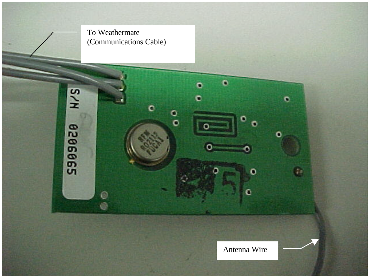
Figure 6 - Back Side of 433.92 MHz Receiver (EUT)
