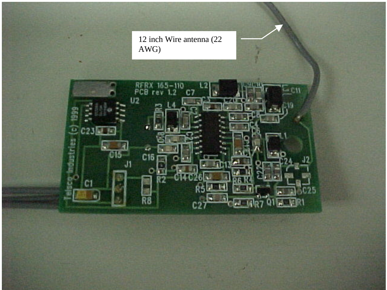
Figure 5 - Component Side of 433.92 MHz Receiver (EUT)
