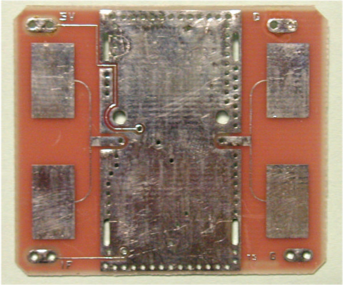
PCB REAR
