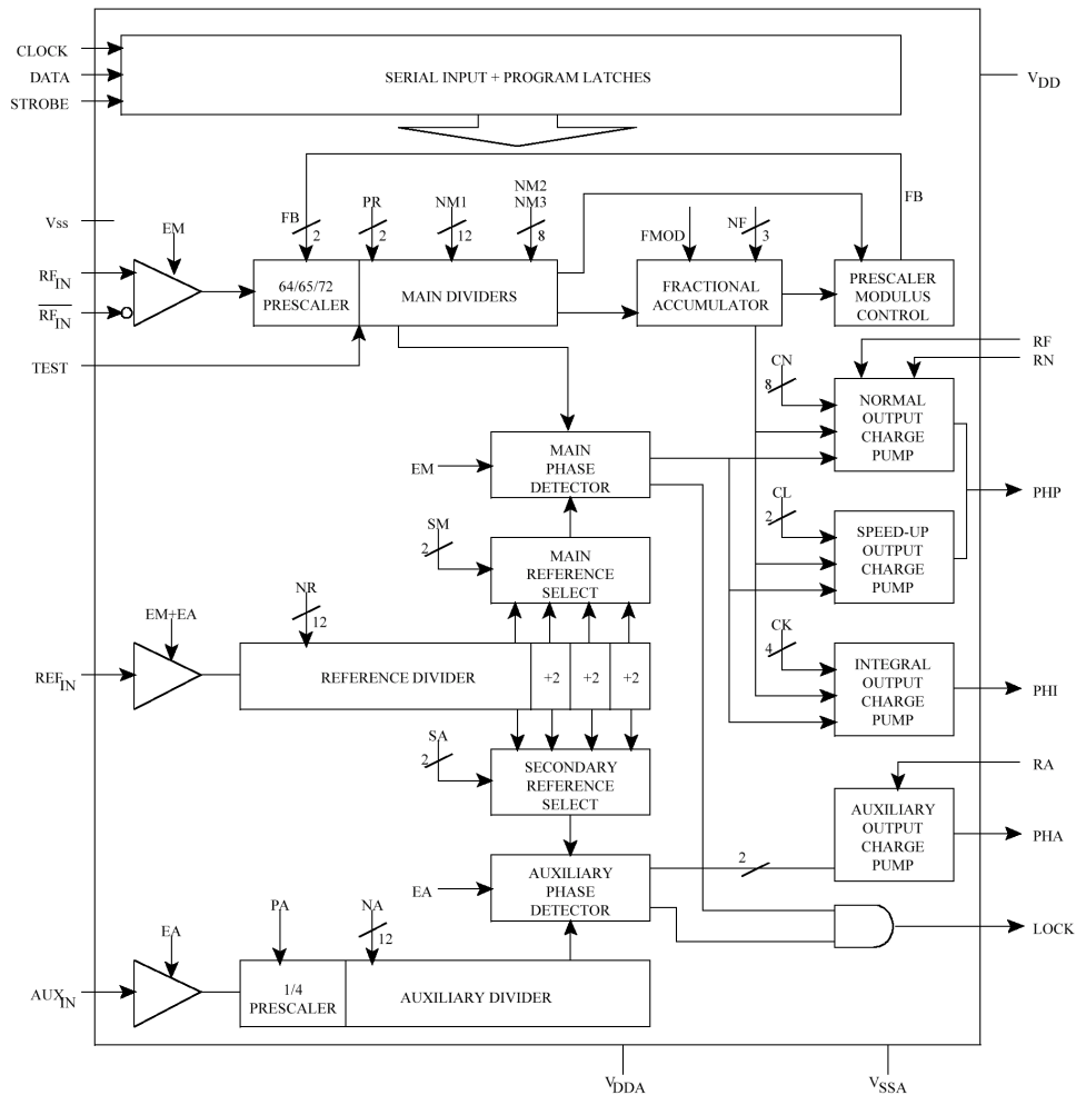
Figure 4-2 U801 SYNTHESIZER BLOCK DIAGRAM
