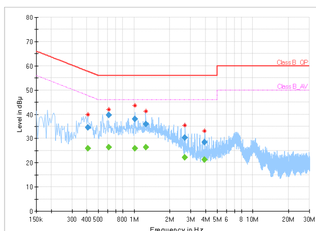
Full Spectrum
