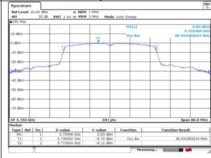
99% Occupied Bandwidth
