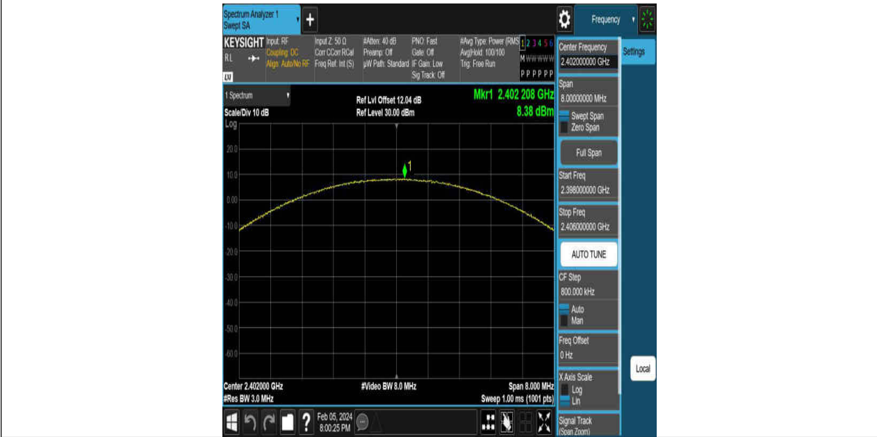
2DH5-Ant1-2402-PASS
