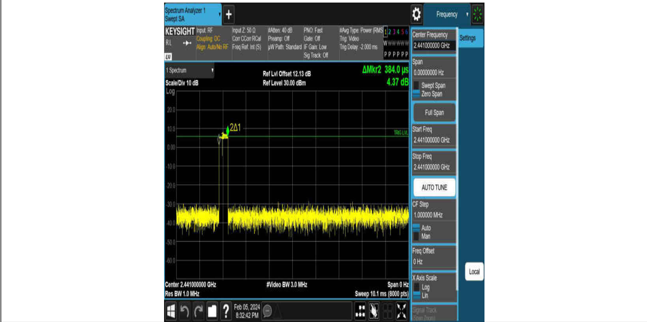
2DH1-Ant1-Hop-PASS
