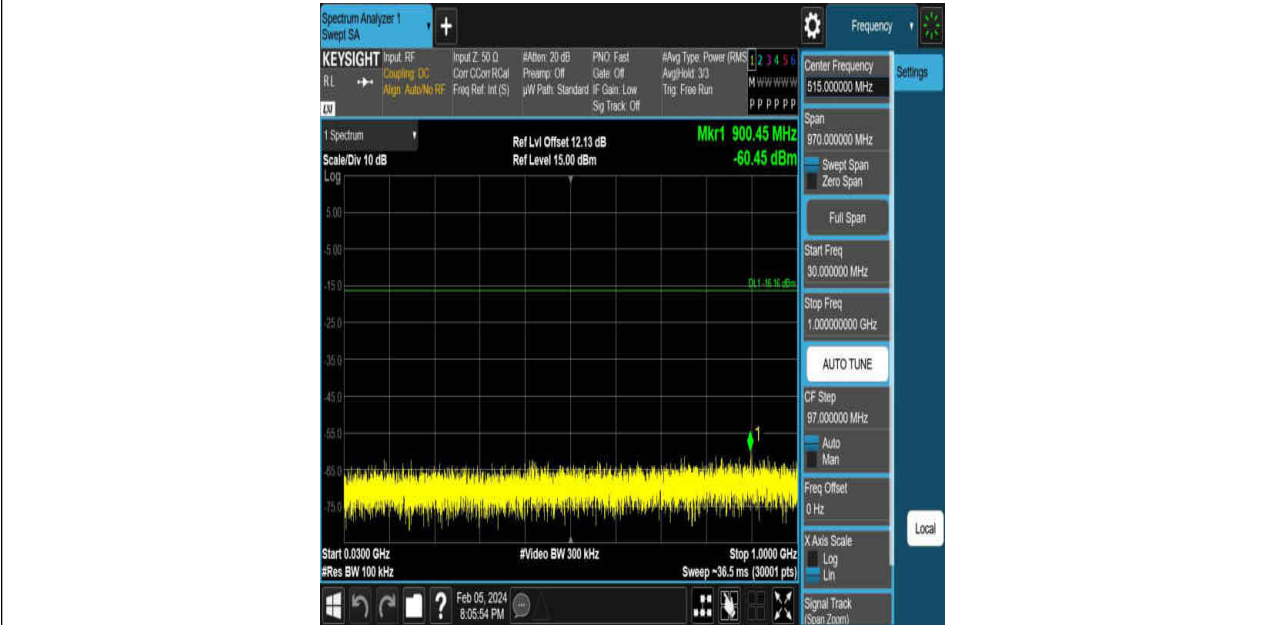
3DH5-Ant1-2441-30~1000-PASS
