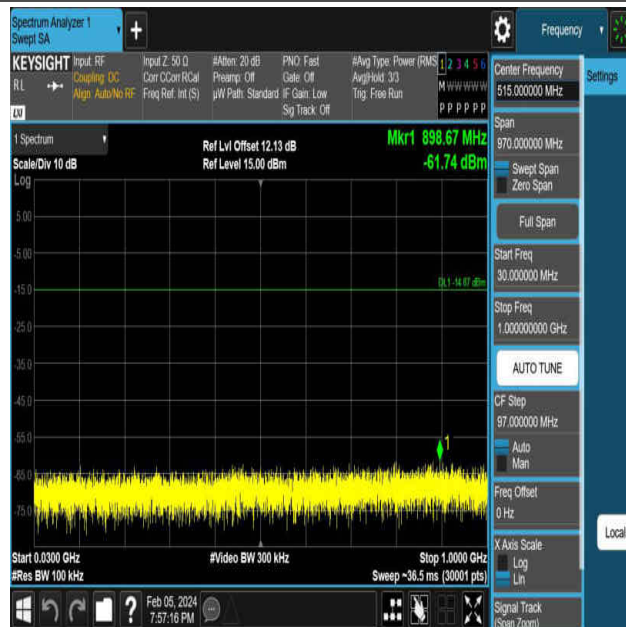
DH5-Ant1-2441-30~1000-PASS
