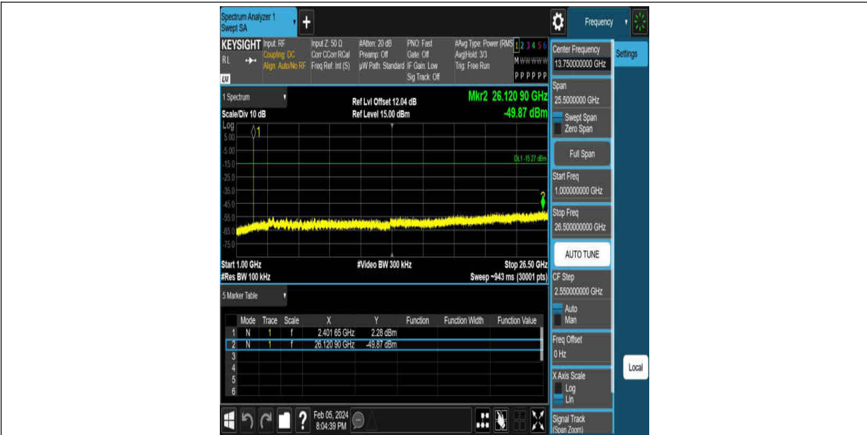
3DH5-Ant1-2402-1000~26500-PASS
