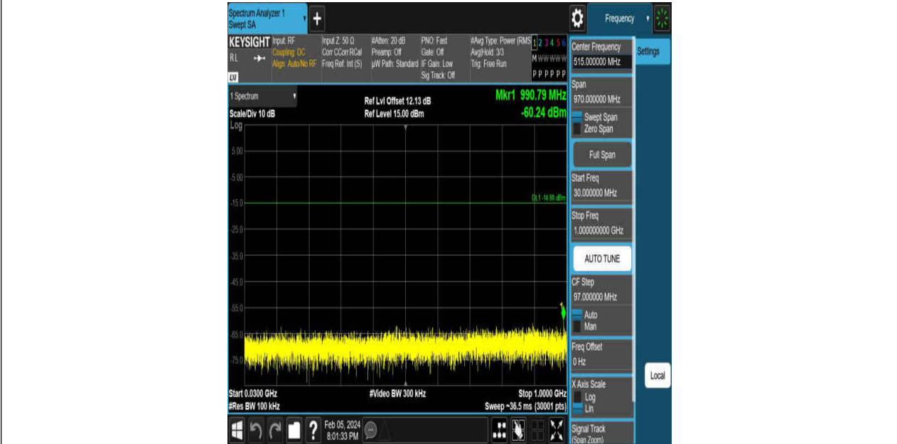
2DH5-Ant1-2441-30~1000-PASS
