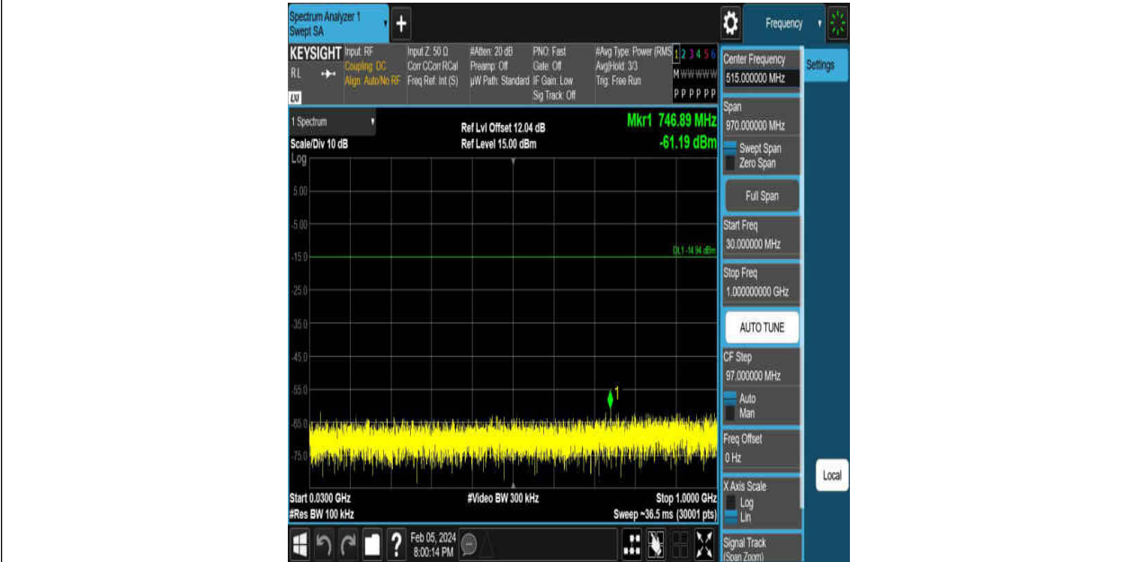
2DH5-Ant1-2402-30~1000-PASS
