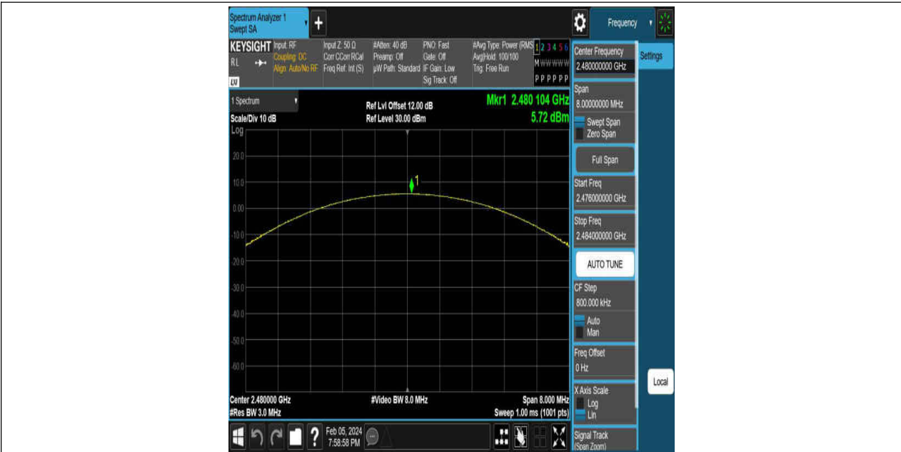
DH5-Ant1-2480-PASS
