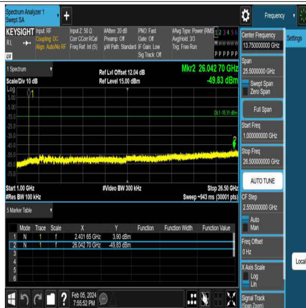
DH5-Ant1-2402-1000~26500-PASS
