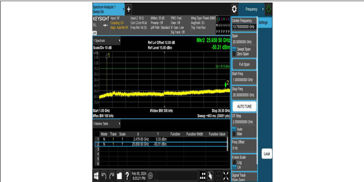
2DH5-Ant1-2480-1000~26500-PASS
