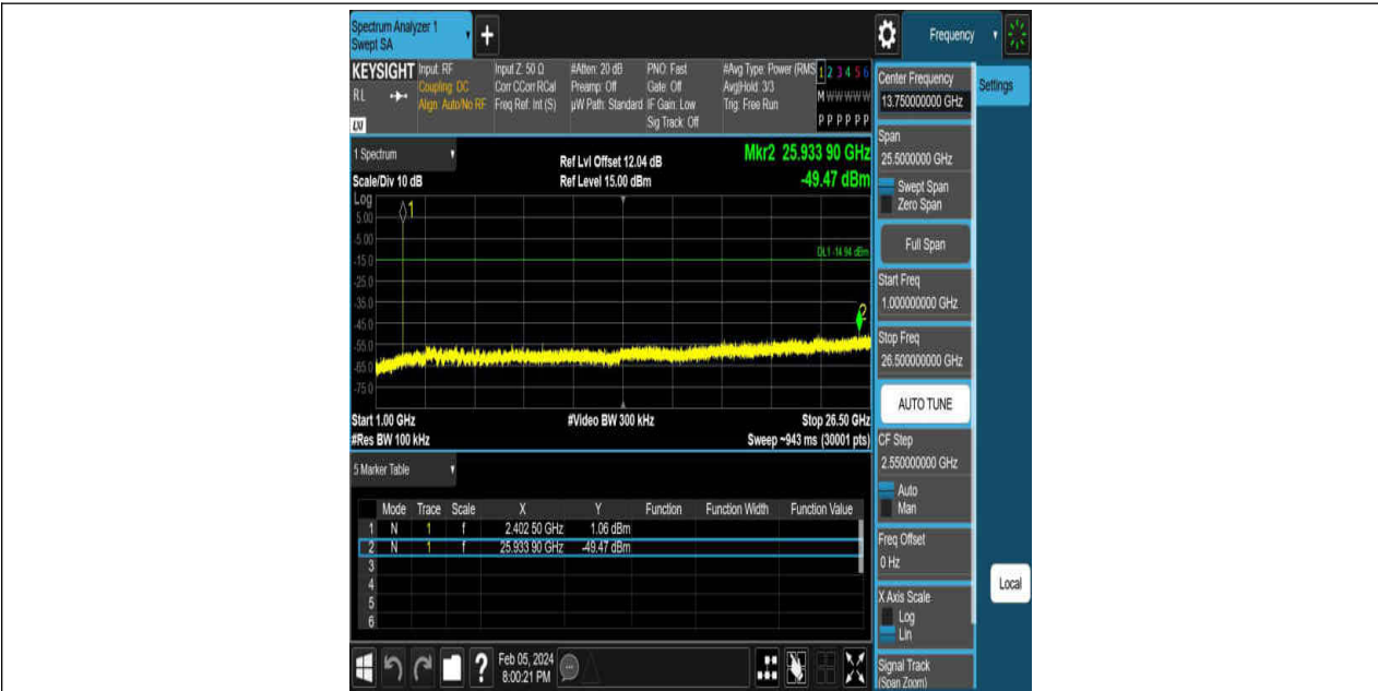
2DH5-Ant1-2402-1000~26500-PASS
