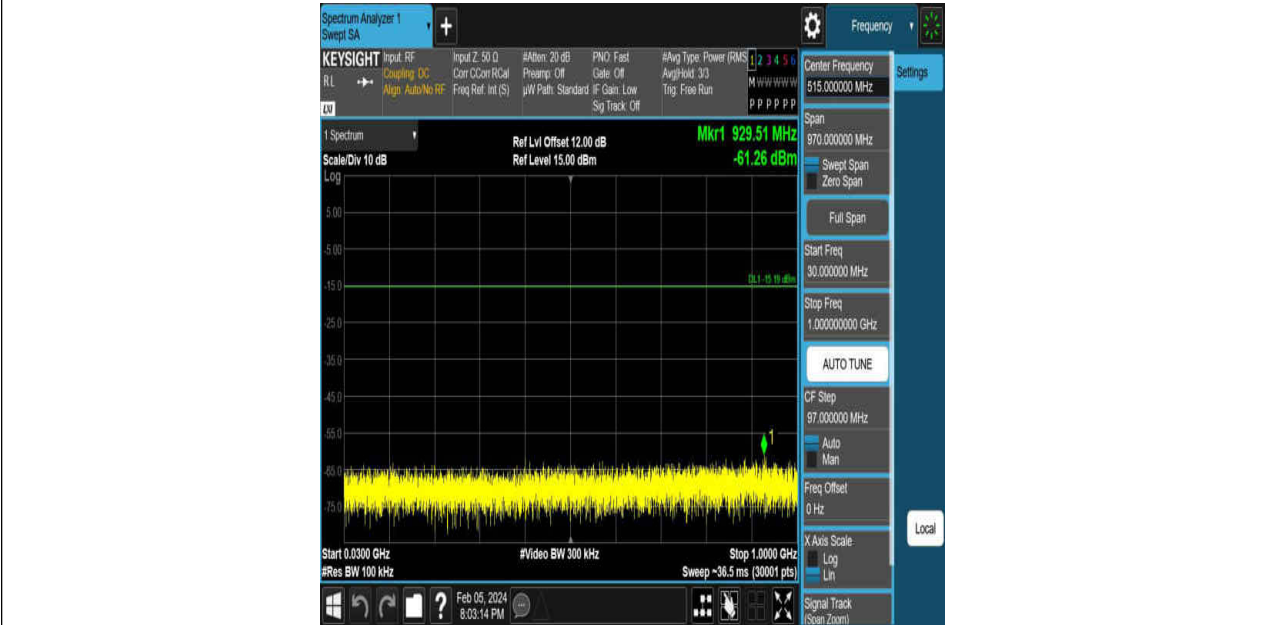
2DH5-Ant1-2480-30~1000-PASS
