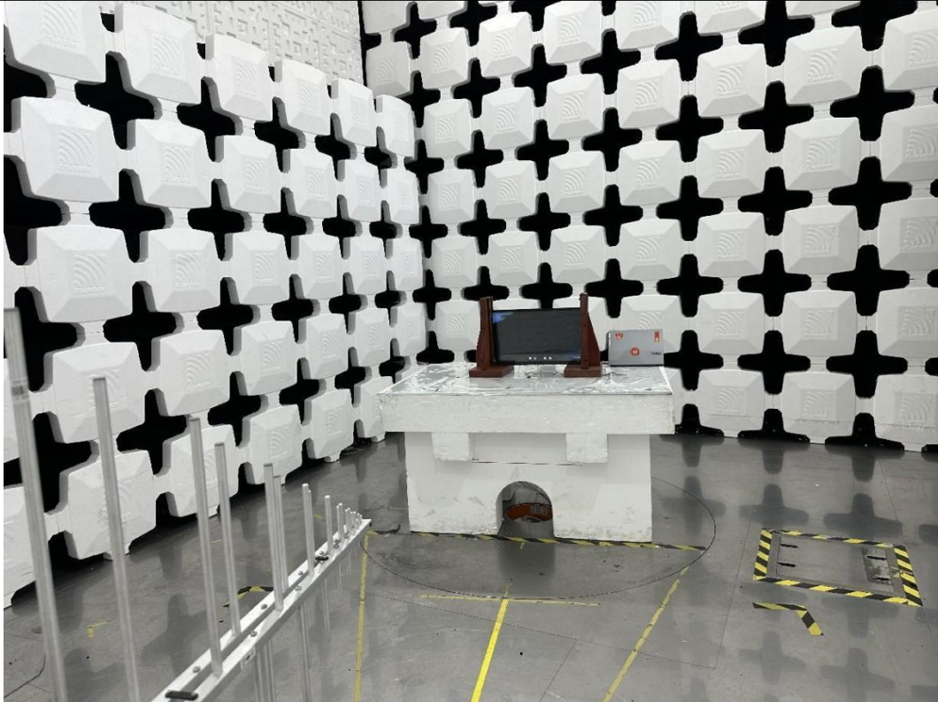
Radiated Emission Above 1G
