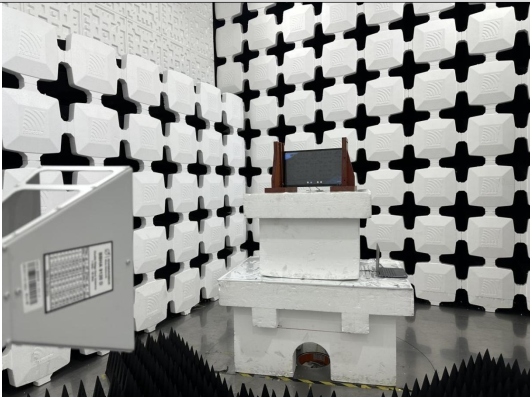
AC Power Conducted Emission
