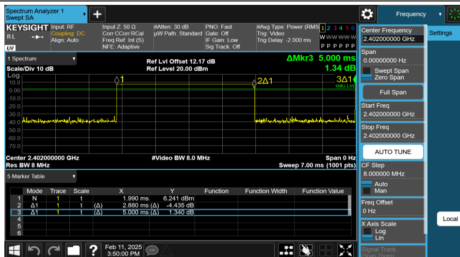
NTNV-DH5-Ant1-2402
