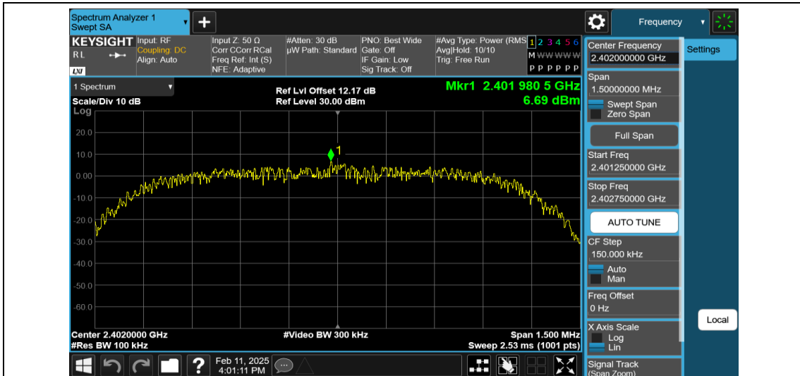
2DH5-Ant1-2402-0~Reference-PASS
