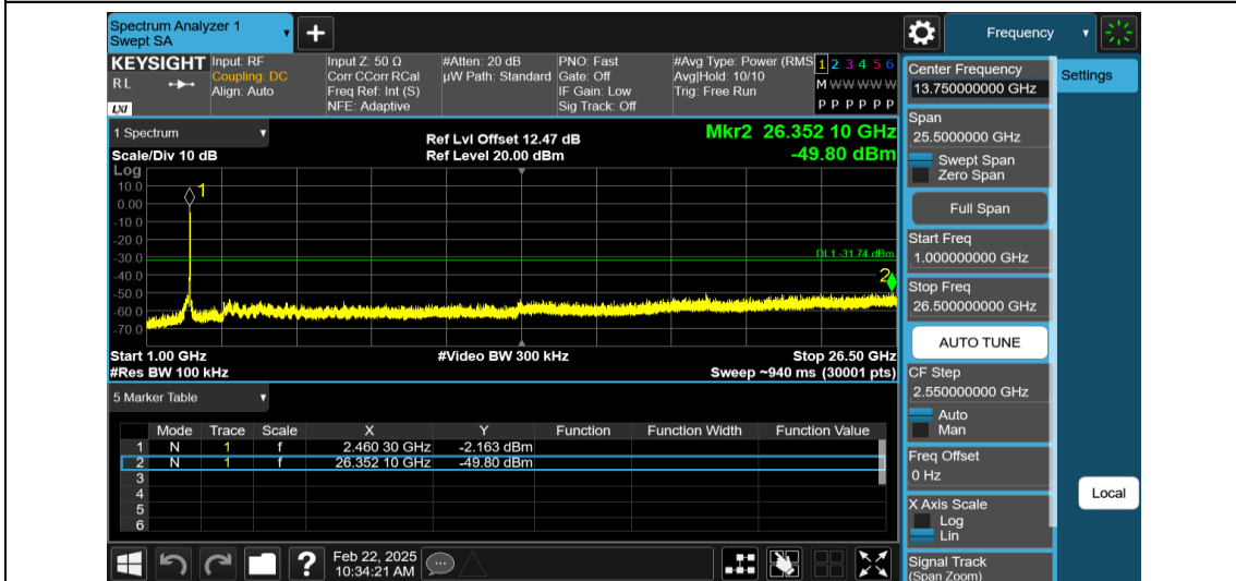
11AX20MIMO-Ant1-2462-1000~26500-PASS
