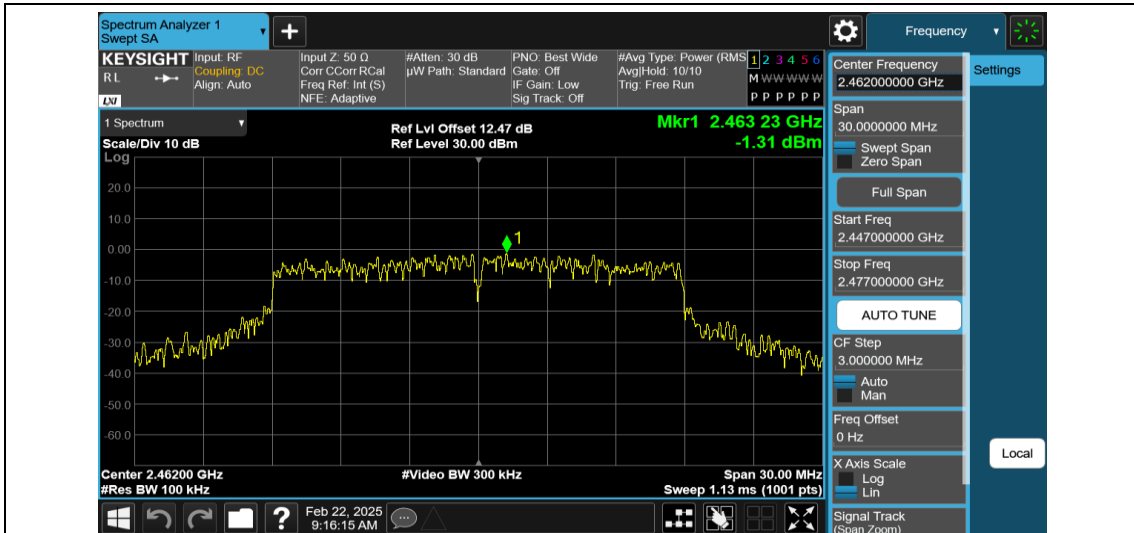
11N20MIMO-Ant1-2462-0~Reference-PASS
