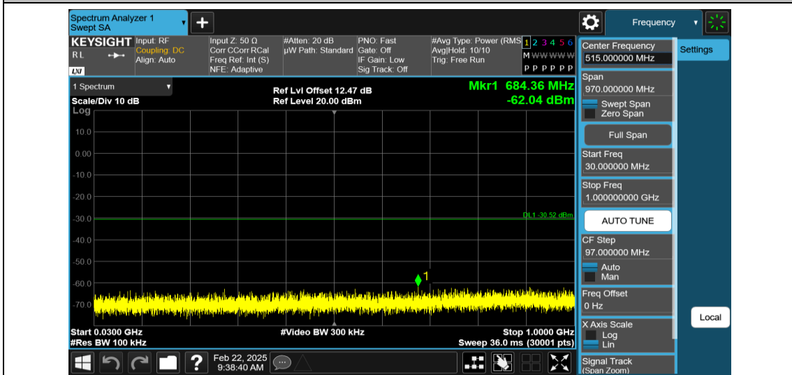
11N40MIMO-Ant1-2437-30~1000-PASS
