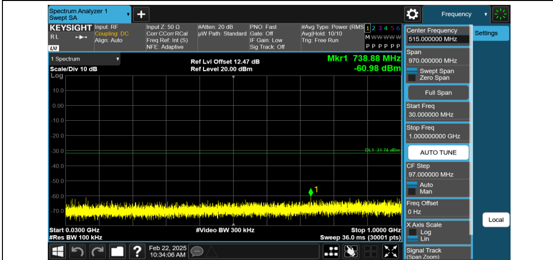
11AX20MIMO-Ant1-2462-30~1000-PASS
