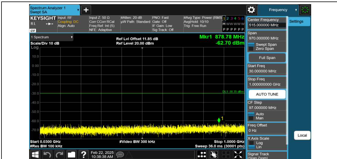
11AX20MIMO-Ant2-2462-30~1000-PASS
