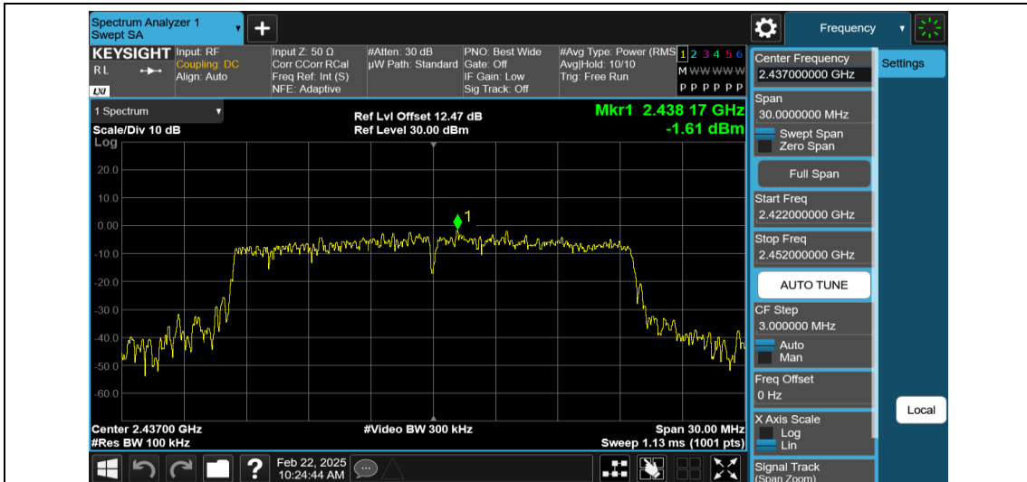
11AX20MIMO-Ant1-2437-0~Reference-PASS
