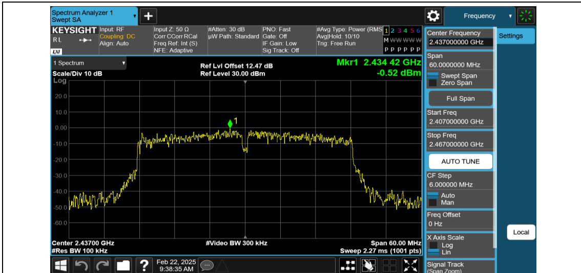
11N40MIMO-Ant1-2437-0~Reference-PASS
