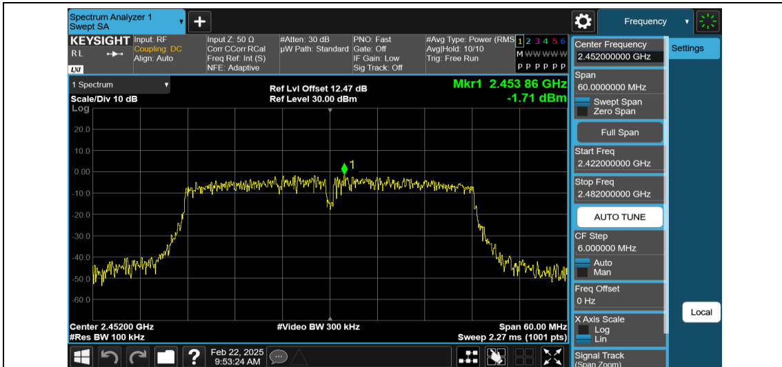
11N40MIMO-Ant1-2452-0~Reference-PASS
