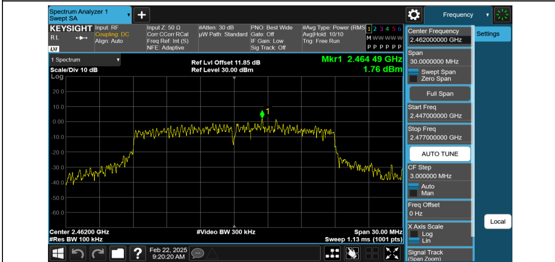
11N20MIMO-Ant2-2462-0~Reference-PASS
