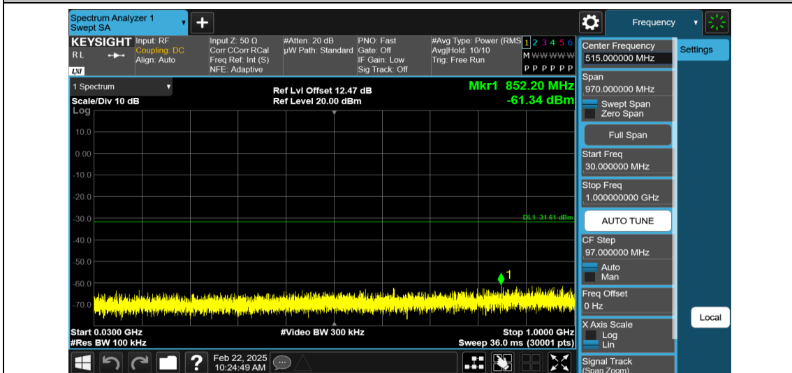
11AX20MIMO-Ant1-2437-30~1000-PASS
