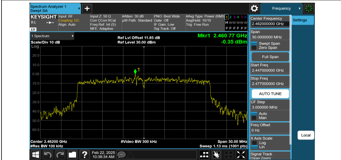
11AX20MIMO-Ant2-2462-0~Reference-PASS
