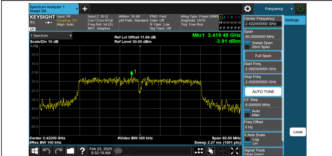
11N40MIMO-Ant2-2422-0~Reference-PASS
