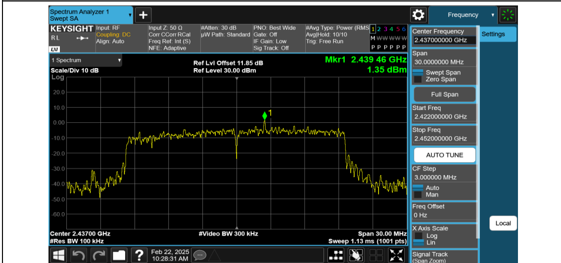
11AX20MIMO-Ant2-2437-0~Reference-PASS
