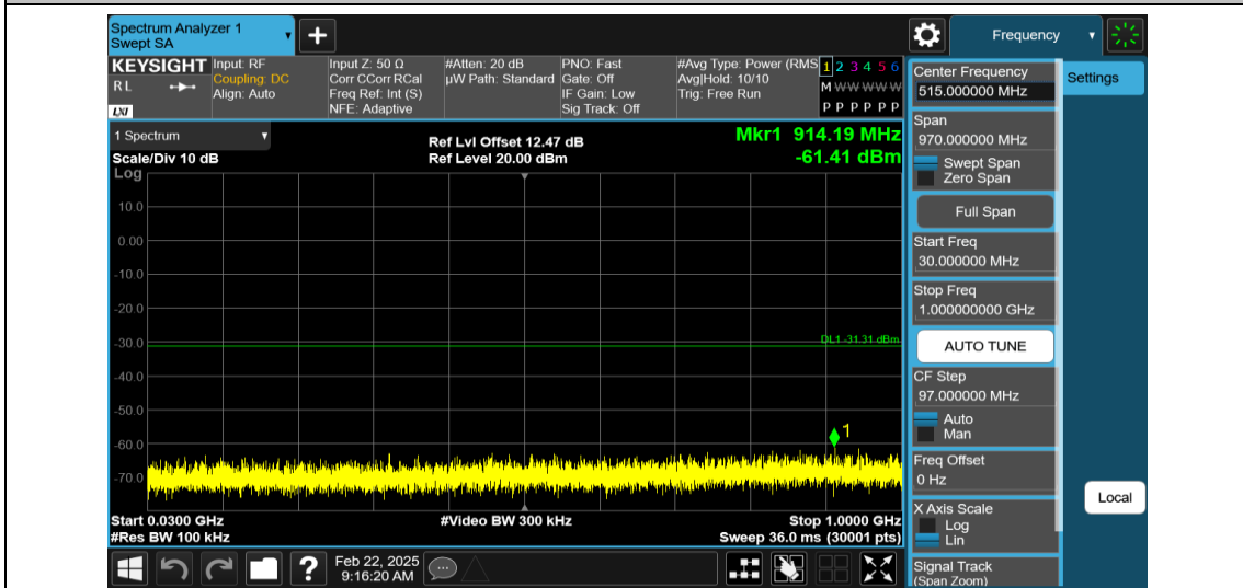
11N20MIMO-Ant1-2462-30~1000-PASS
