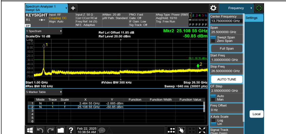
11AX20MIMO-Ant2-2462-1000~26500-PASS
