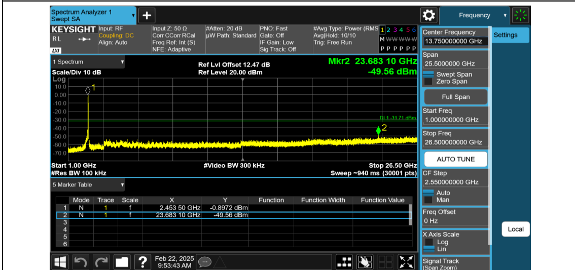
11N40MIMO-Ant1-2452-1000~26500-PASS
