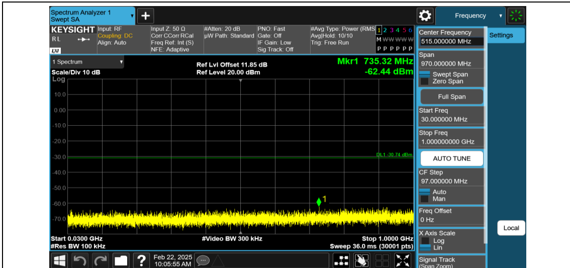
11N40MIMO-Ant2-2452-30~1000-PASS
