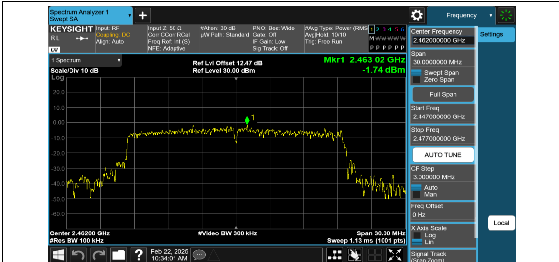
11AX20MIMO-Ant1-2462-0~Reference-PASS
