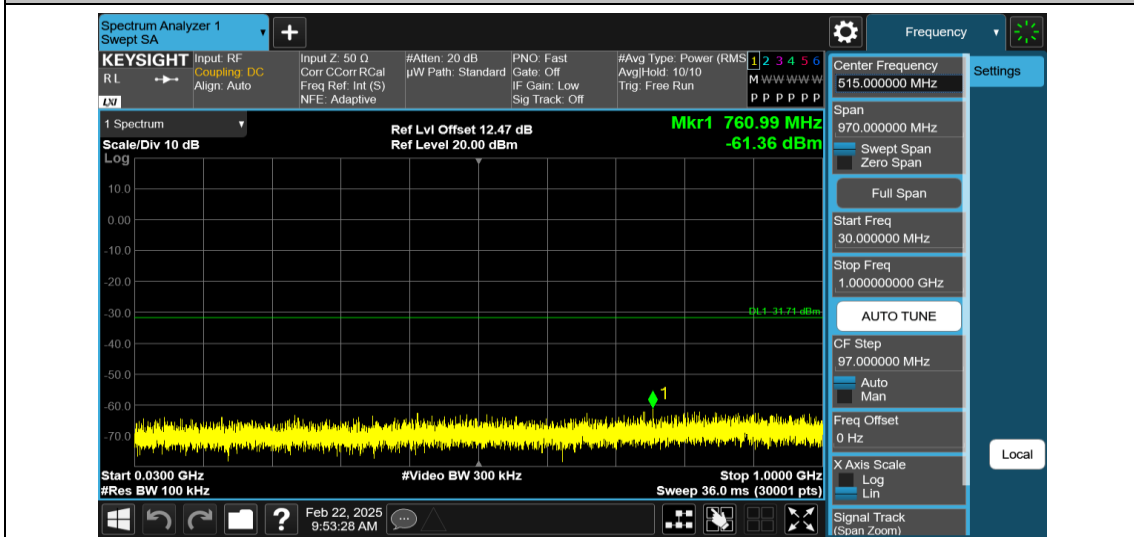
11N40MIMO-Ant1-2452-30~1000-PASS
