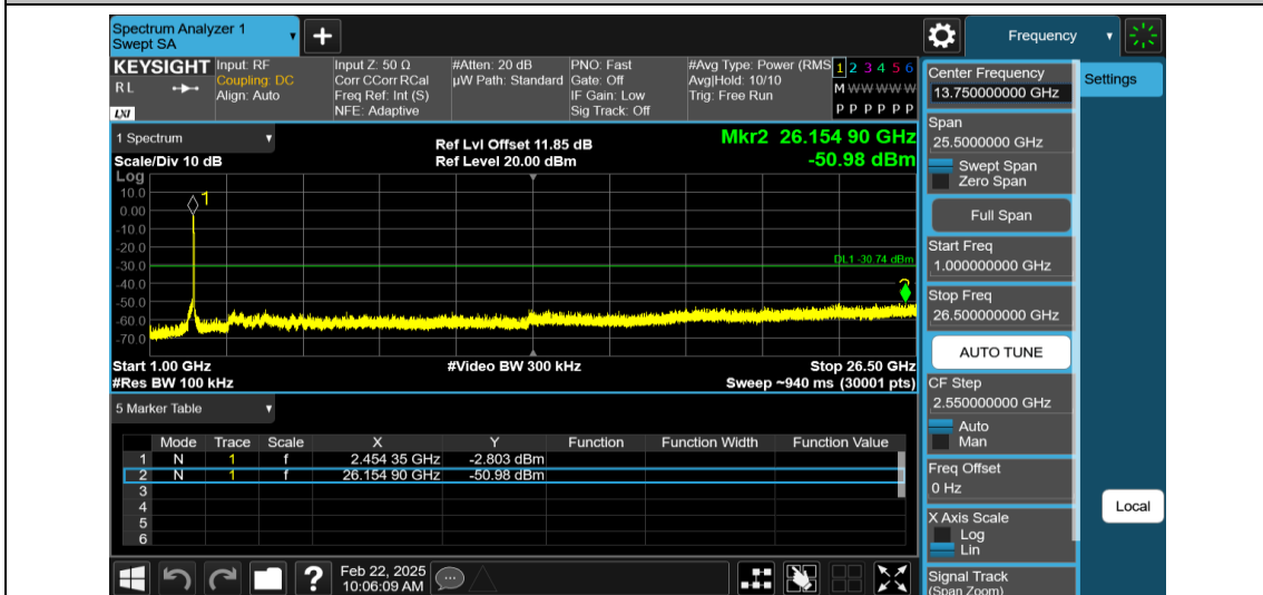
11N40MIMO-Ant2-2452-1000~26500-PASS
