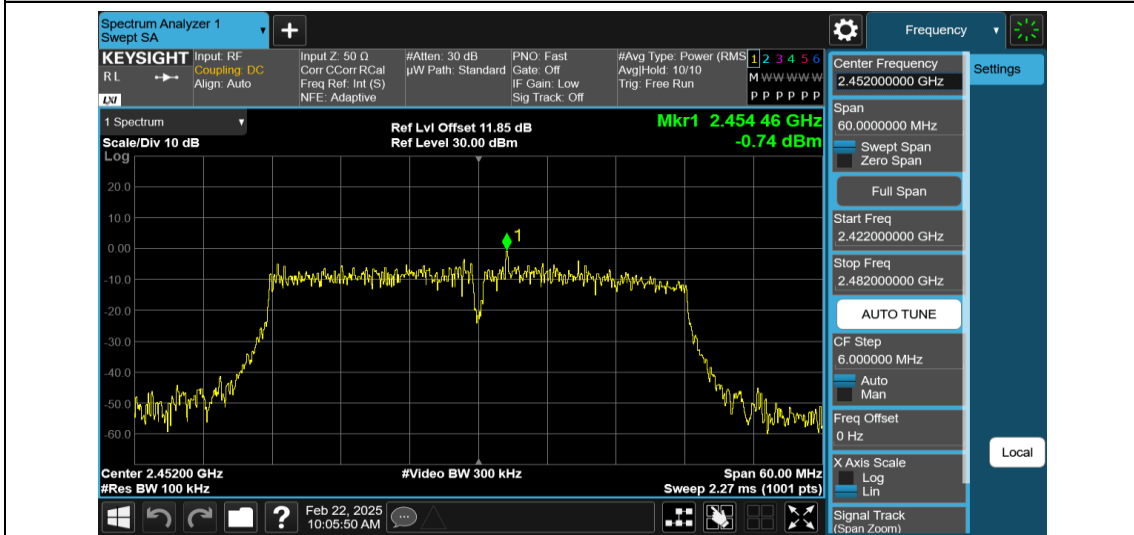
11N40MIMO-Ant2-2452-0~Reference-PASS
