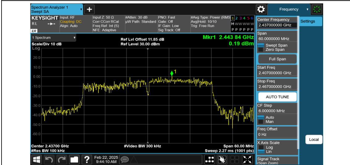
11N40MIMO-Ant2-2437-0~Reference-PASS
