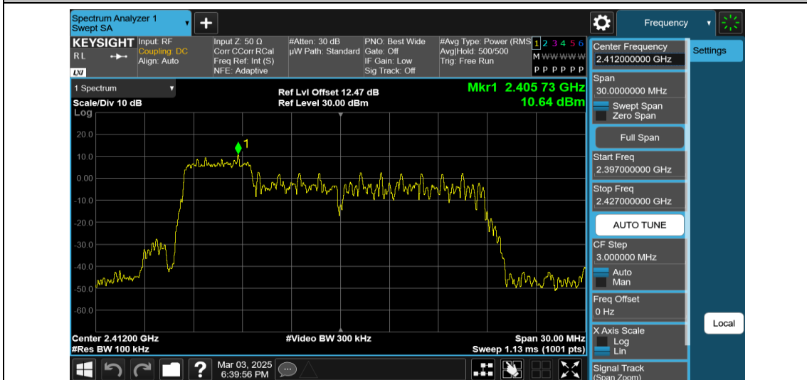
11AX20MIMO-Ant1-2412-52Tone-RU37-0~Reference-PASS
