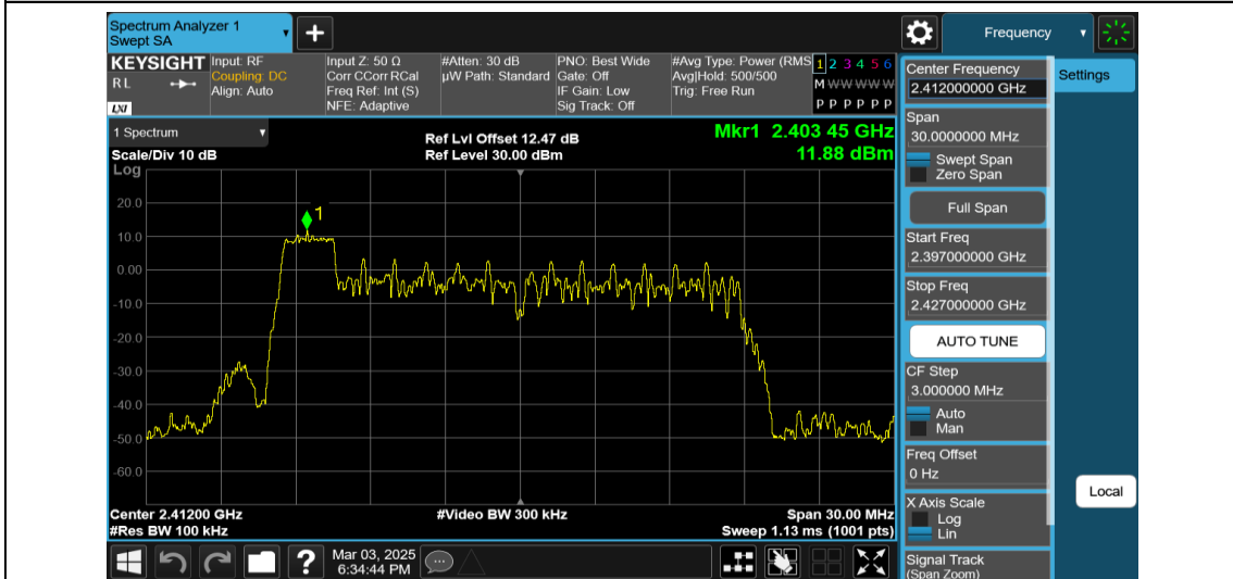
11AX20MIMO-Ant1-2412-26Tone-RU0-0~Reference-PASS
