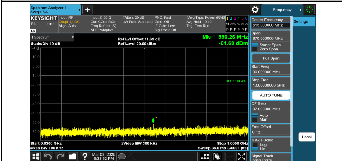
11AX20MIMO-Ant2-2412-26Tone-RU0-30~1000-PASS
