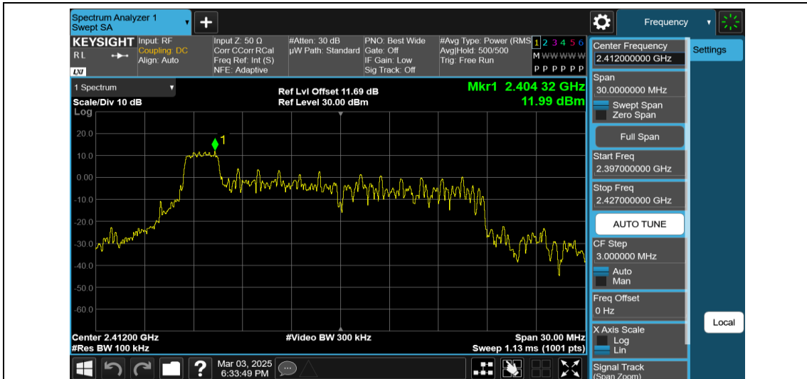
11AX20MIMO-Ant2-2412-26Tone-RU0-0~Reference-PASS
