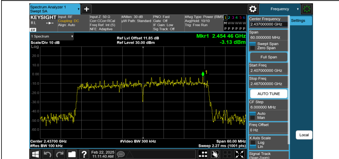
11AX40MIMO-Ant2-2437-0~Reference-PASS
