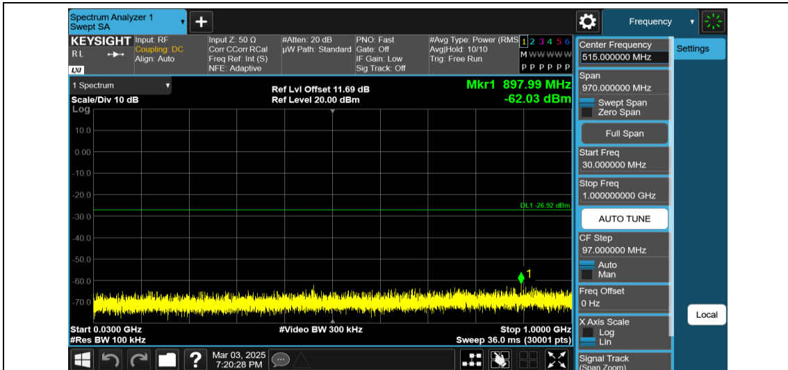
11AX20MIMO-Ant2-2412-106Tone-RU53-30~1000-PASS
