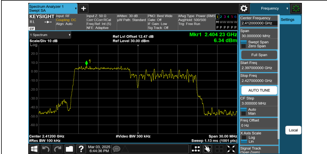
11AX20MIMO-Ant1-2412-106Tone-RU53-0~Reference-PASS
