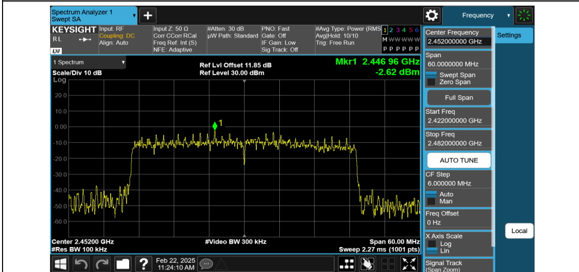
11AX40MIMO-Ant2-2452-0~Reference-PASS
