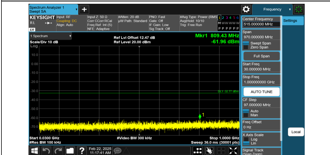
11AX40MIMO-Ant1-2452-30~1000-PASS
