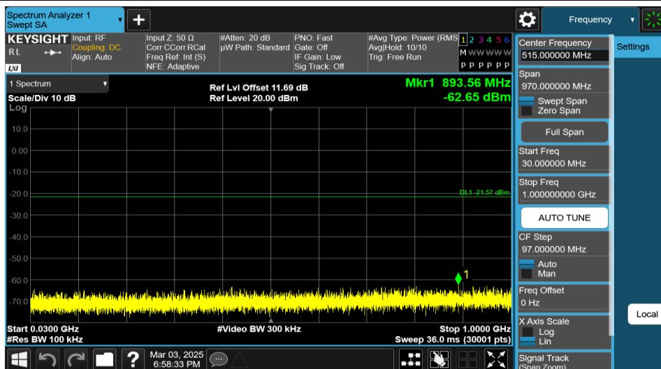
11AX20MIMO-Ant2-2412-52Tone-RU37-30~1000-PASS
