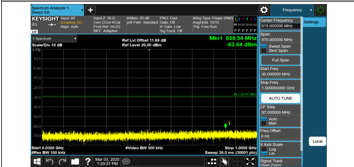
11AX20MIMO-Ant2-2412-242Tone-RU61-30~1000-PASS
