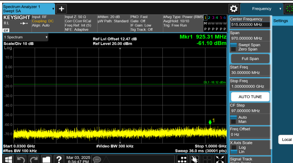
11AX20MIMO-Ant1-2412-26Tone-RU0-30~1000-PASS
