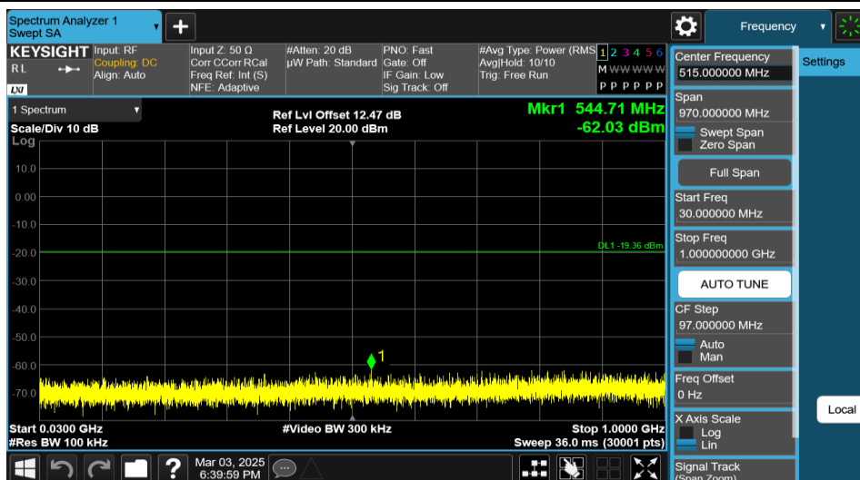
11AX20MIMO-Ant1-2412-52Tone-RU37-30~1000-PASS
