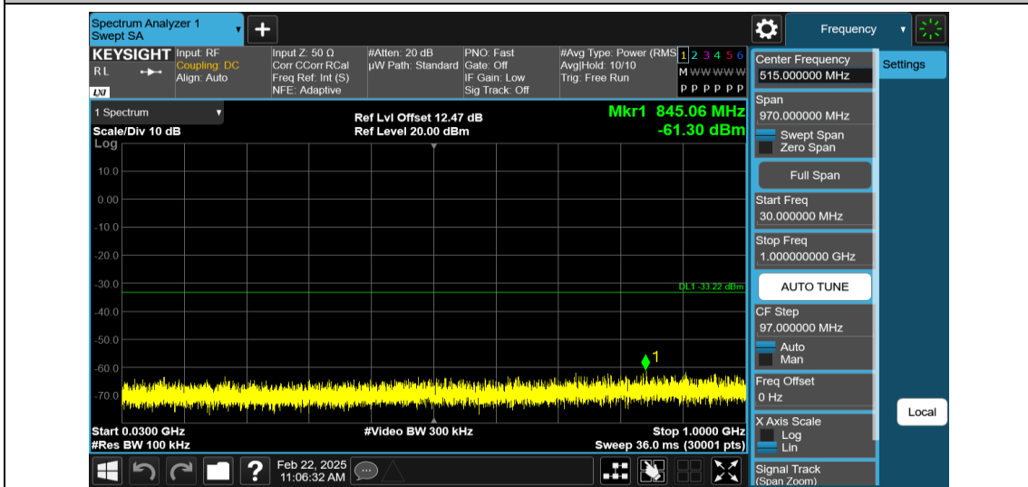
11AX40MIMO-Ant1-2437-30~1000-PASS
