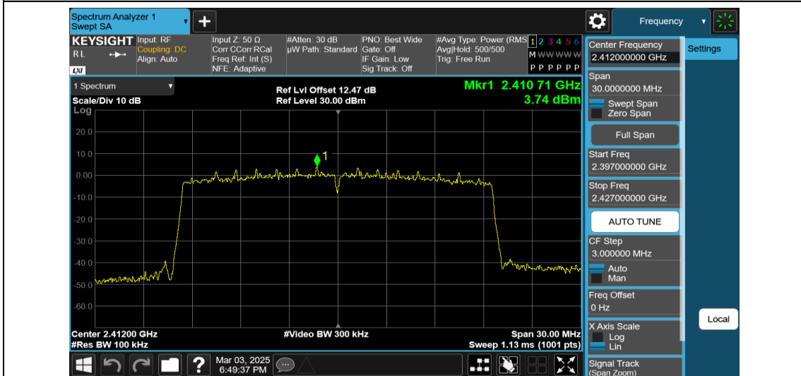
11AX20MIMO-Ant1-2412-242Tone-RU61-0~Reference-PASS
