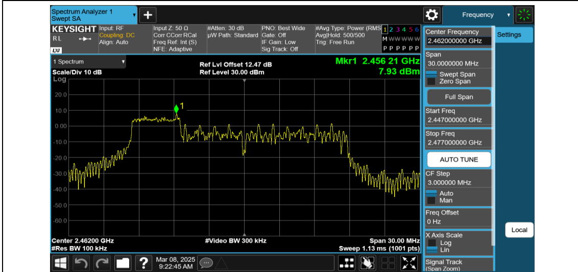
11AX20MIMO-Ant1-2462-52Tone-RU37-0~Reference-PASS
