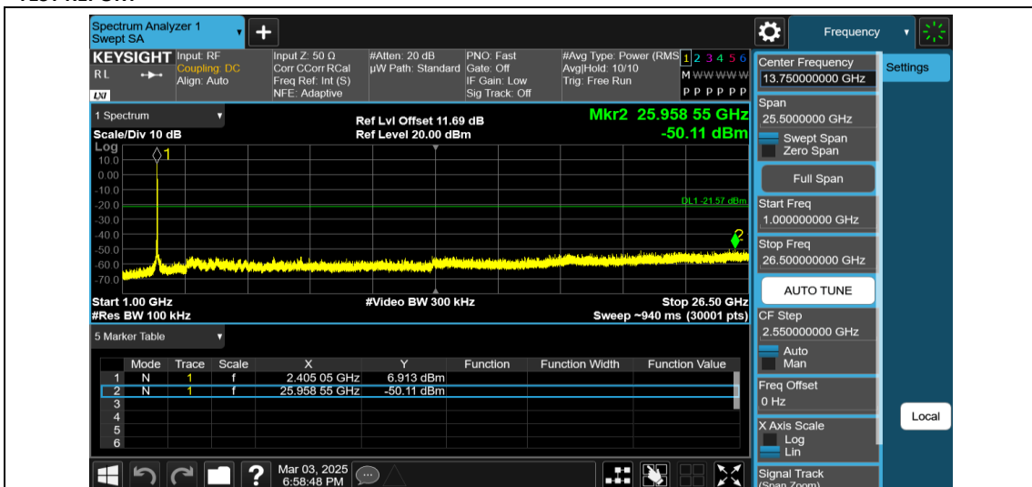
11AX20MIMO-Ant2-2412-52Tone-RU37-1000~26500-PASS
