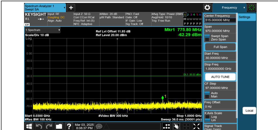
11AX20MIMO-Ant2-2437-242Tone-RU61-30~1000-PASS
