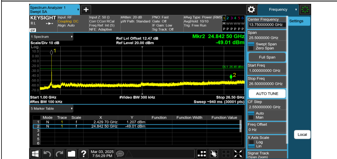
11AX20MIMO-Ant1-2437-106Tone-RU53-1000~26500-PASS
