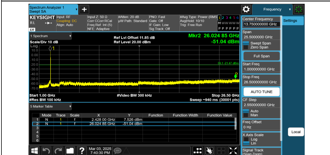
11AX20MIMO-Ant2-2437-26Tone-RU0-1000~26500-PASS
