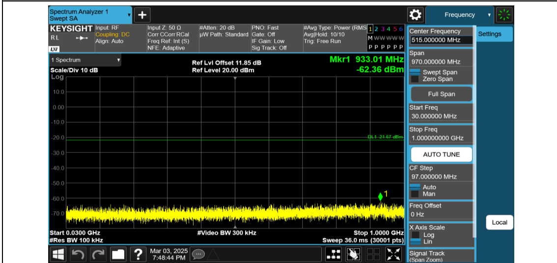
11AX20MIMO-Ant2-2437-52Tone-RU37-30~1000-PASS
