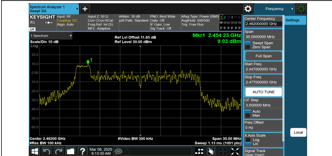
11AX20MIMO-Ant2-2462-26Tone-RU0-0~Reference-PASS
