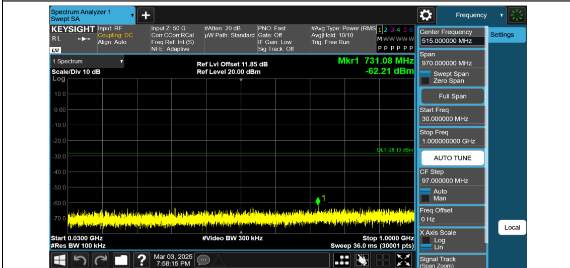
11AX20MIMO-Ant2-2437-106Tone-RU53-30~1000-PASS
