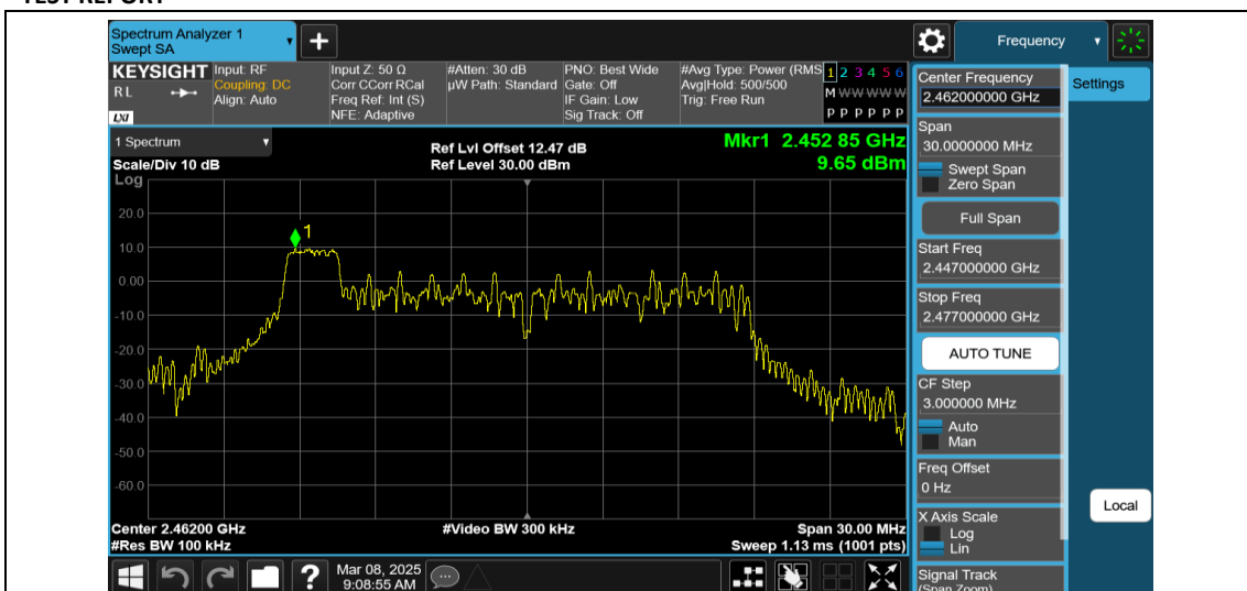
11AX20MIMO-Ant1-2462-26Tone-RU0-0~Reference-PASS
