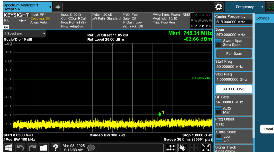
11AX20MIMO-Ant2-2462-26Tone-RU0-30~1000-PASS
