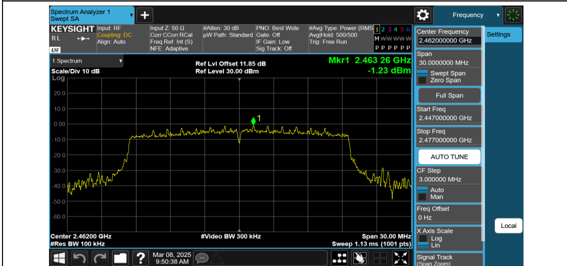
11AX20MIMO-Ant2-2462-242Tone-RU61-0~Reference-PASS
