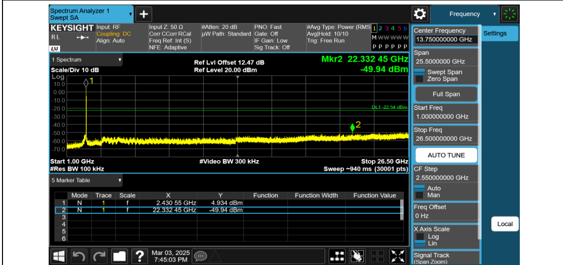
11AX20MIMO-Ant1-2437-52Tone-RU37-1000~26500-PASS
