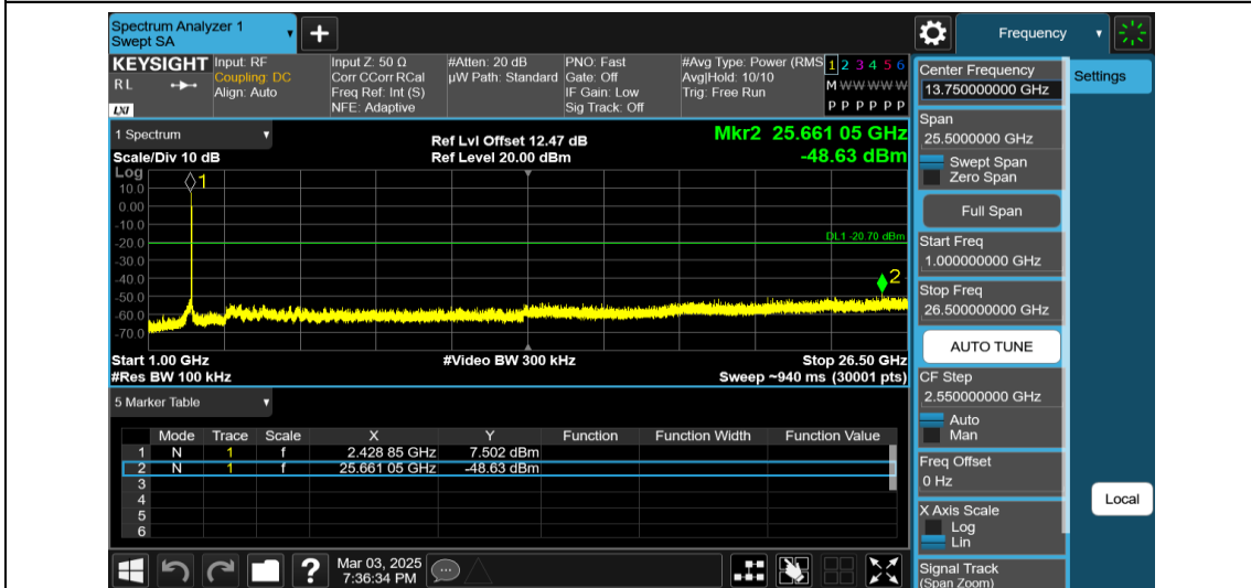
11AX20MIMO-Ant1-2437-26Tone-RU0-1000~26500-PASS
