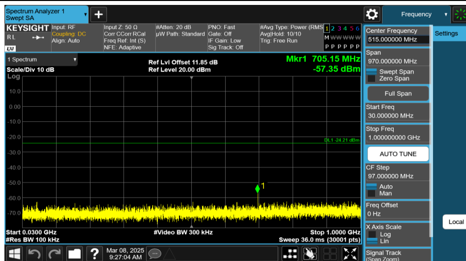
11AX20MIMO-Ant2-2462-52Tone-RU37-30~1000-PASS
