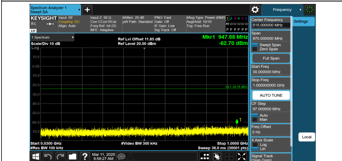
11AX40MIMO-Ant2-2452-26Tone-RU0-30~1000-PASS
