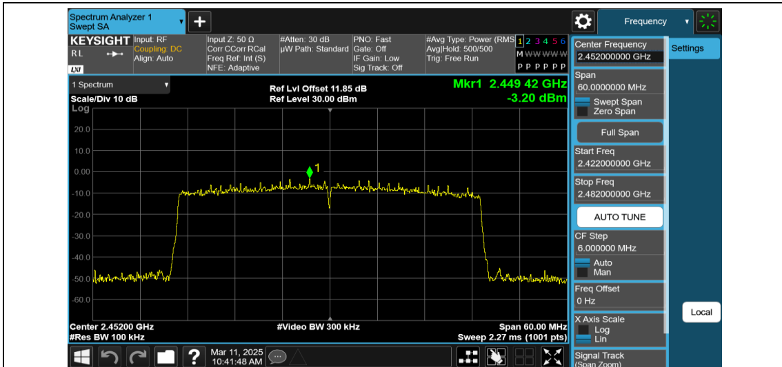
11AX40MIMO-Ant2-2452-484Tone-RU65-0~Reference-PASS
