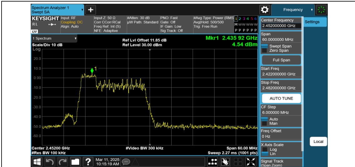
11AX40MIMO-Ant2-2452-52Tone-RU37-0~Reference-PASS
