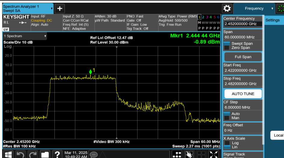
11AX40MIMO-Ant1-2452-242Tone-RU61-0~Reference-PASS
