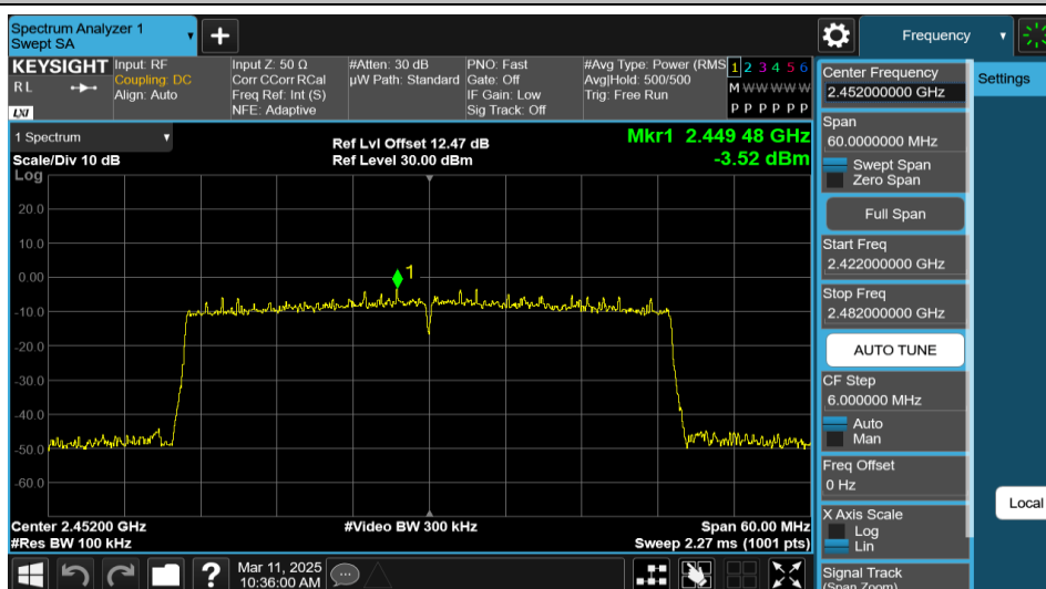
11AX40MIMO-Ant1-2452-484Tone-RU65-0~Reference-PASS
