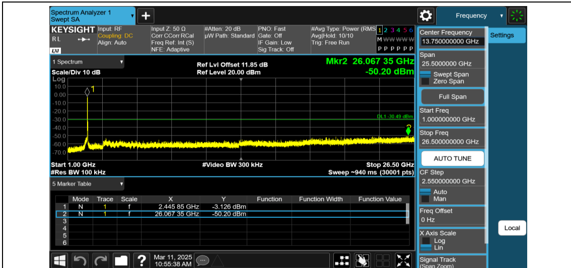
11AX40MIMO-Ant2-2452-242Tone-RU61-1000~26500-PASS
