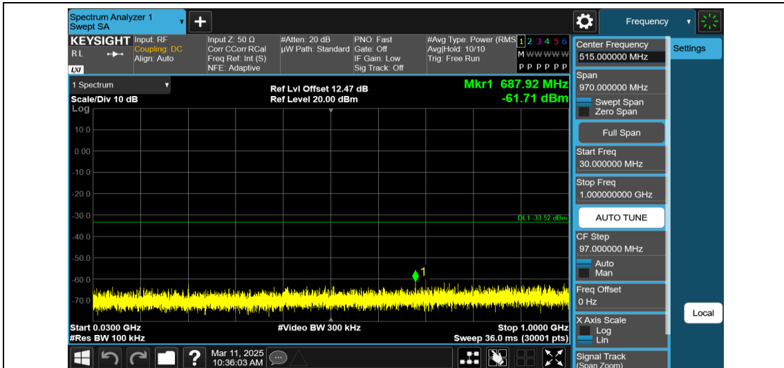
11AX40MIMO-Ant1-2452-484Tone-RU65-30~1000-PASS
