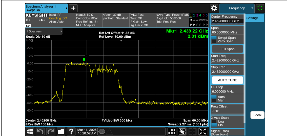
11AX40MIMO-Ant2-2452-106Tone-RU53-0~Reference-PASS
