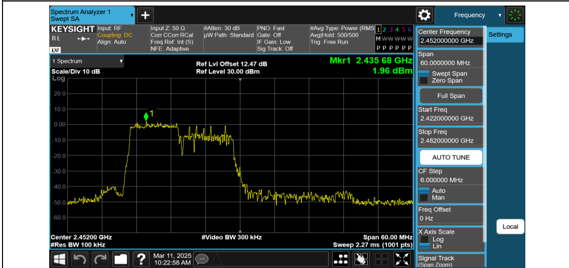
11AX40MIMO-Ant1-2452-106Tone-RU53-0~Reference-PASS
