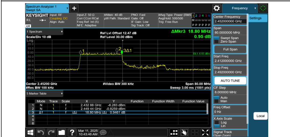
11AX40MIMO-Ant1-2452-242Tone-RU61-PASS
