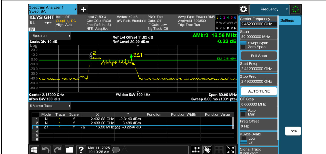
11AX40MIMO-Ant2-2452-52Tone-RU37-PASS
