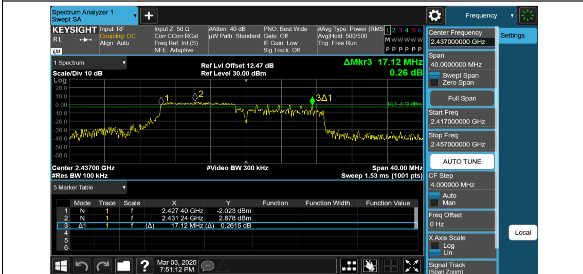
11AX20MIMO-Ant1-2437-106Tone-RU53-PASS
