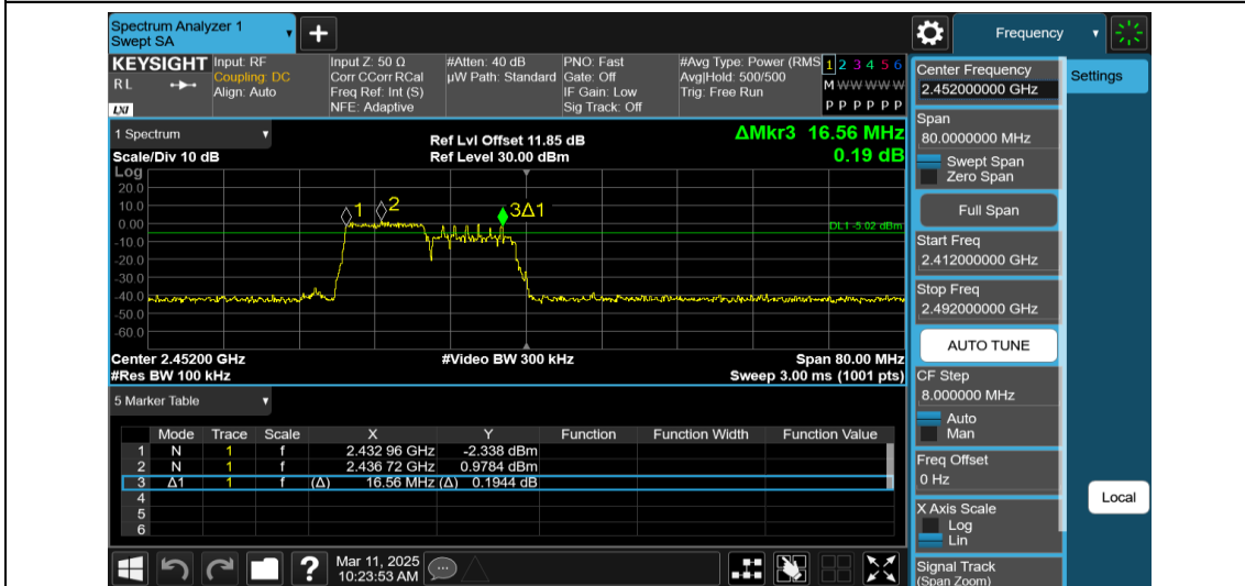
11AX40MIMO-Ant2-2452-106Tone-RU53-PASS
