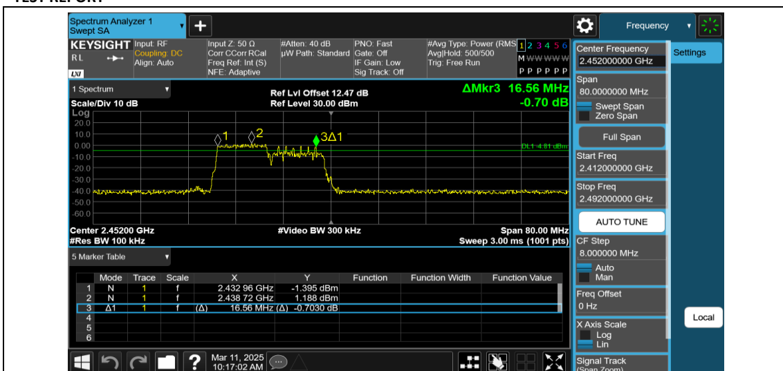
11AX40MIMO-Ant1-2452-106Tone-RU53-PASS
