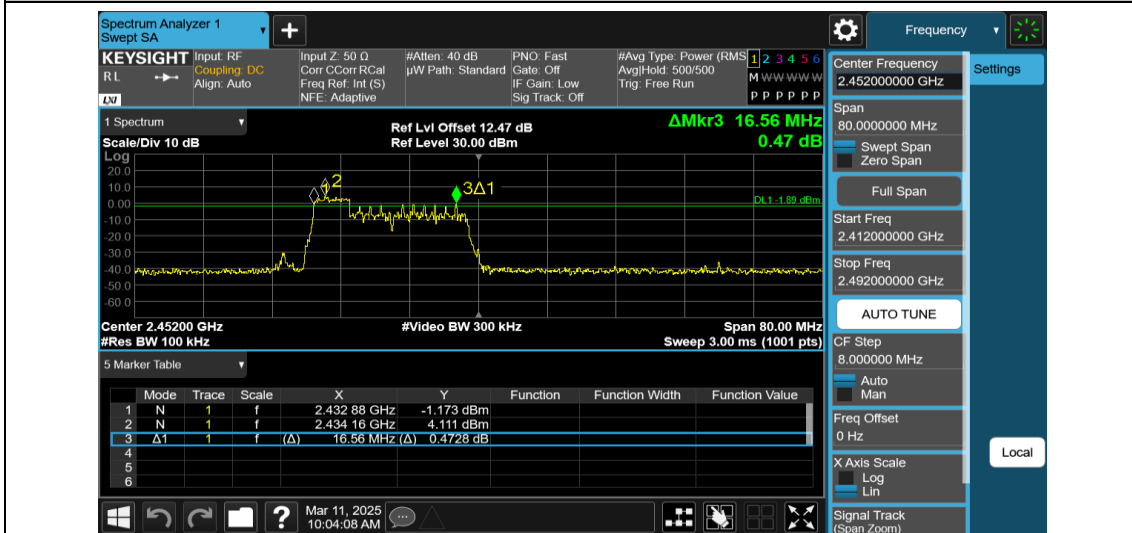
11AX40MIMO-Ant1-2452-52Tone-RU37-PASS
