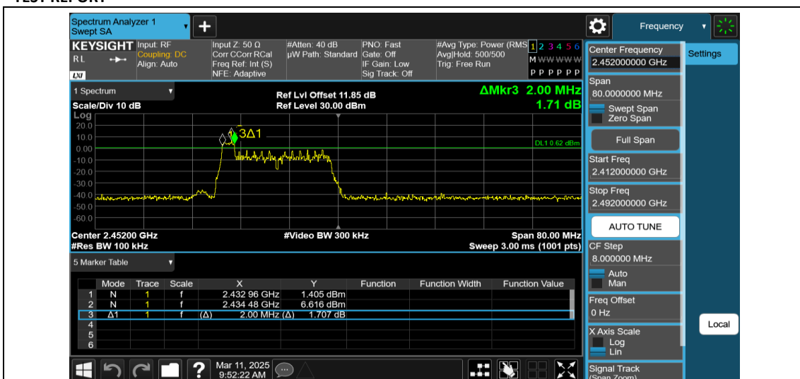
11AX40MIMO-Ant2-2452-26Tone-RU0-PASS
