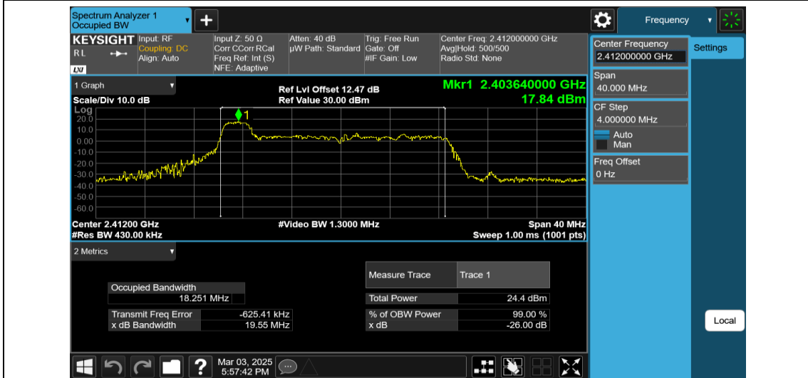
11AX20MIMO-Ant1-2412-26Tone-RU0
