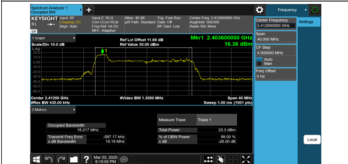
11AX20MIMO-Ant2-2412-26Tone-RU0
