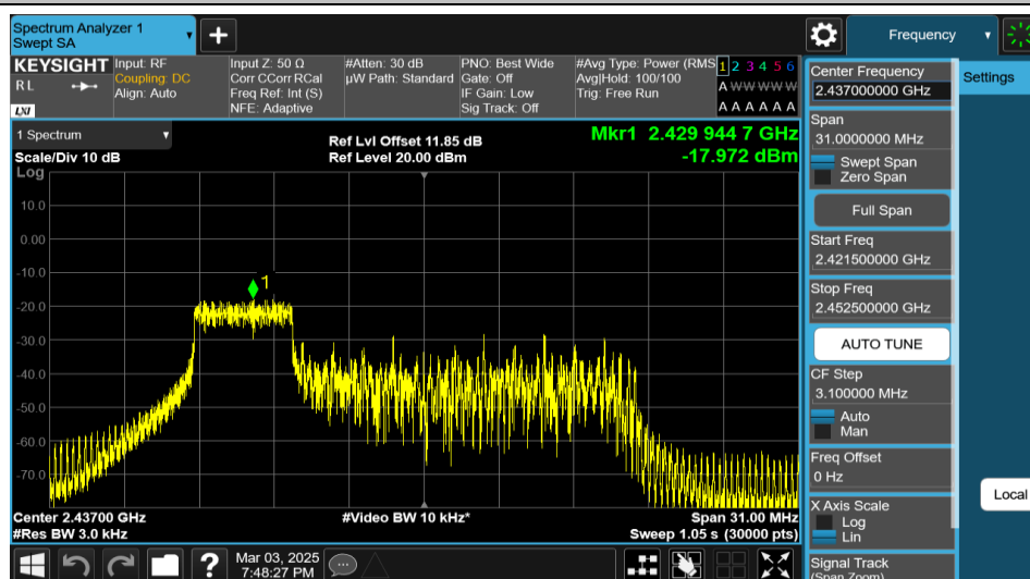
11AX20MIMO-Ant2-2437-52Tone-RU37-PASS
