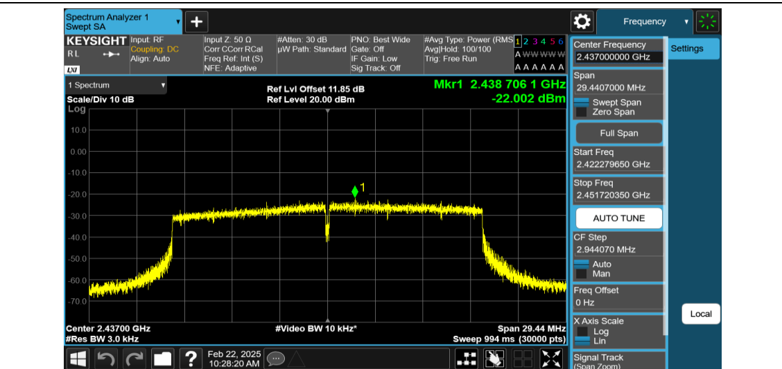
11AX20MIMO-Ant2-2437-PASS
