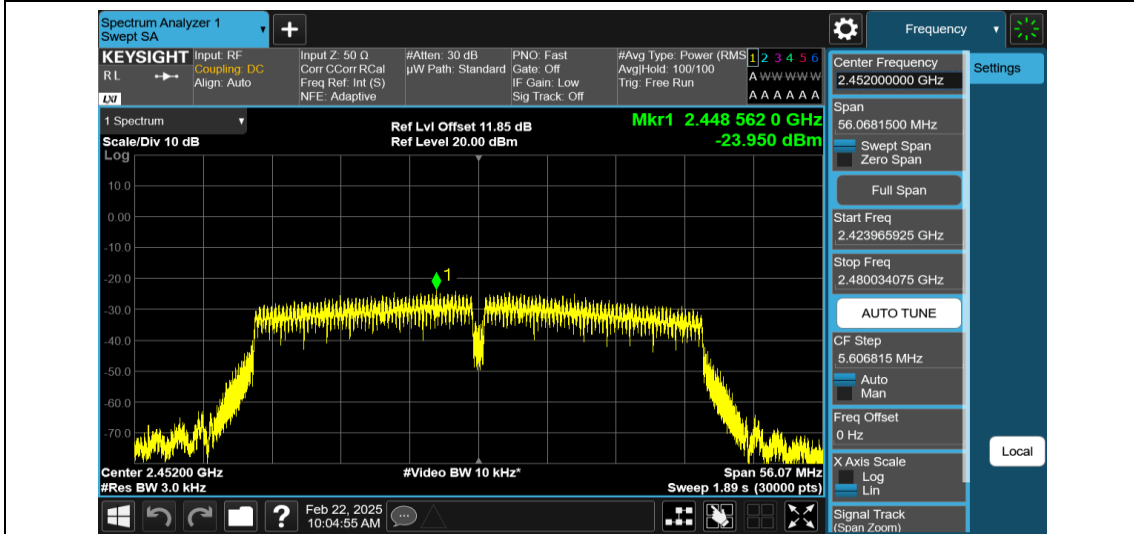
11N40MIMO-Ant2-2452-PASS
