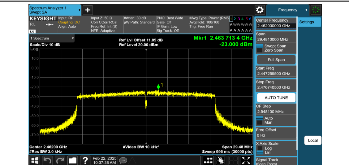
11AX20MIMO-Ant2-2462-PASS
