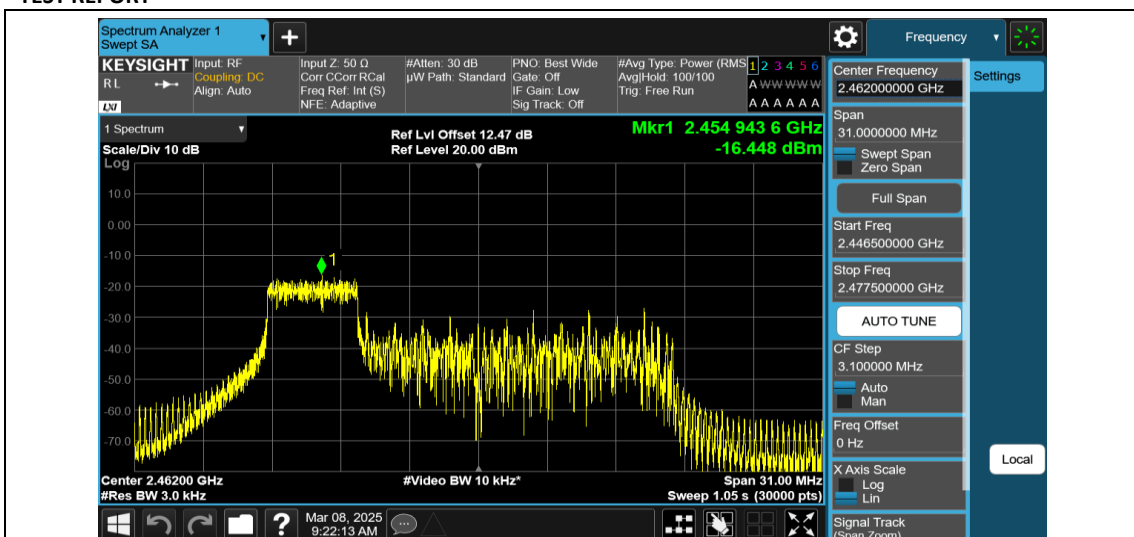
11AX20MIMO-Ant1-2462-52Tone-RU37-PASS
