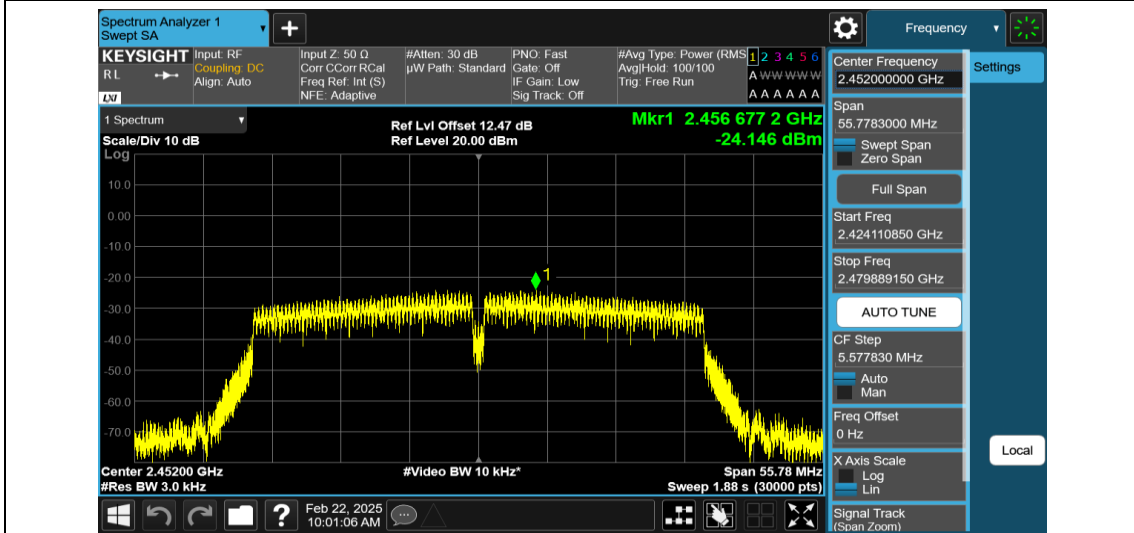
11N40MIMO-Ant1-2452-PASS
