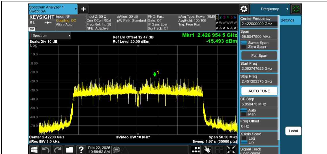
11AX40MIMO-Ant1-2422-PASS
