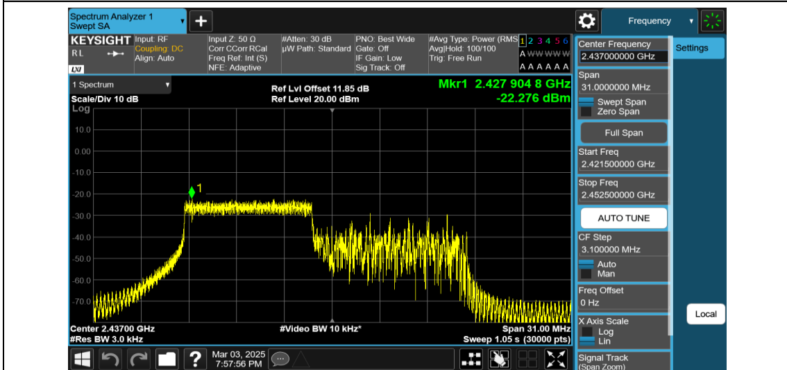
11AX20MIMO-Ant2-2437-106Tone-RU53-PASS
