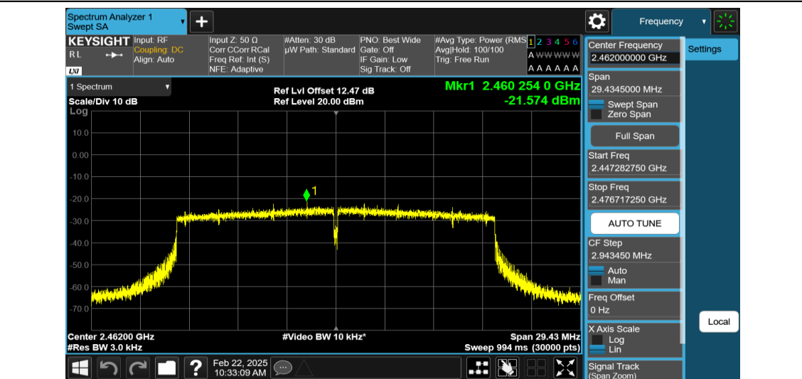
11AX20MIMO-Ant1-2462-PASS
