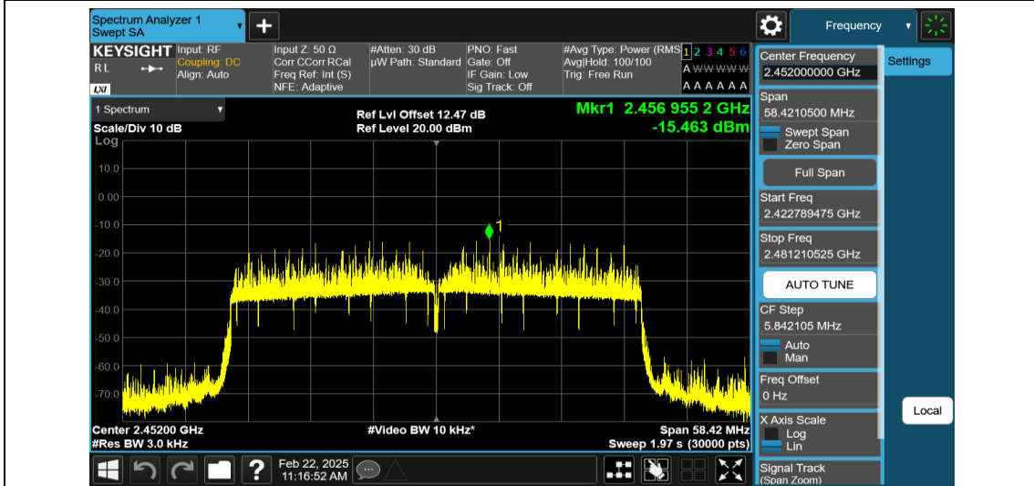
11AX40MIMO-Ant1-2452-PASS
