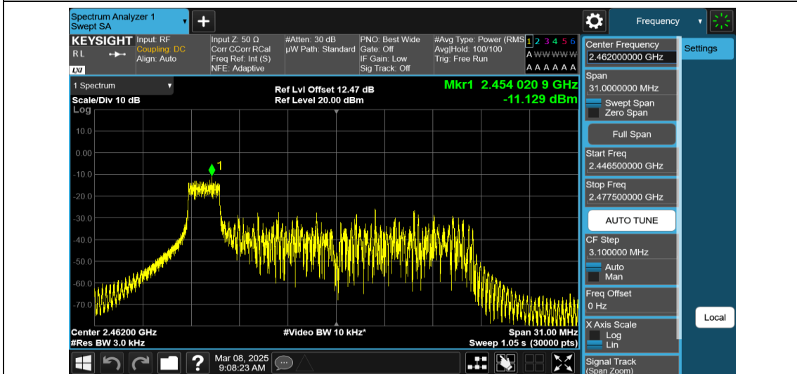
11AX20MIMO-Ant1-2462-26Tone-RU0-PASS
