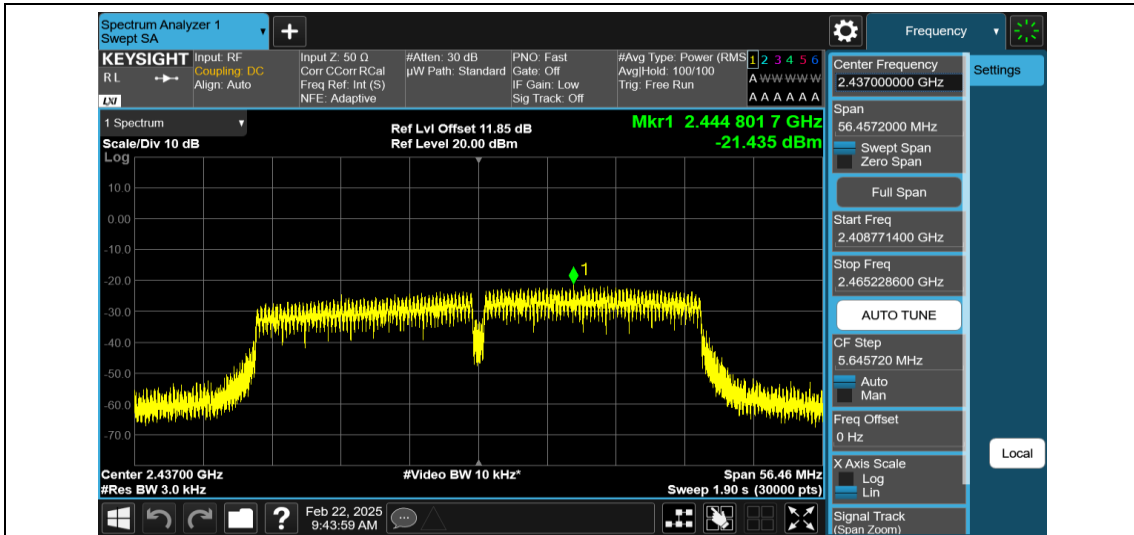
11N40MIMO-Ant2-2437-PASS
