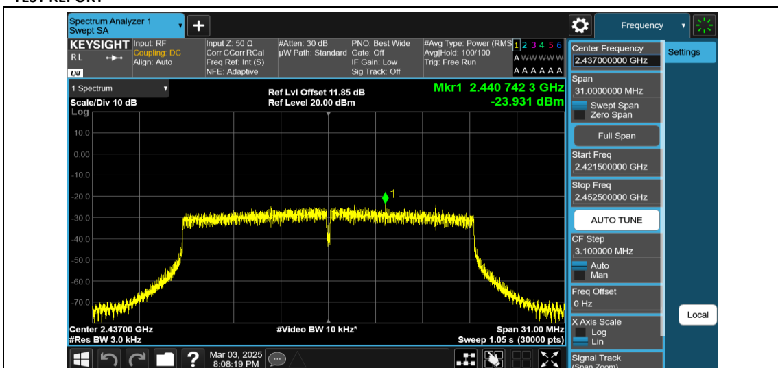
11AX20MIMO-Ant2-2437-242Tone-RU61-PASS
