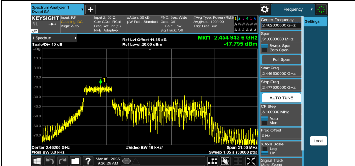
11AX20MIMO-Ant2-2462-52Tone-RU37-PASS
