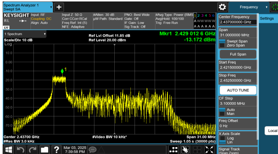
11AX20MIMO-Ant2-2437-26Tone-RU0-PASS
