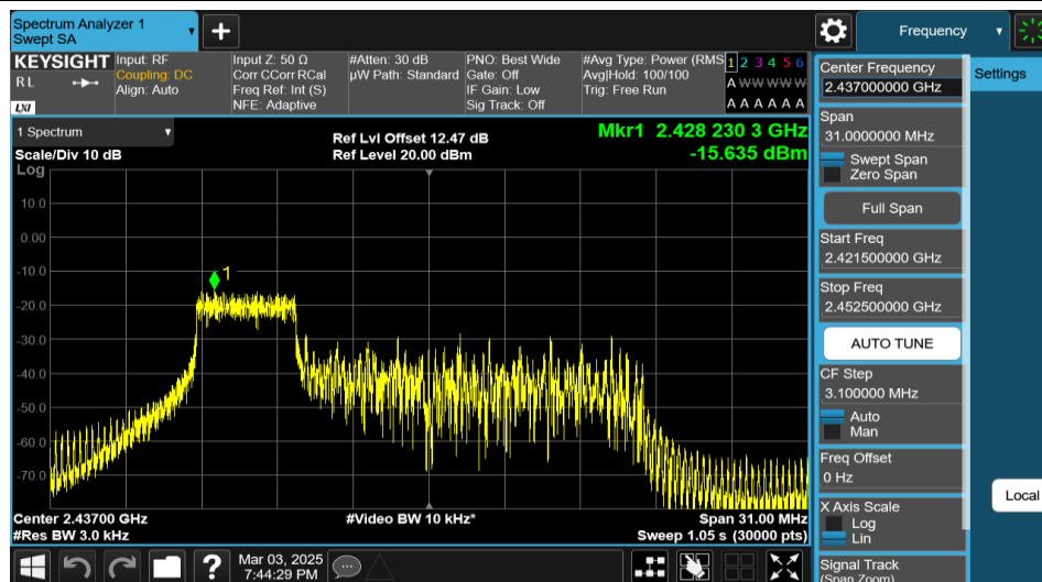
11AX20MIMO-Ant1-2437-52Tone-RU37-PASS
