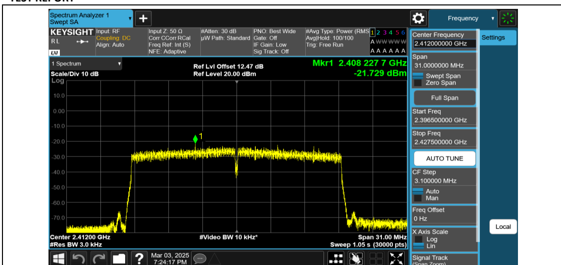
11AX20MIMO-Ant1-2412-242Tone-RU61-PASS
