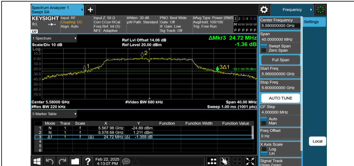
11A-Ant2-5580
