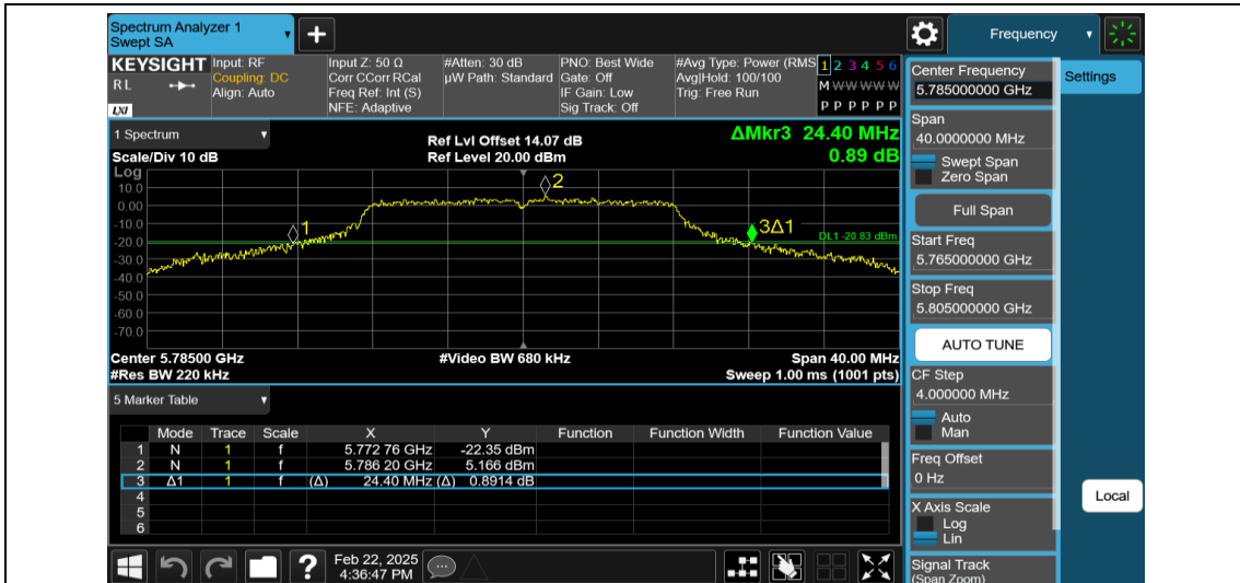
11A-Ant2-5785
