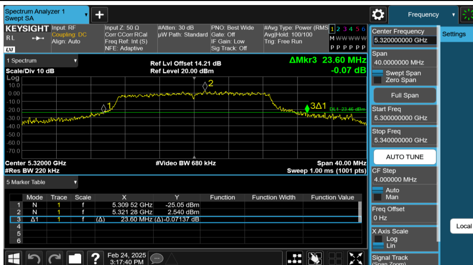
11N20MIMO-Ant2-5320
