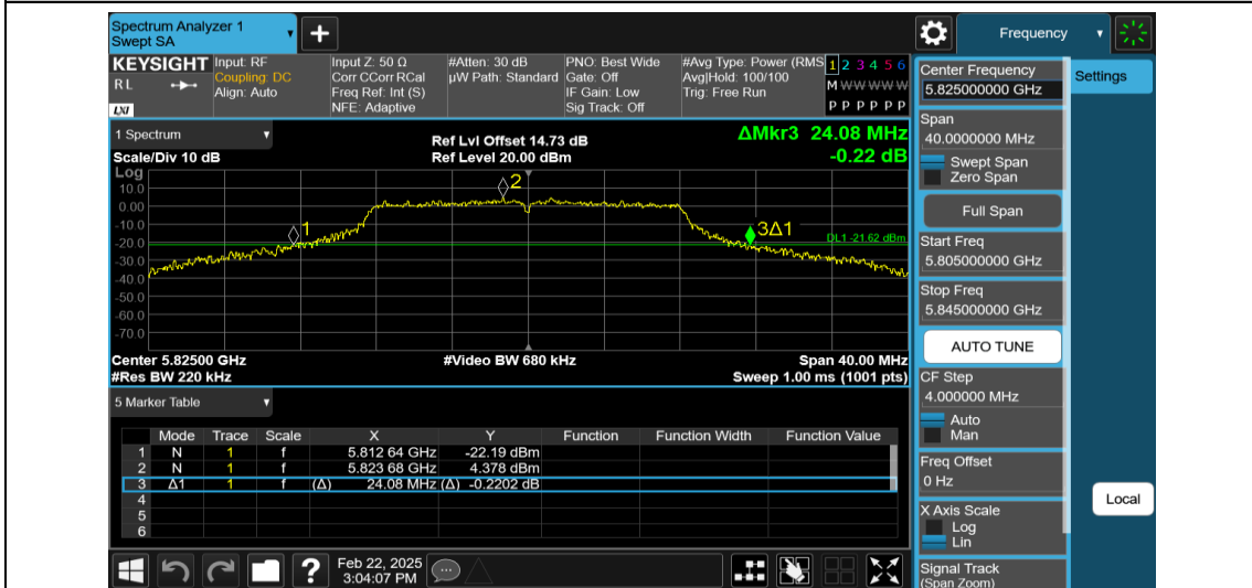
11A-Ant1-5825
