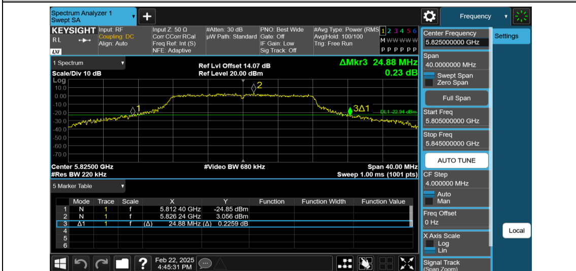
11A-Ant2-5825
