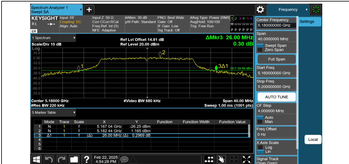
11N20MIMO-Ant1-5180
