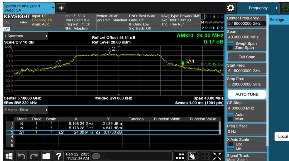
11A-Ant1-5180
