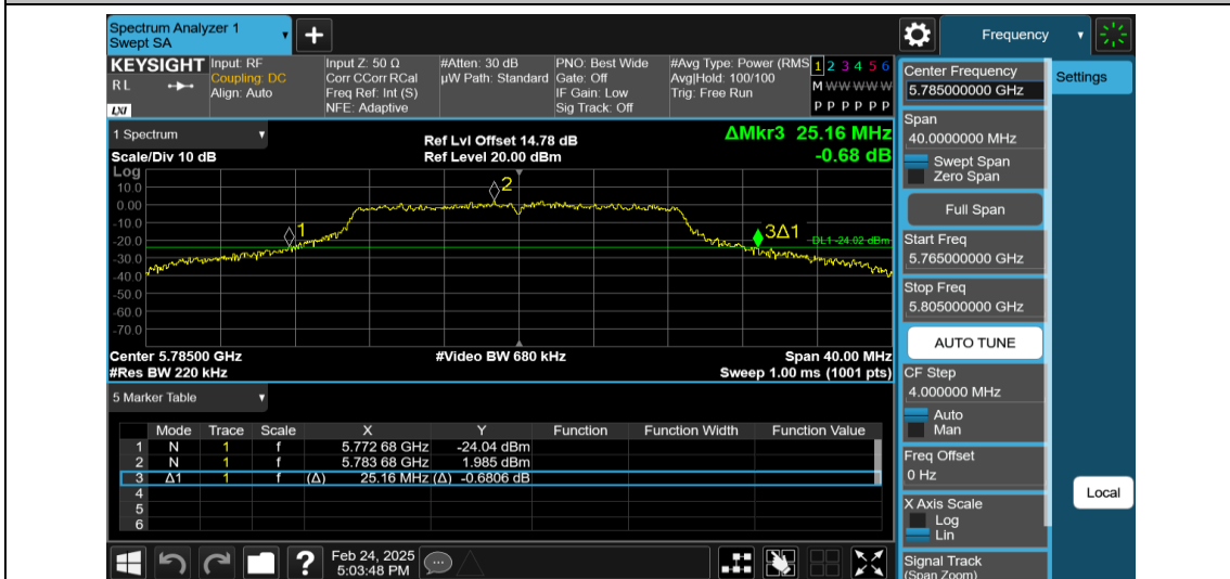
11N20MIMO-Ant1-5785
