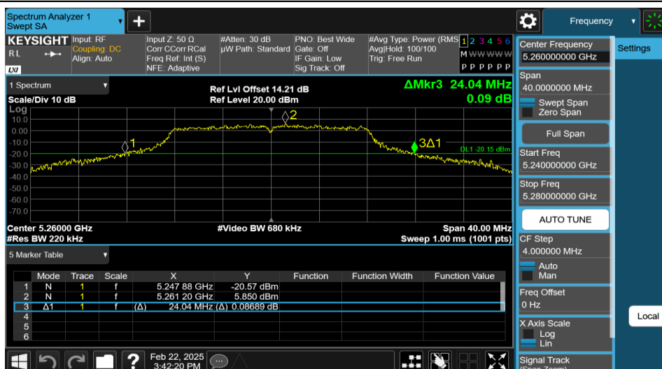
11A-Ant2-5260
