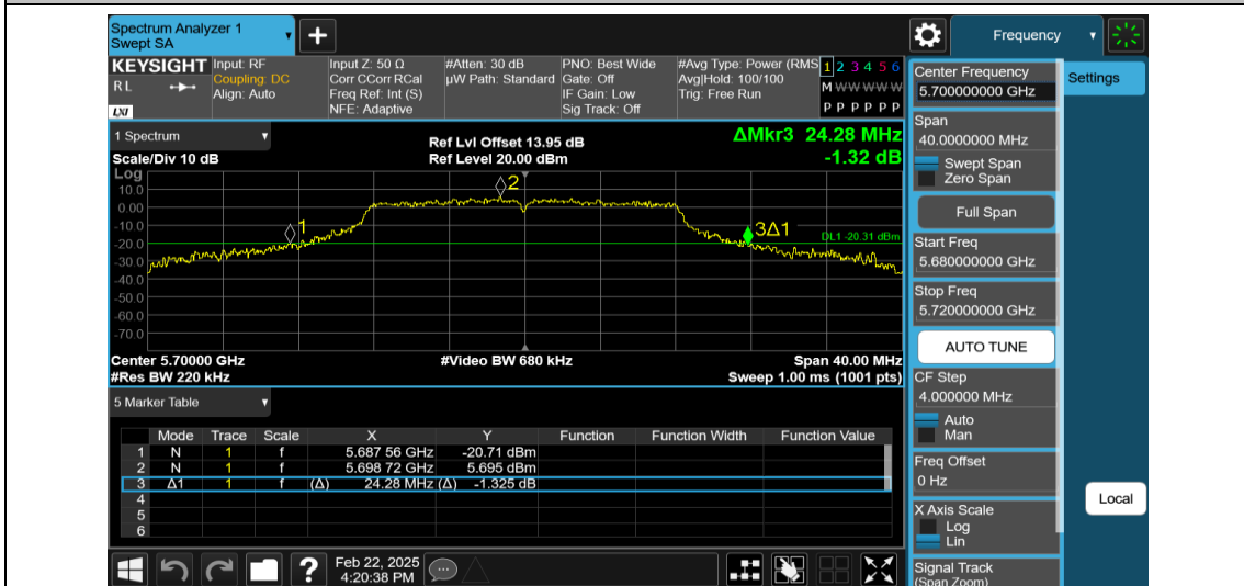
11A-Ant2-5700
