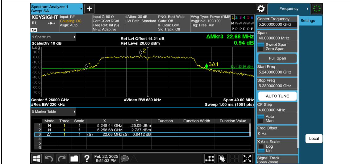
11N20MIMO-Ant2-5260
