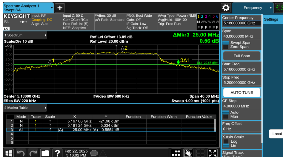
11A-Ant2-5180
