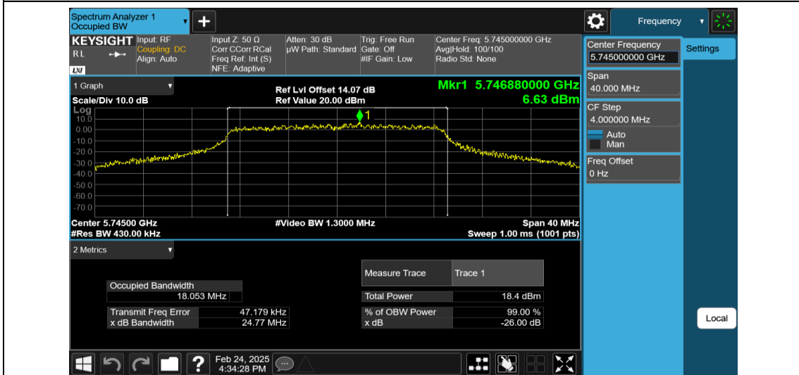
11N20MIMO-Ant2-5745
