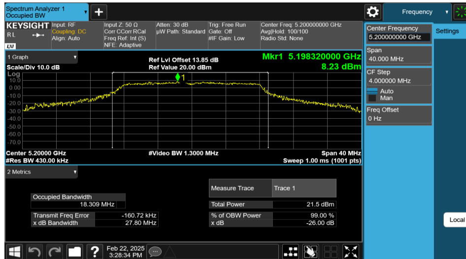
11A-Ant2-5200
