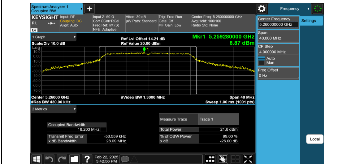
11A-Ant2-5260
