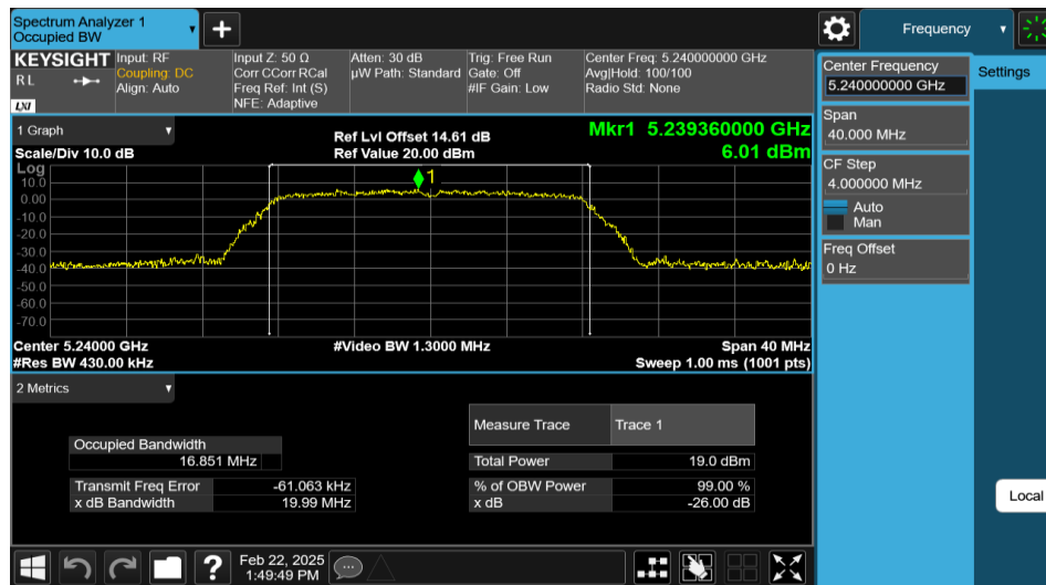
11A-Ant1-5240
