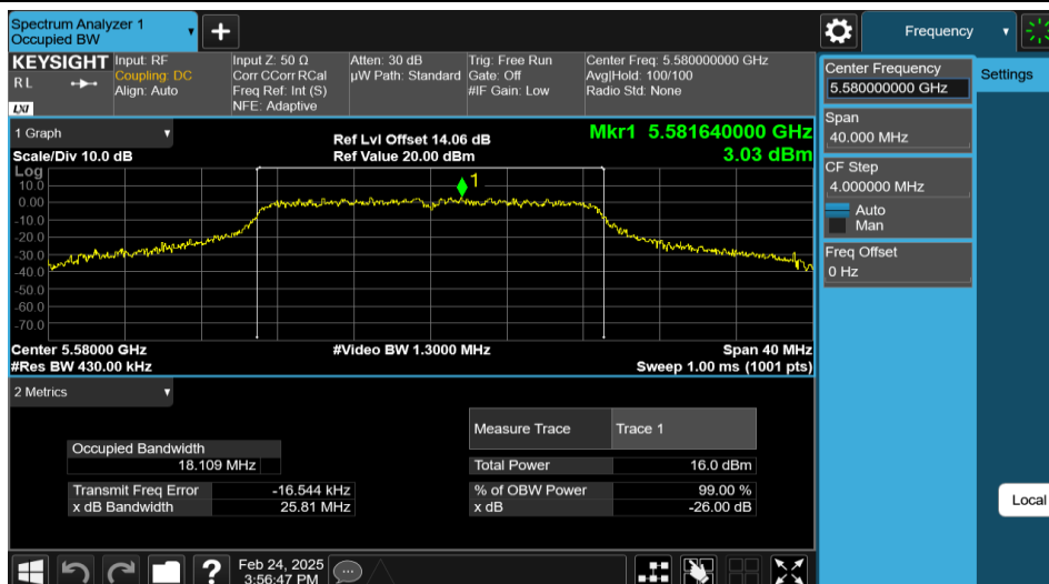
11N20MIMO-Ant2-5580
