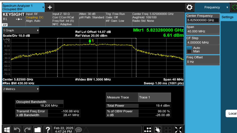
11A-Ant2-5825
