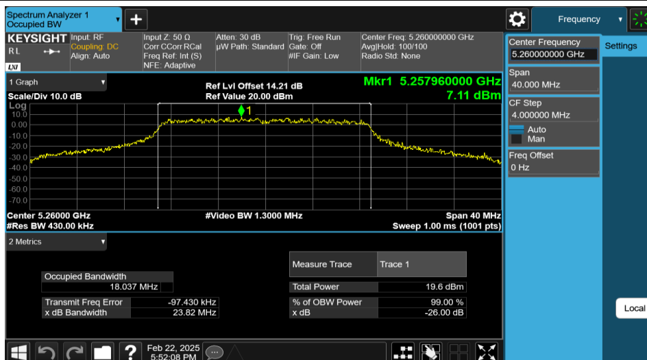
11N20MIMO-Ant2-5260
