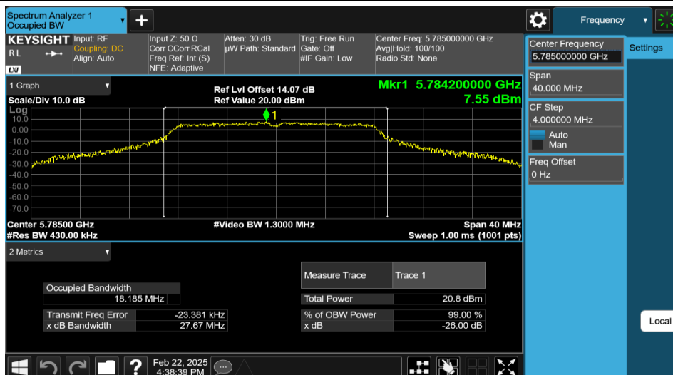
11A-Ant2-5785
