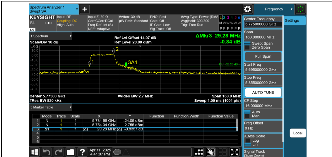
11AX80MIMO-Ant2-5775-242Tone-RU61
