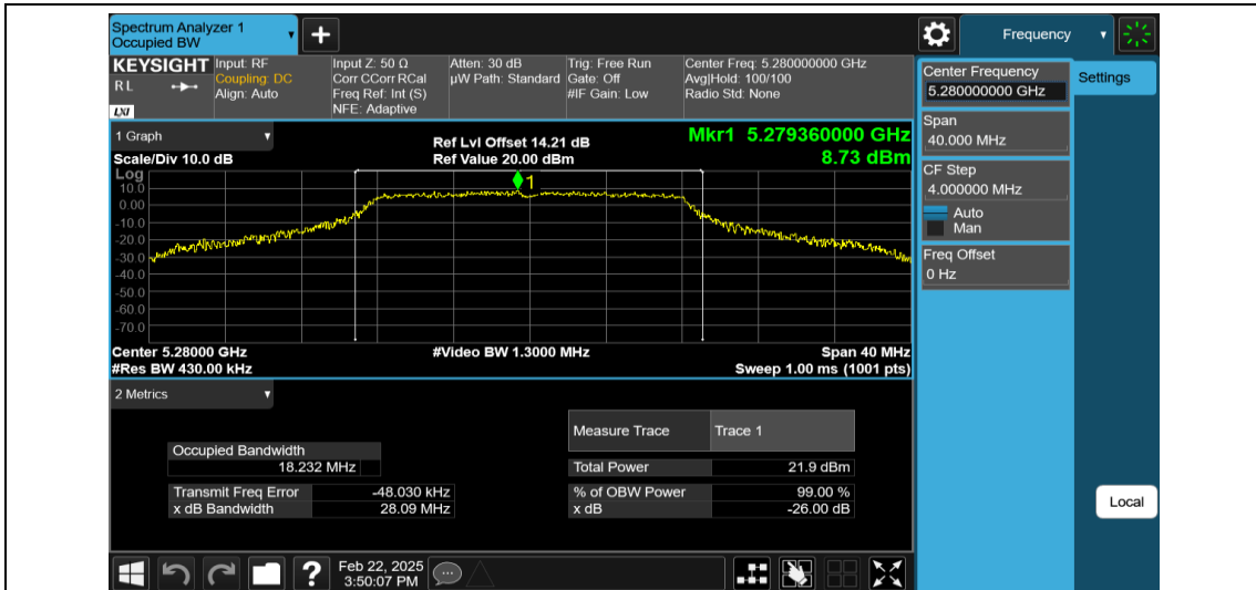
11A-Ant2-5280
