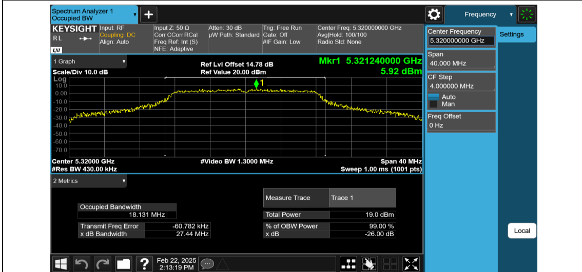
11A-Ant1-5320
