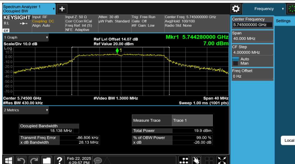
11A-Ant2-5745
