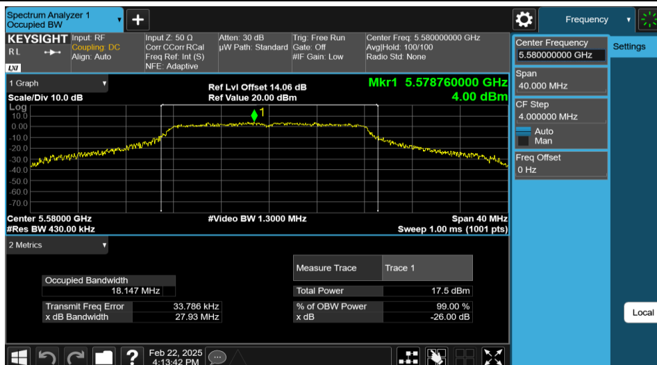
11A-Ant2-5580
