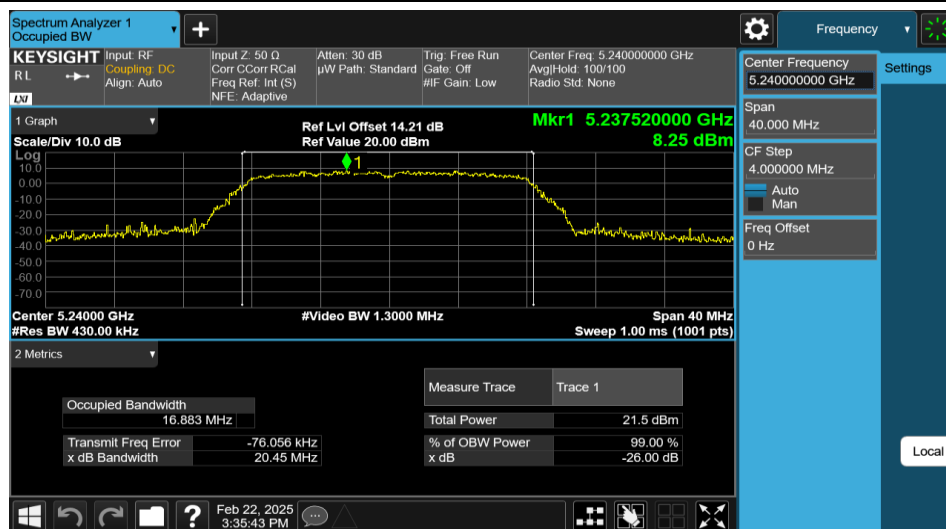
11A-Ant2-5240
