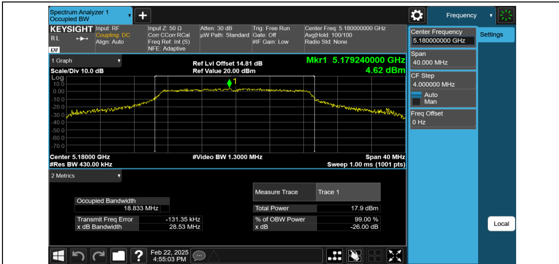
11N20MIMO-Ant1-5180
