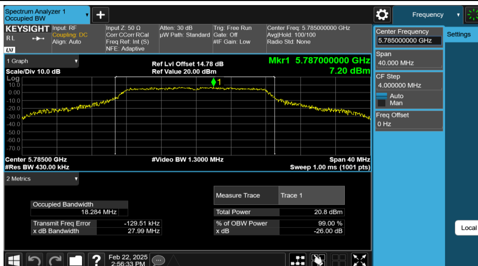
11A-Ant1-5785
