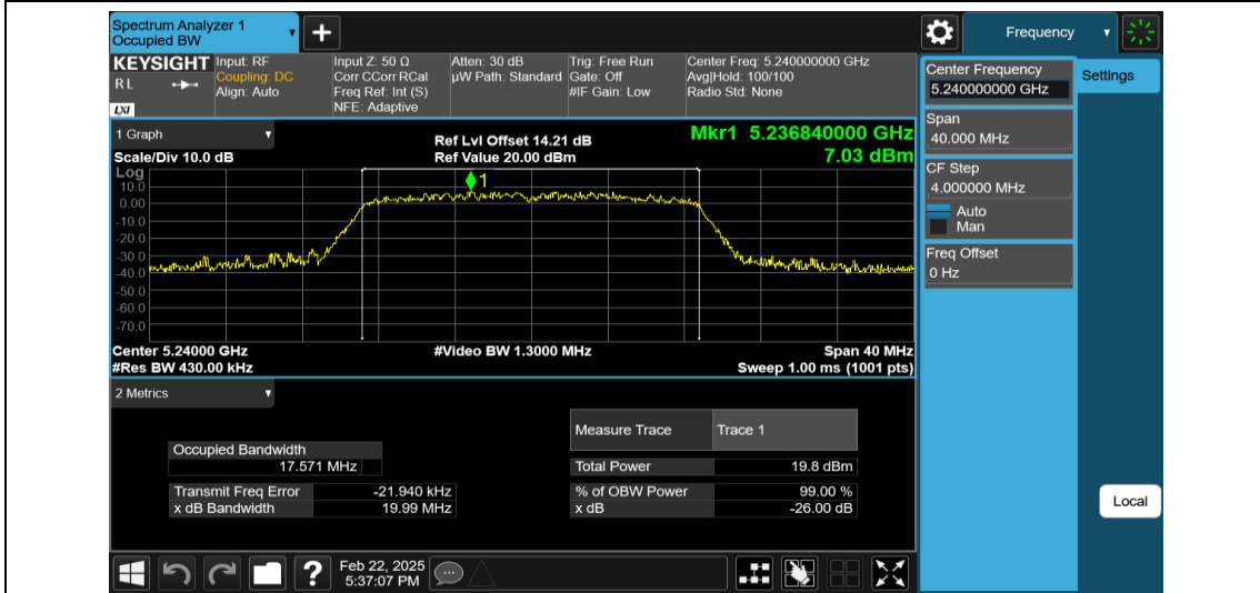
11N20MIMO-Ant2-5240
