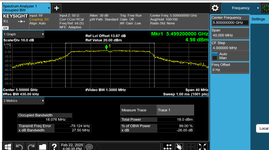
11A-Ant2-5500
