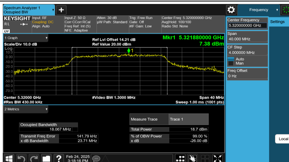
11N20MIMO-Ant2-5320
