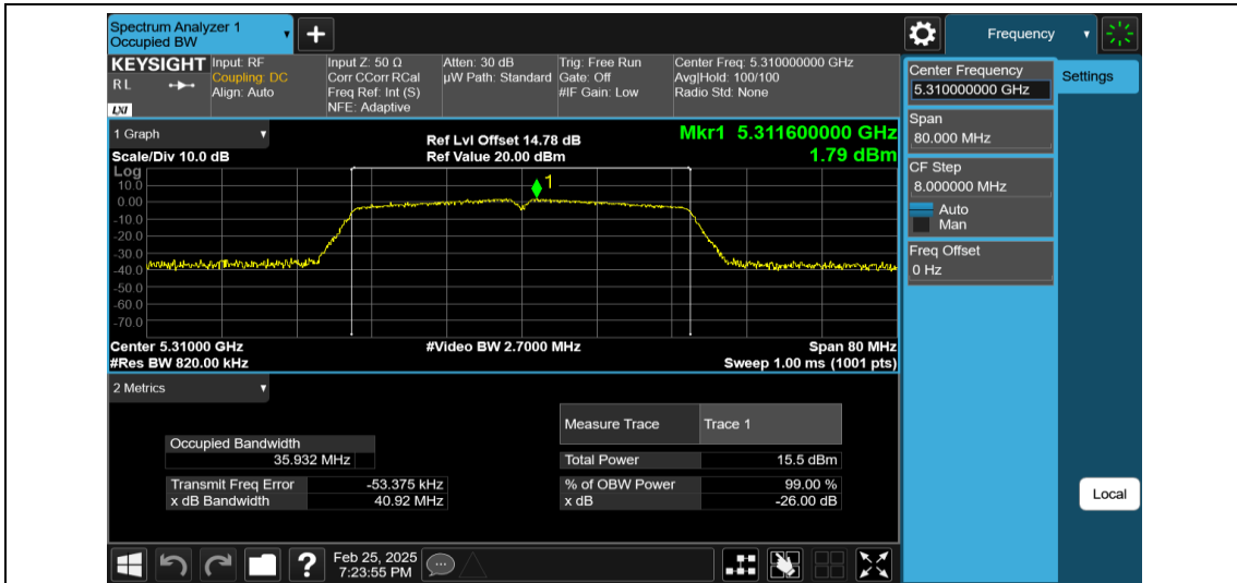
11AC40MIMO-Ant1-5310
