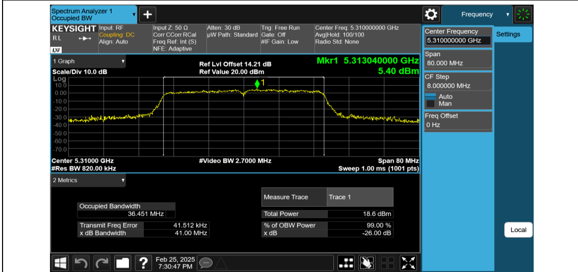
11AC40MIMO-Ant2-5310
