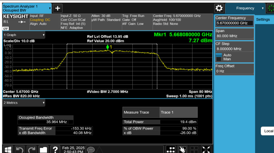
11N40MIMO-Ant2-5670
