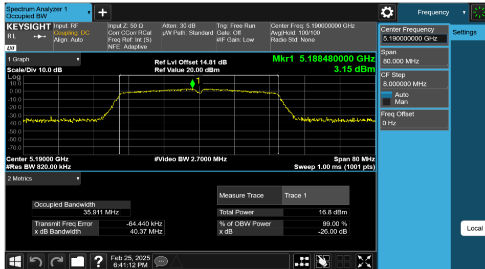
11AC40MIMO-Ant1-5190
