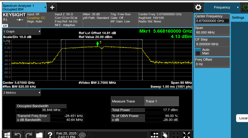
11N40MIMO-Ant1-5670
