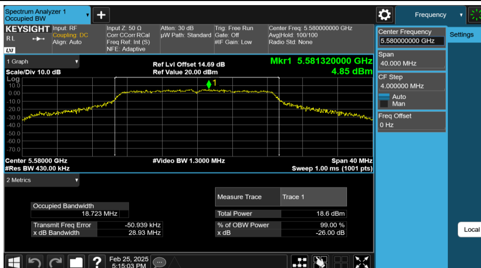
11AC20MIMO-Ant1-5580
