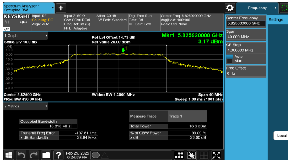
11AC20MIMO-Ant1-5825
