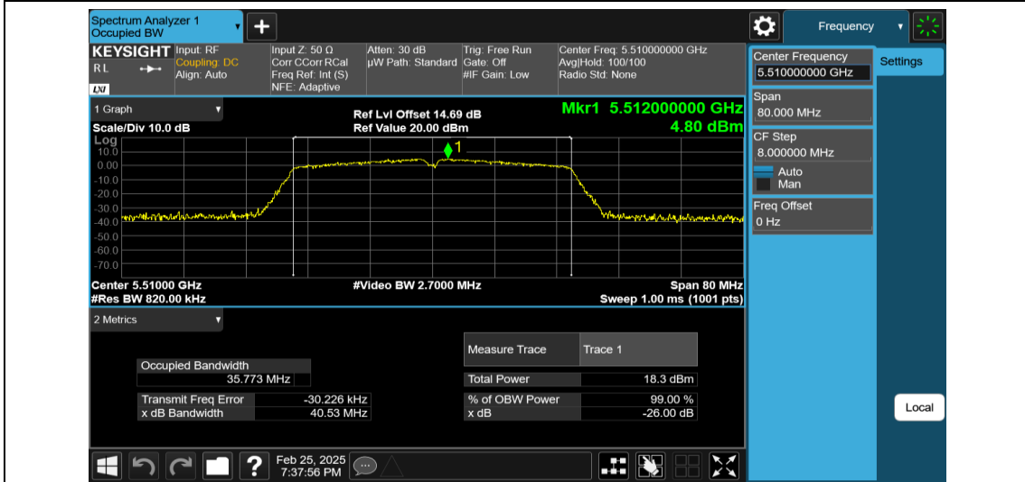
11AC40MIMO-Ant1-5510
