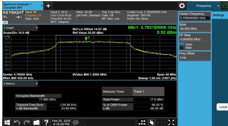
11AC20MIMO-Ant2-5785
