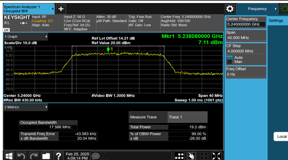
11AC20MIMO-Ant2-5240
