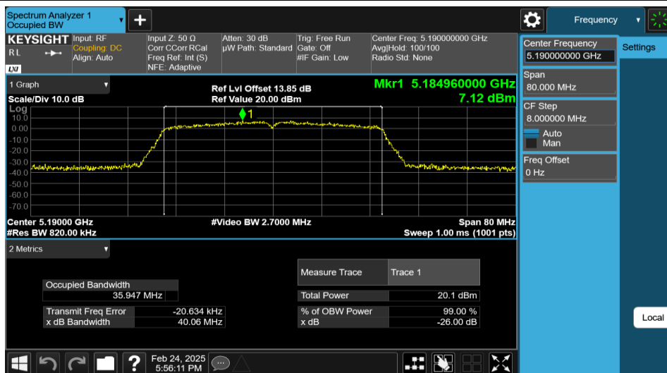
11N40MIMO-Ant2-5190
