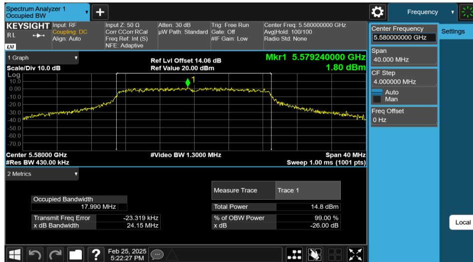
11AC20MIMO-Ant2-5580
