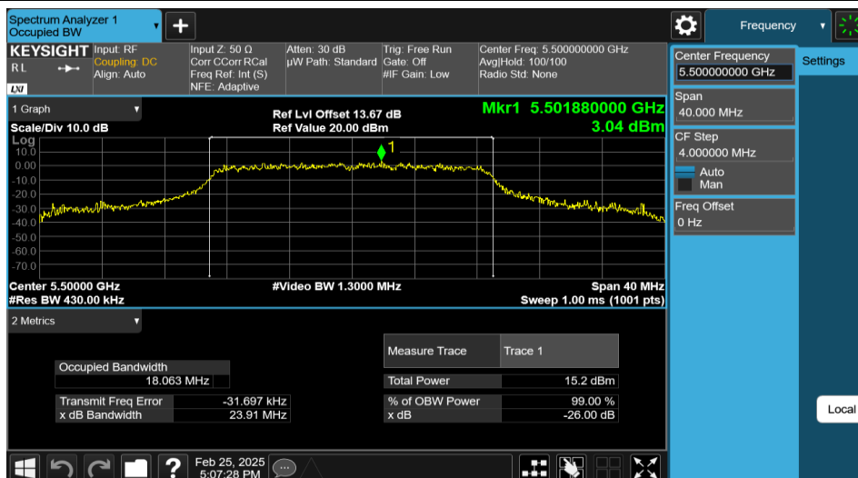
11AC20MIMO-Ant2-5500
