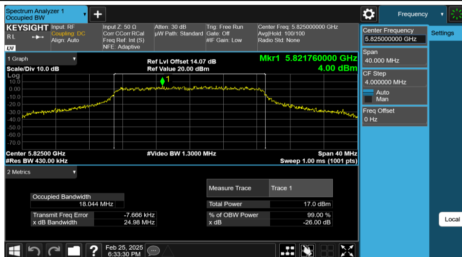
11AC20MIMO-Ant2-5825
