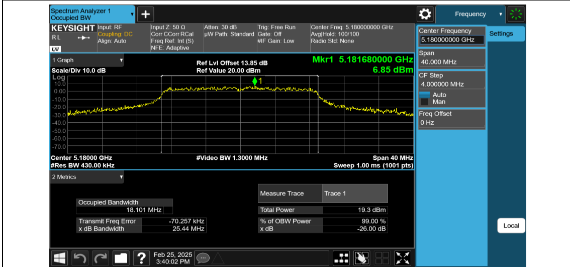
11AC20MIMO-Ant2-5180
