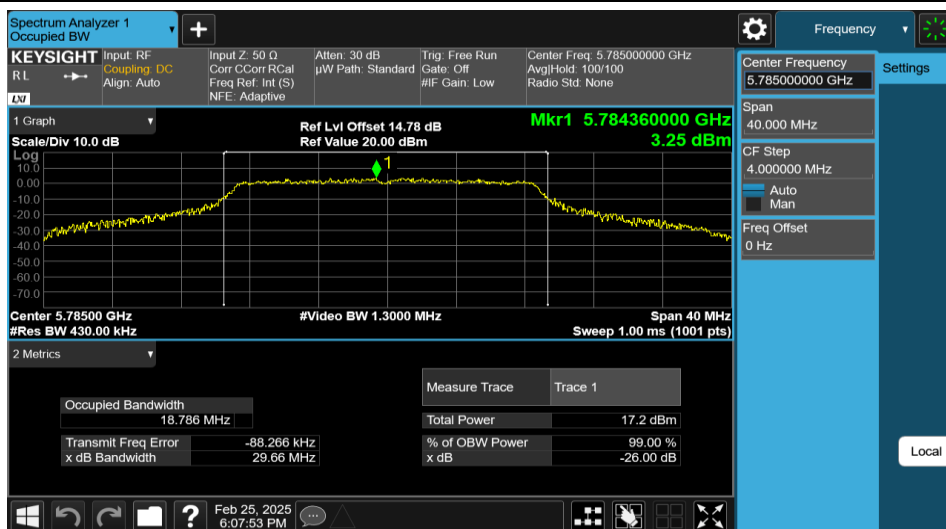
11AC20MIMO-Ant1-5785
