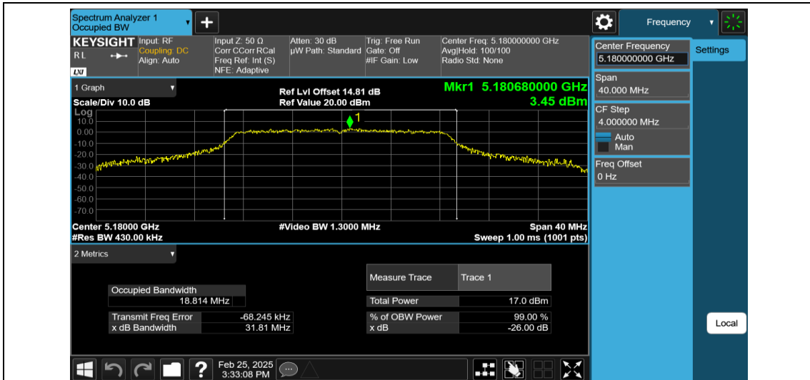
11AC20MIMO-Ant1-5180
