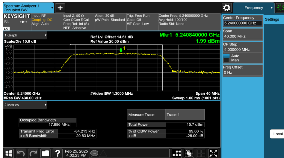
11AC20MIMO-Ant1-5240
