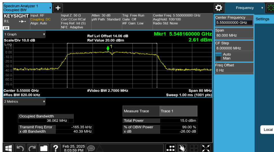
11AC40MIMO-Ant2-5550
