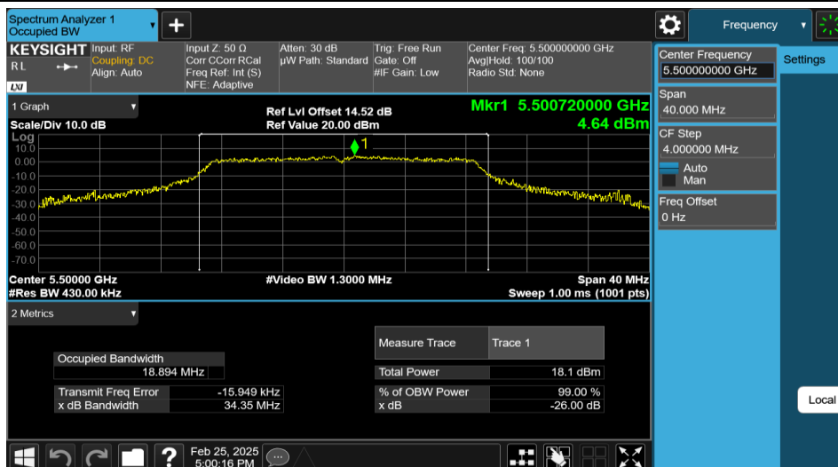
11AC20MIMO-Ant1-5500
