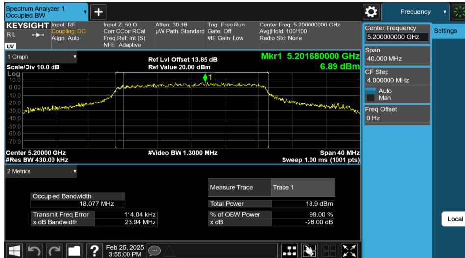
11AC20MIMO-Ant2-5200
