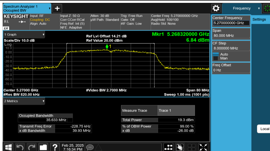
11AC40MIMO-Ant2-5270
