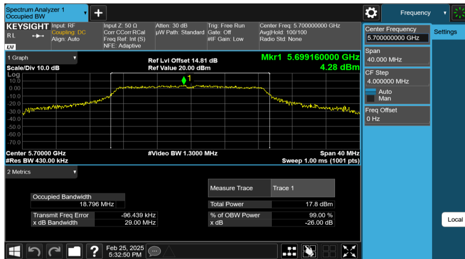
11AC20MIMO-Ant1-5700
