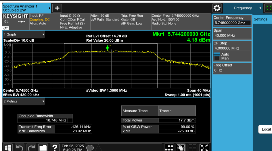
11AC20MIMO-Ant1-5745
