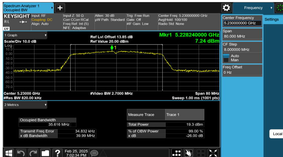
11AC40MIMO-Ant2-5230
