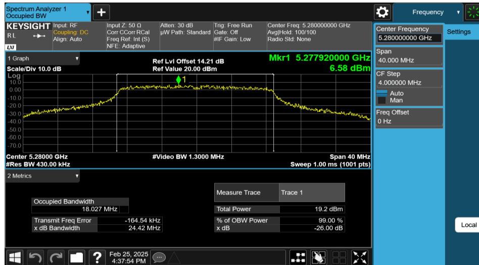
11AC20MIMO-Ant2-5280
