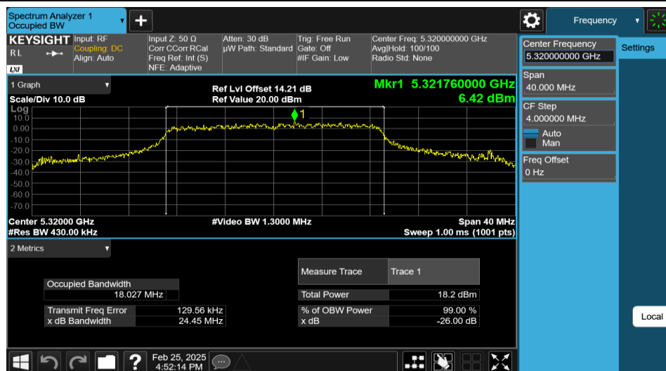
11AC20MIMO-Ant2-5320
