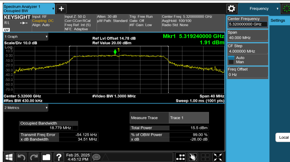
11AC20MIMO-Ant1-5320
