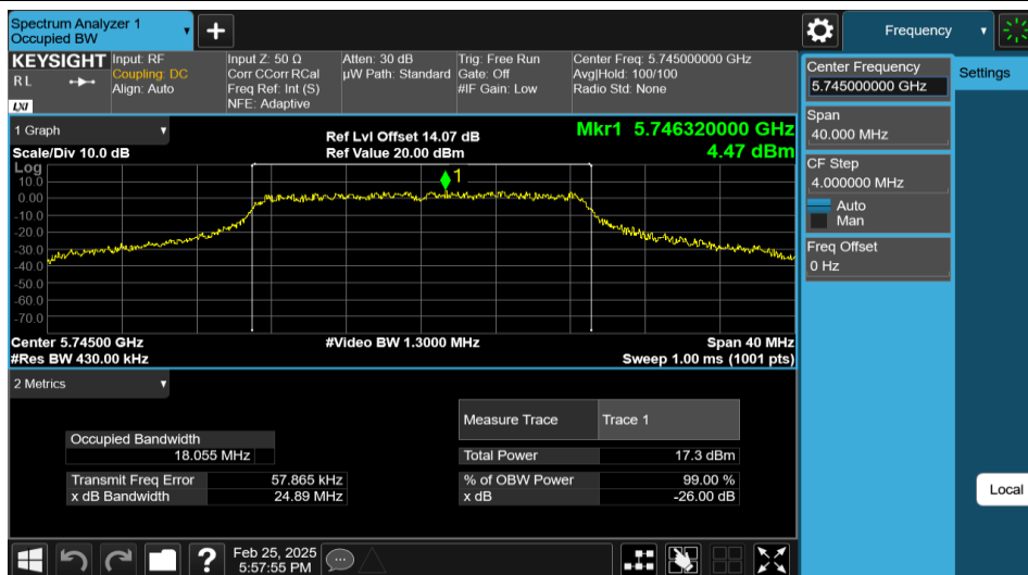
11AC20MIMO-Ant2-5745
