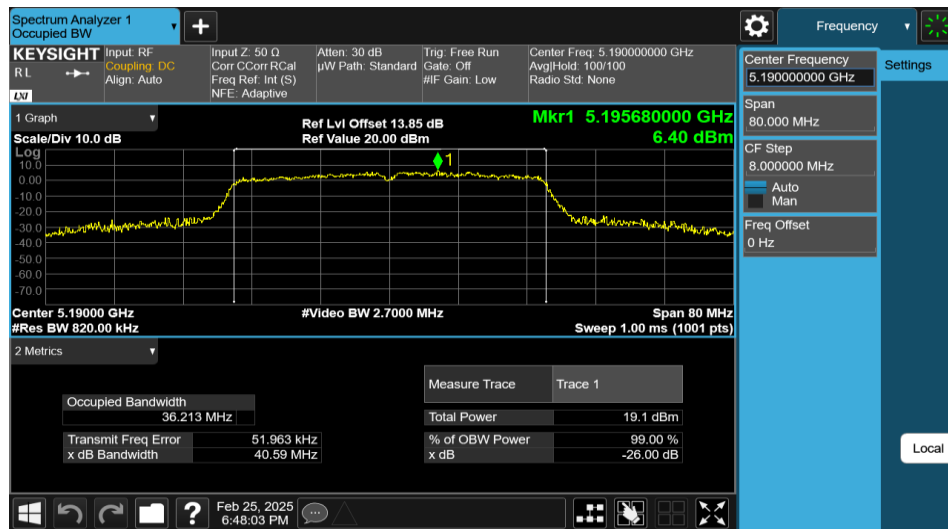
11AC40MIMO-Ant2-5190
