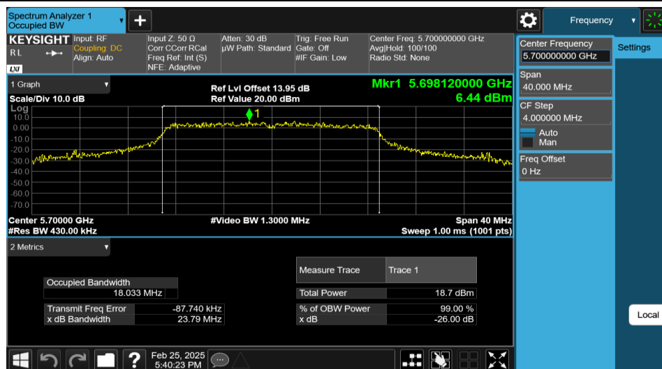
11AC20MIMO-Ant2-5700
