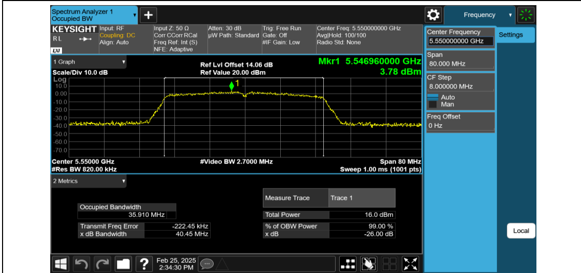
11N40MIMO-Ant2-5550
