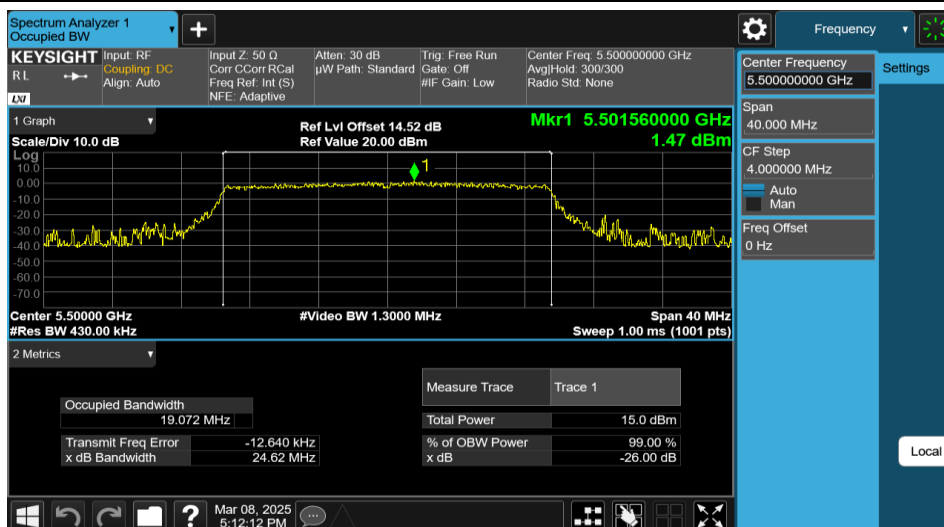
11AX20MIMO-Ant1-5500-242Tone-RU61
