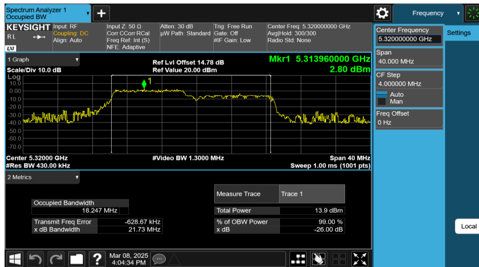
11AX20MIMO-Ant1-5320-106Tone-RU53
