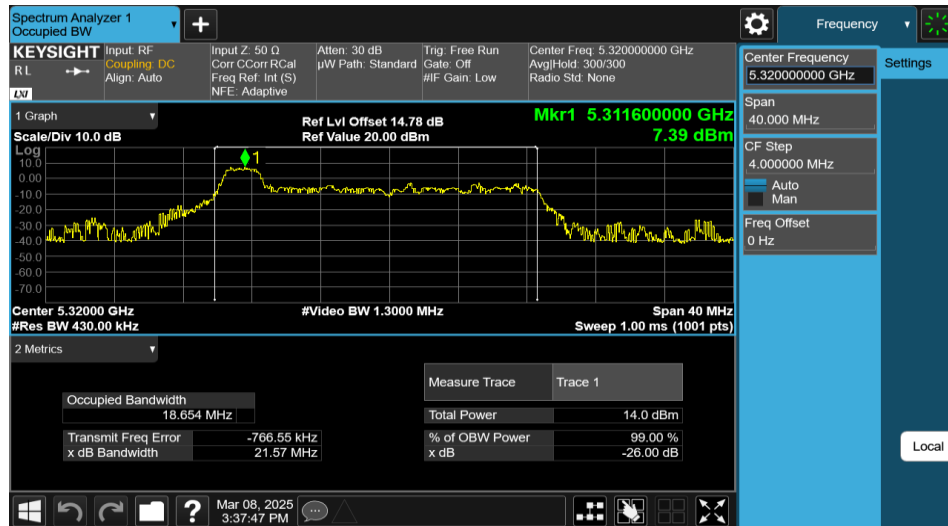
11AX20MIMO-Ant1-5320-26Tone-RU0
