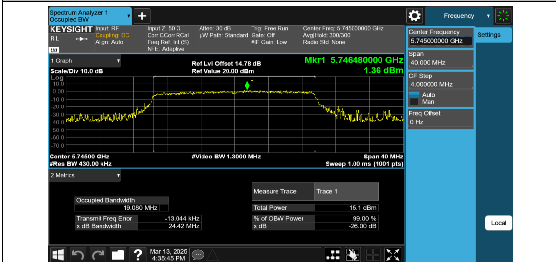
11AX20MIMO-Ant1-5745-242Tone-RU61
