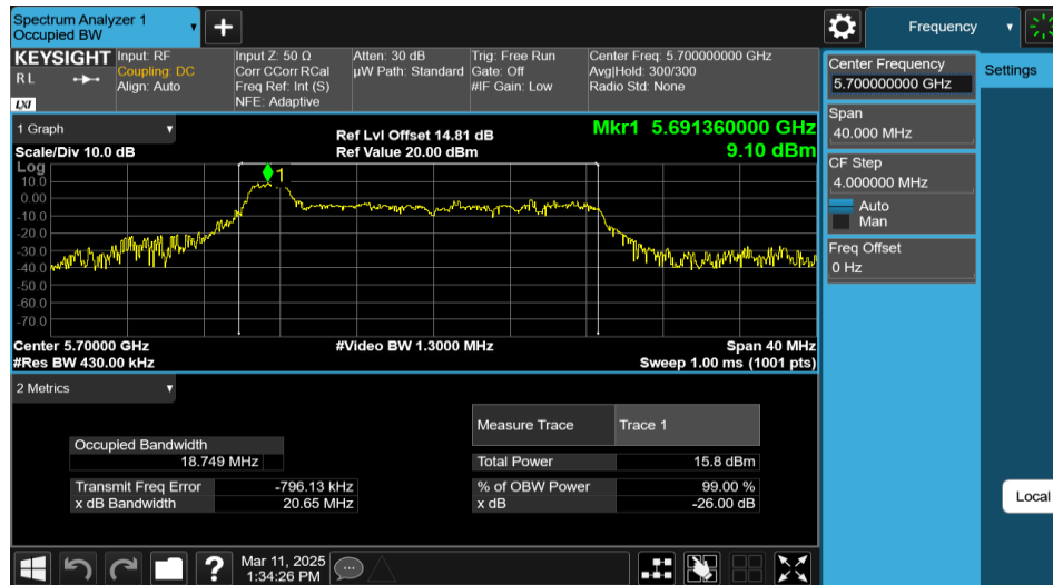
11AX20MIMO-Ant1-5700-26Tone-RU0
