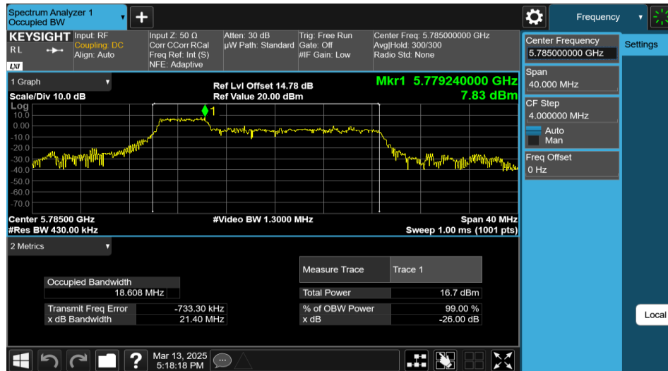
11AX20MIMO-Ant1-5785-52Tone-RU37
