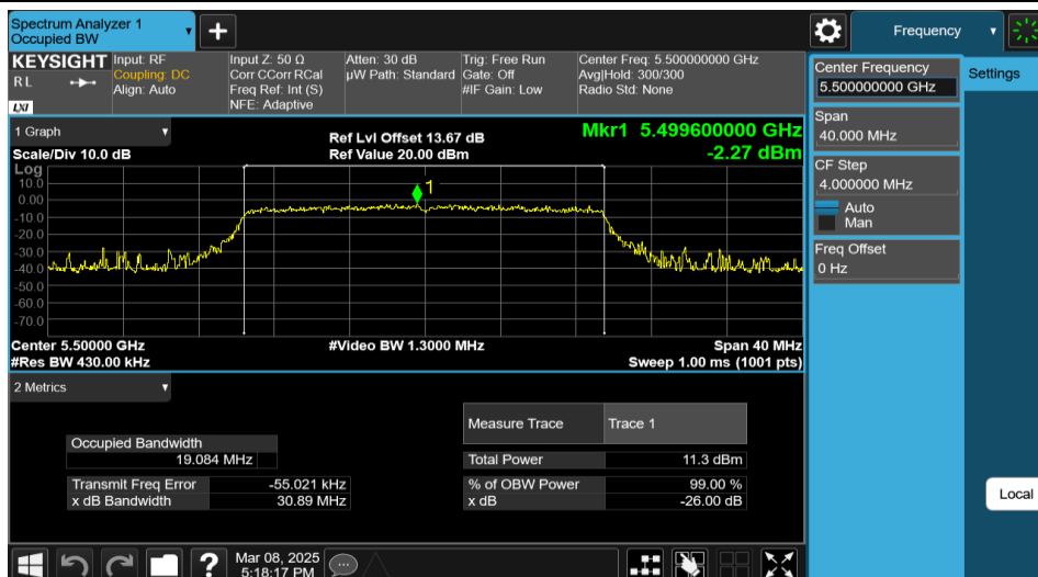
11AX20MIMO-Ant2-5500-242Tone-RU61
