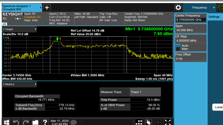
11AX20MIMO-Ant1-5745-26Tone-RU0
