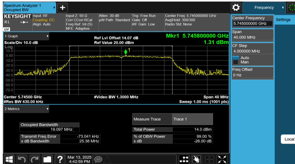
11AX20MIMO-Ant2-5745-242Tone-RU61
