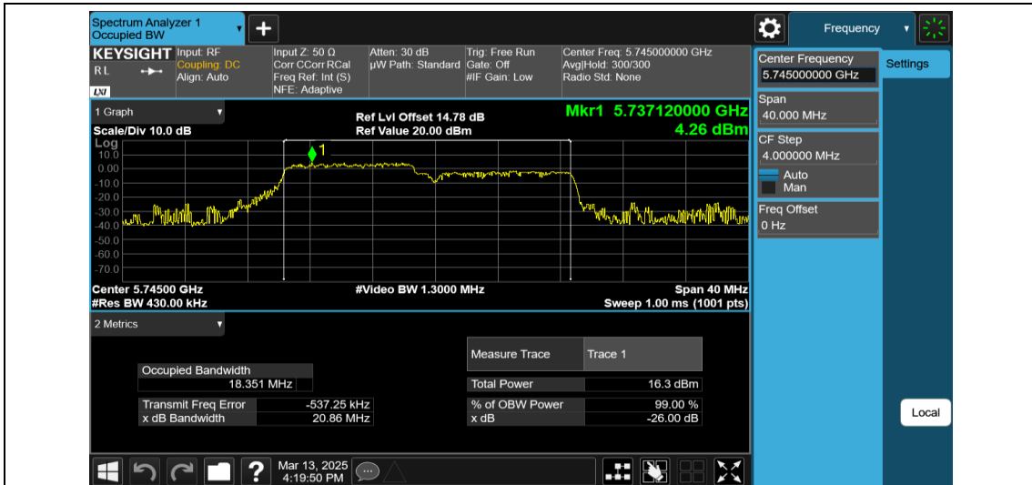
11AX20MIMO-Ant1-5745-106Tone-RU53
