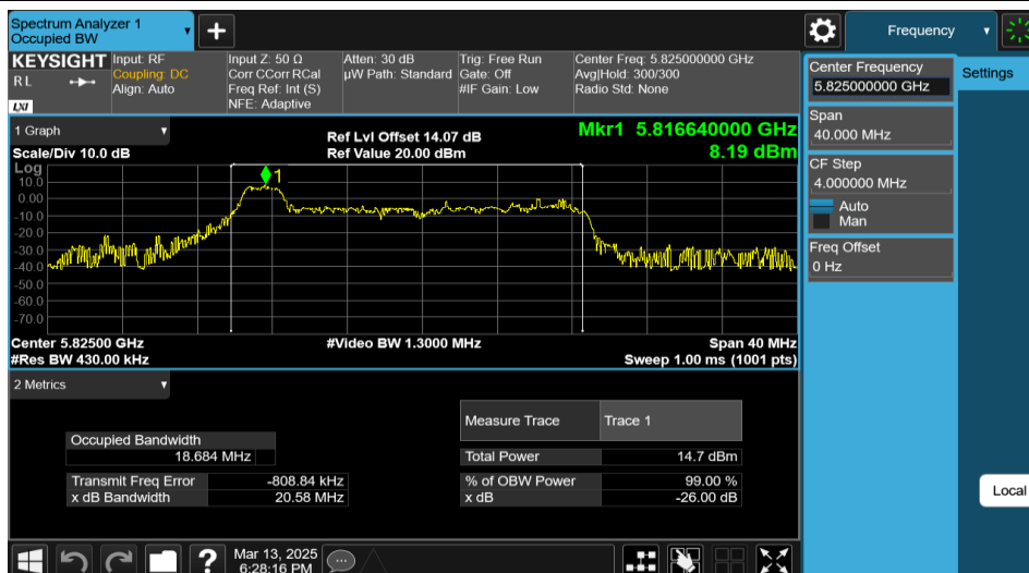
11AX20MIMO-Ant2-5825-26Tone-RU0
