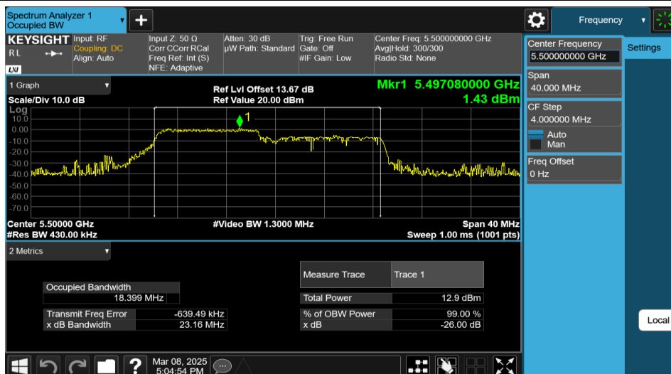
11AX20MIMO-Ant2-5500-106Tone-RU53
