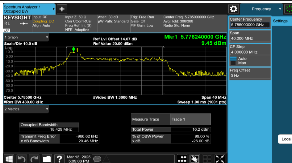
11AX20MIMO-Ant2-5785-26Tone-RU0
