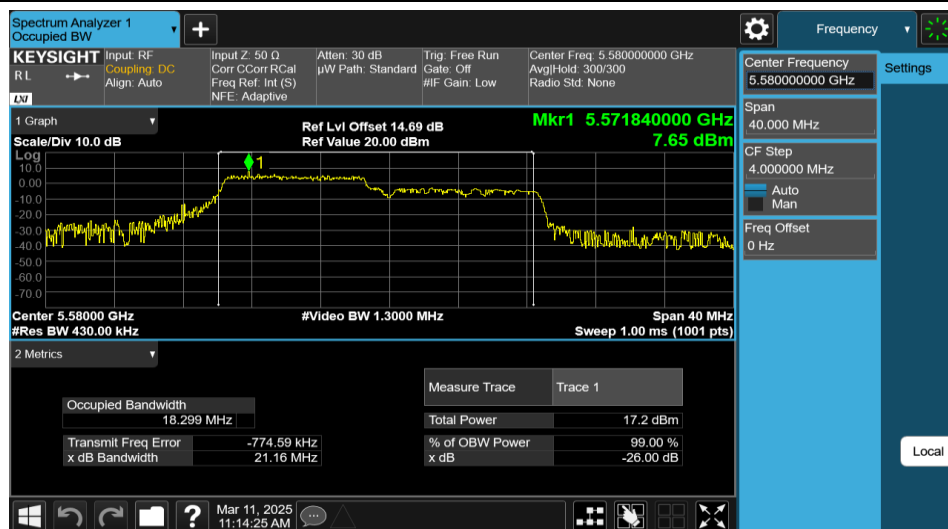
11AX20MIMO-Ant1-5580-106Tone-RU53
