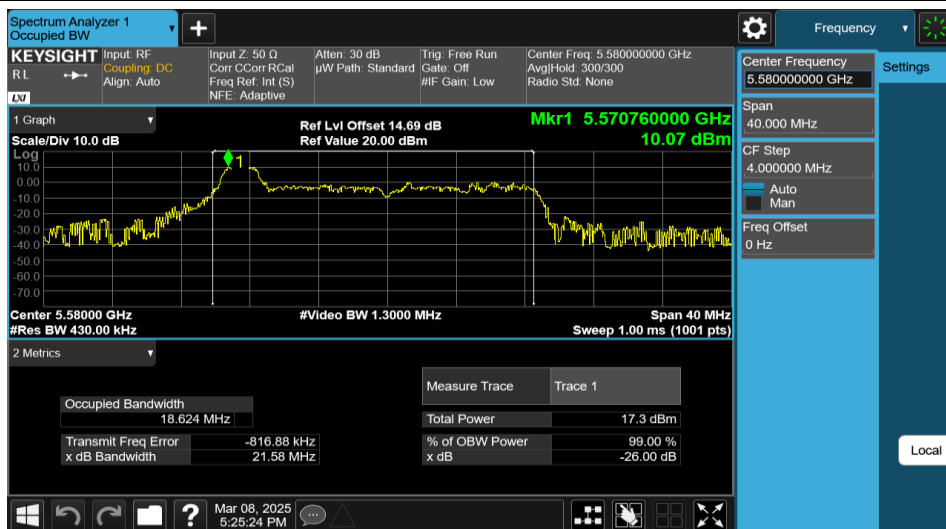
11AX20MIMO-Ant1-5580-26Tone-RU0
