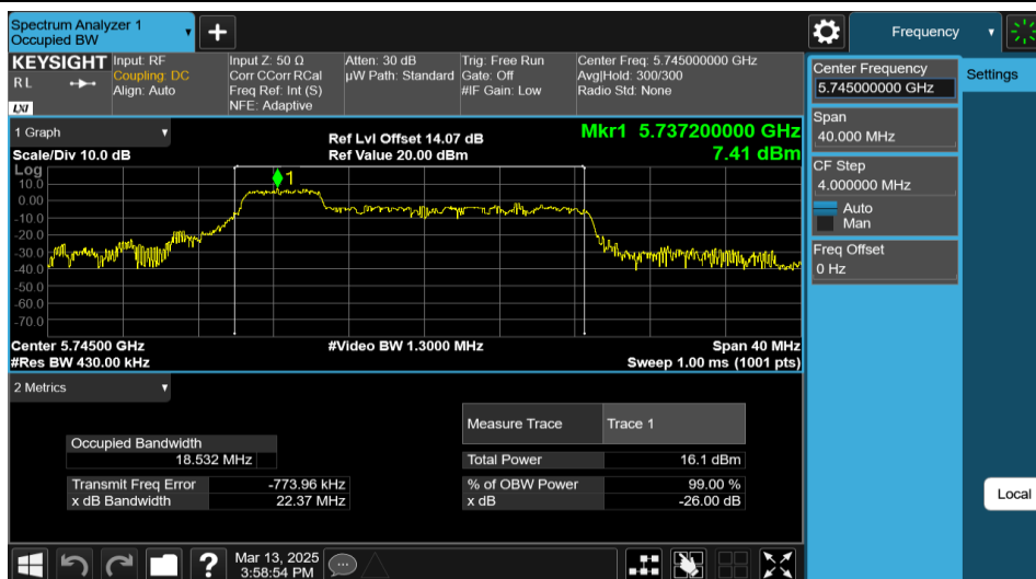
11AX20MIMO-Ant2-5745-52Tone-RU37
