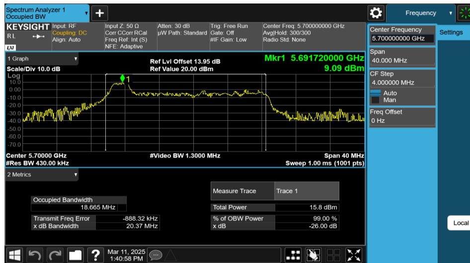
11AX20MIMO-Ant2-5700-26Tone-RU0
