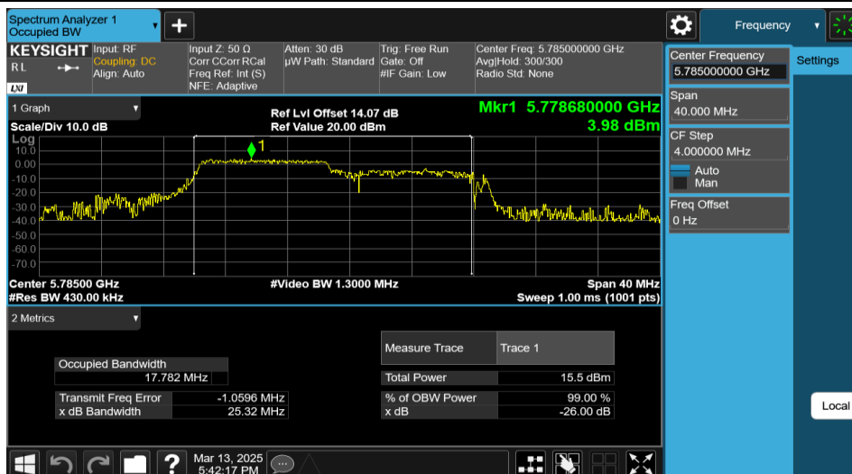
11AX20MIMO-Ant2-5785-106Tone-RU53
