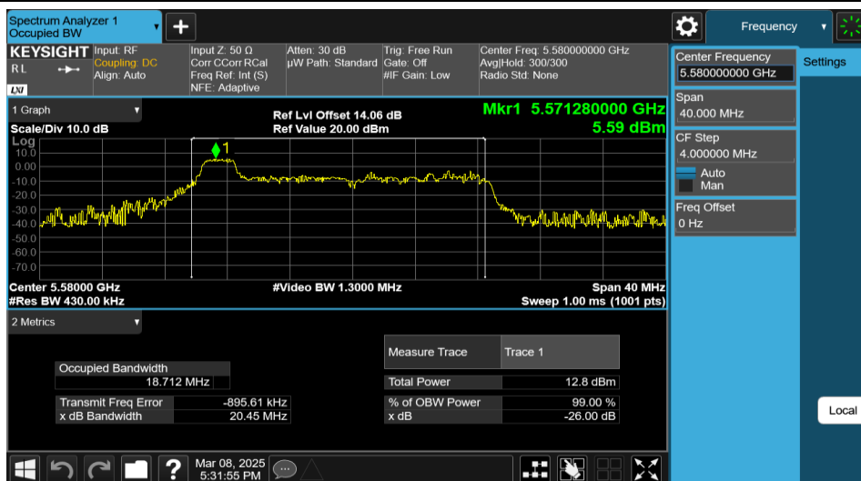
11AX20MIMO-Ant2-5580-26Tone-RU0
