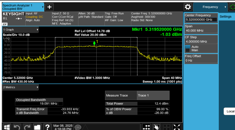
11AX20MIMO-Ant1-5320-242Tone-RU61
