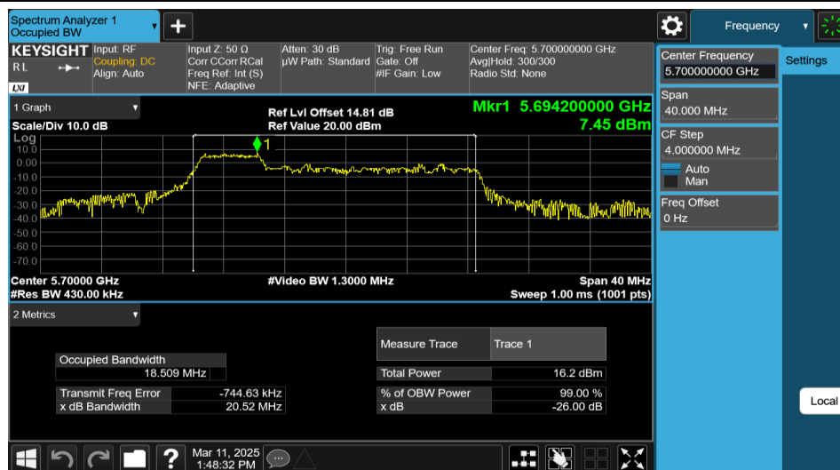
11AX20MIMO-Ant1-5700-52Tone-RU37
