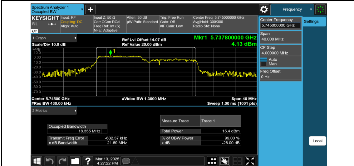
11AX20MIMO-Ant2-5745-106Tone-RU53
