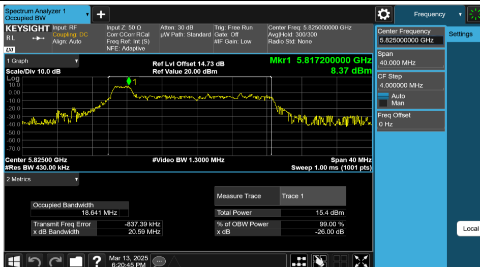
11AX20MIMO-Ant1-5825-26Tone-RU0
