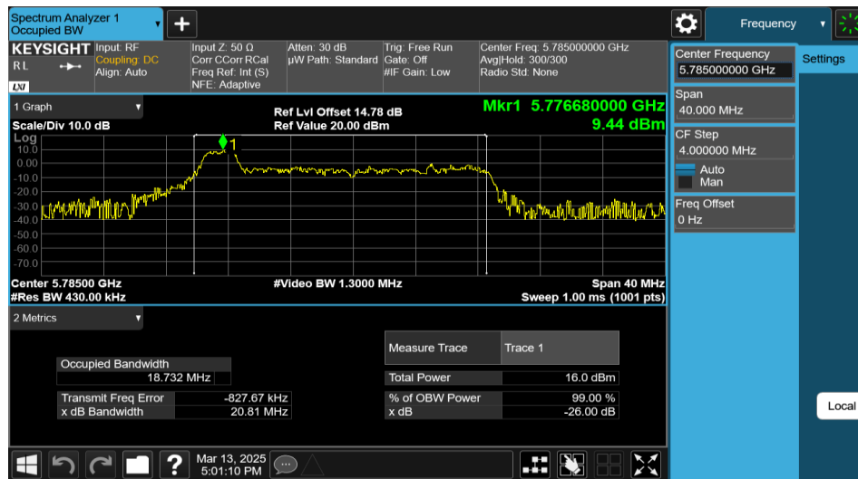
11AX20MIMO-Ant1-5785-26Tone-RU0
