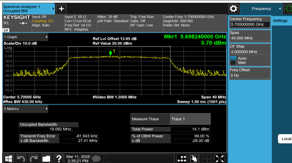
11AX20MIMO-Ant2-5700-242Tone-RU61
