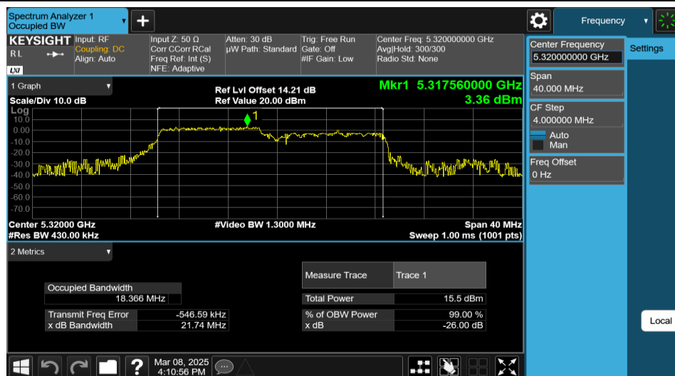
11AX20MIMO-Ant2-5320-106Tone-RU53
