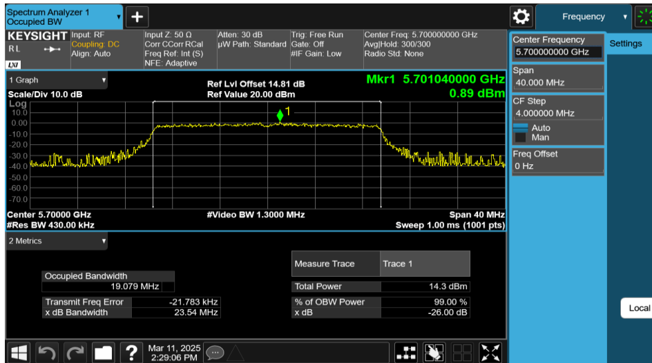
11AX20MIMO-Ant1-5700-242Tone-RU61
