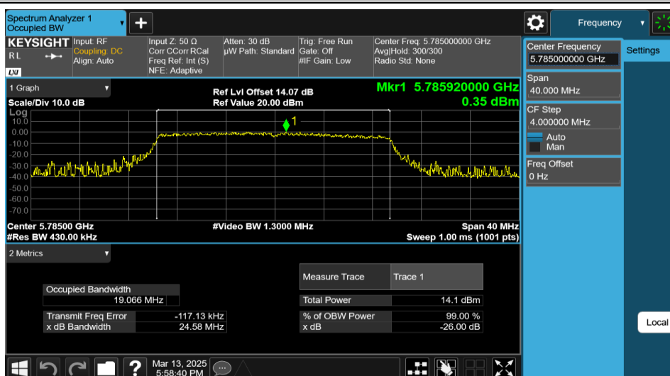
11AX20MIMO-Ant2-5785-242Tone-RU61
