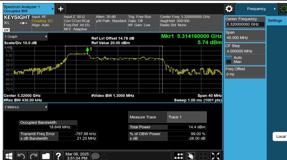
11AX20MIMO-Ant1-5320-52Tone-RU37
