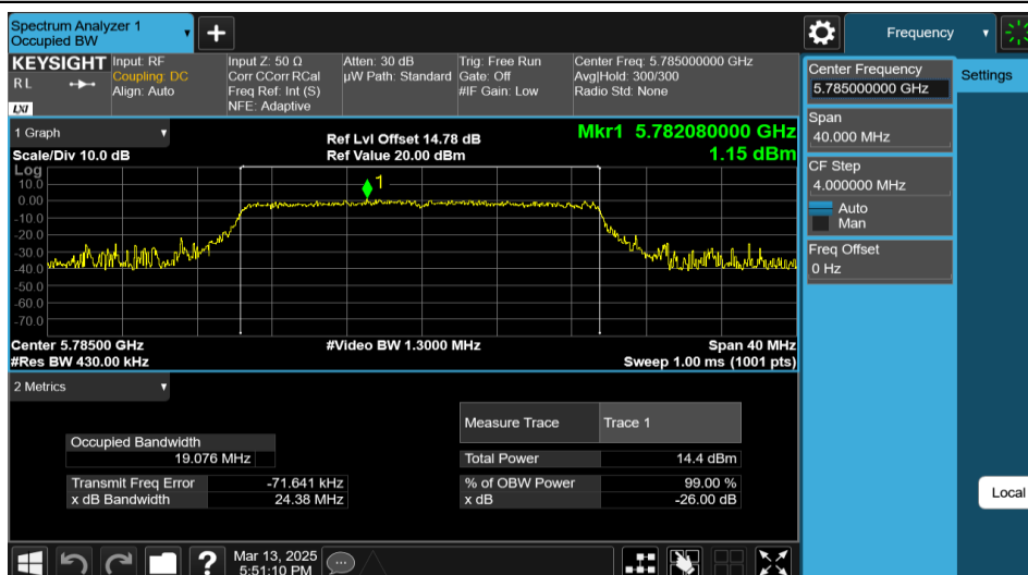
11AX20MIMO-Ant1-5785-242Tone-RU61
