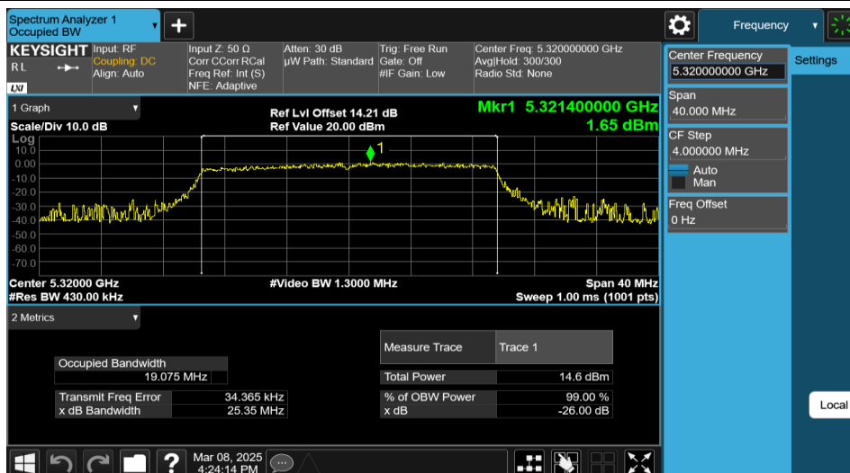
11AX20MIMO-Ant2-5320-242Tone-RU61
