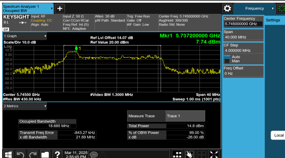
11AX20MIMO-Ant2-5745-26Tone-RU0
